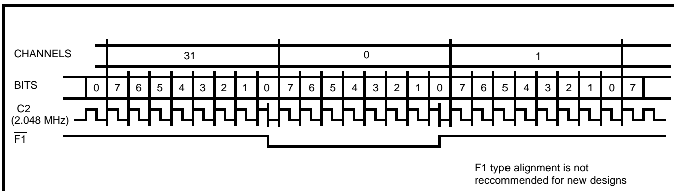
Figure 2 - Example of F1 Alignment for ST-BUS at 2.048 Mb/s
