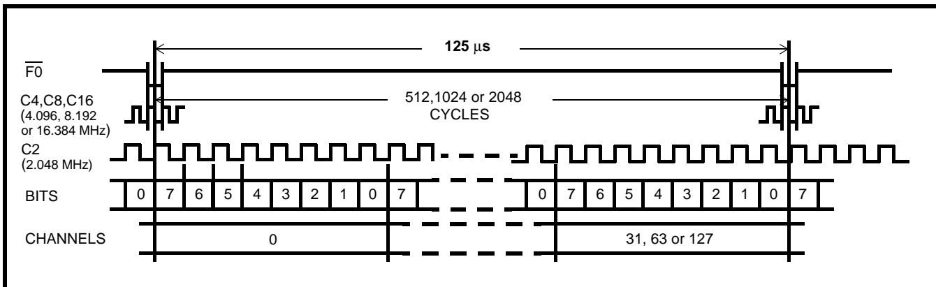
Figure 1 - F0 and Clock Alignment for ST-BUS at 2.048 Mb/s, 4.096 and 8.192 Mb/s
