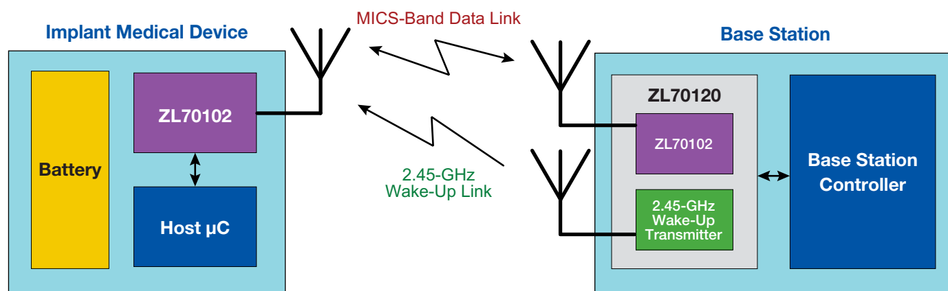
Figure 1-1 • Application Example
