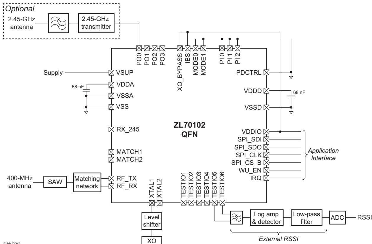
Figure 10-3 • External Device
