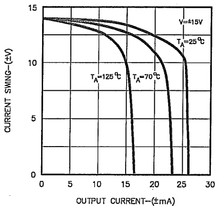
FIGURE 6. CURRENT LIMITING
