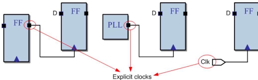
Figure 13 · Explicit Clocks
