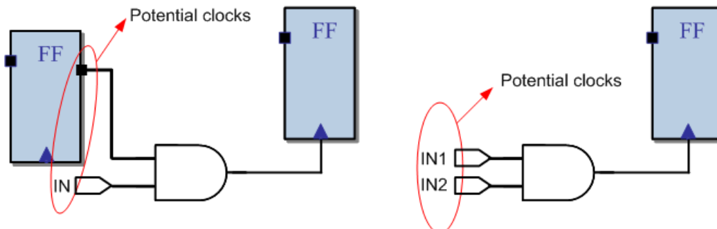
Figure 14 · Potential Clocks
