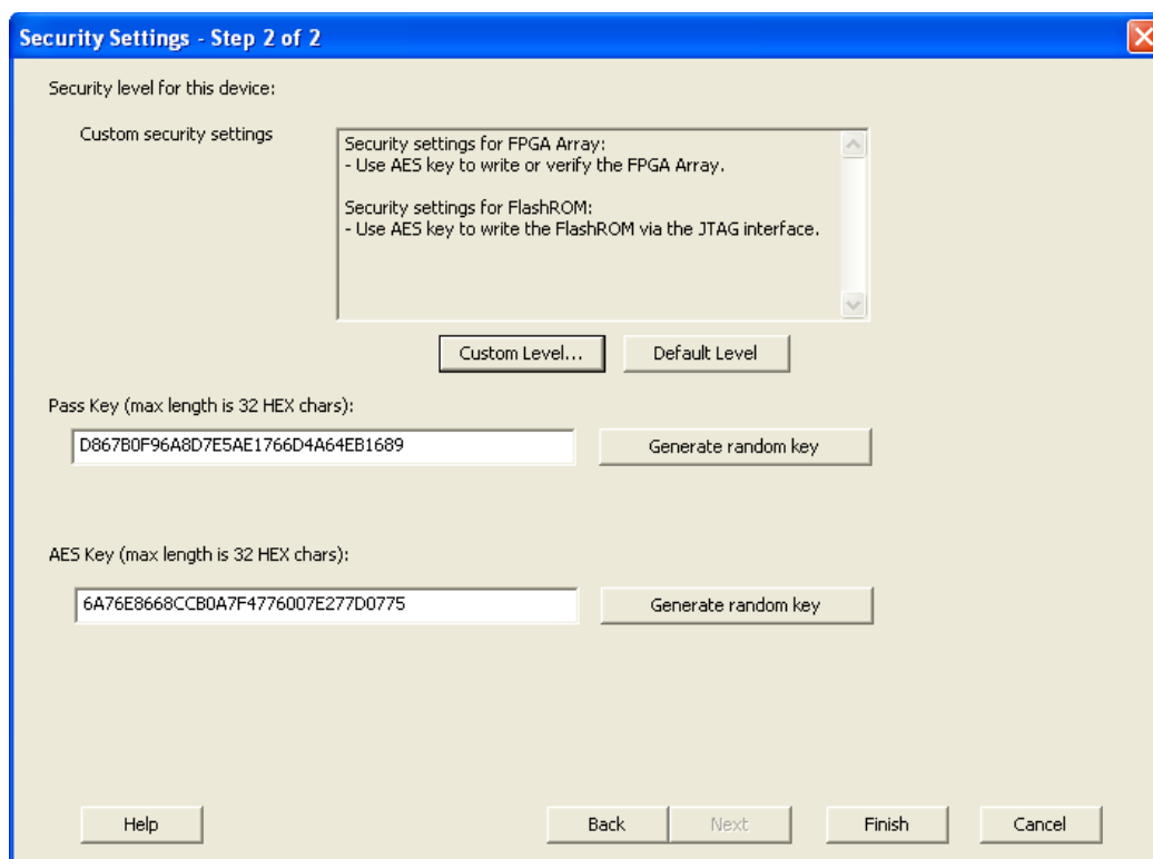
Figure 147 · Security Settings
