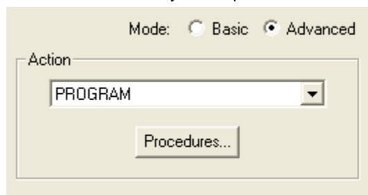
Figure 182 · Advanced Mode
