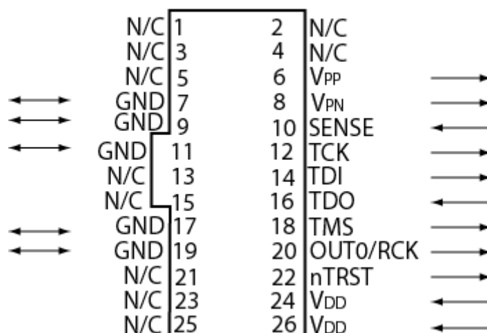
Figure 163 · 26-pin Connector for FlashPro Lite
