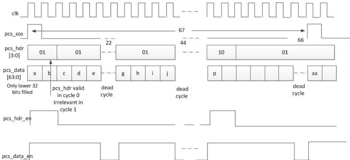
Figure 23 • 64b67b Receive Sequence For 32-Bit Interface
