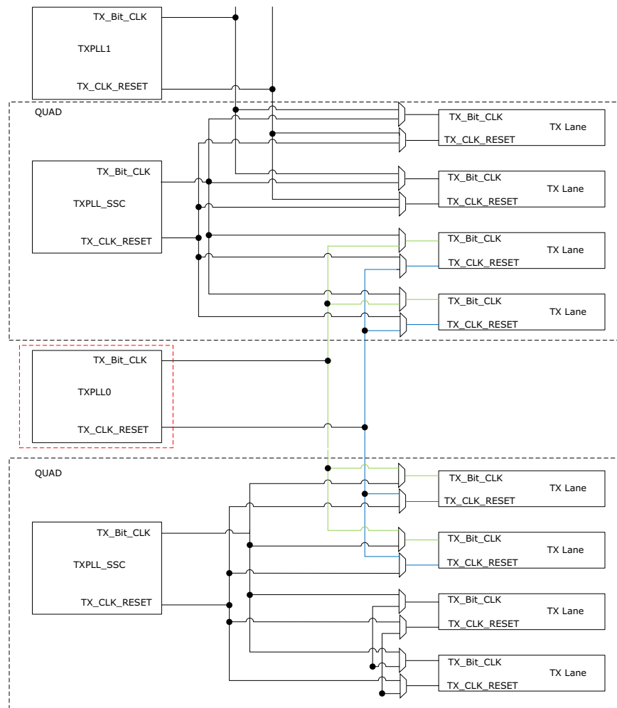
Figure 41 • Using TXPLLs For Upto Four Lanes
