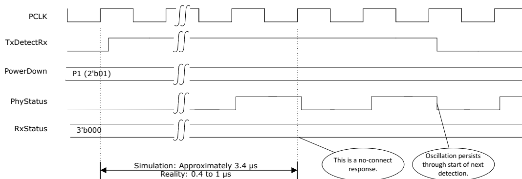
Figure 24 • Initial Receiver Detection Response For Receiver-Not-Present
