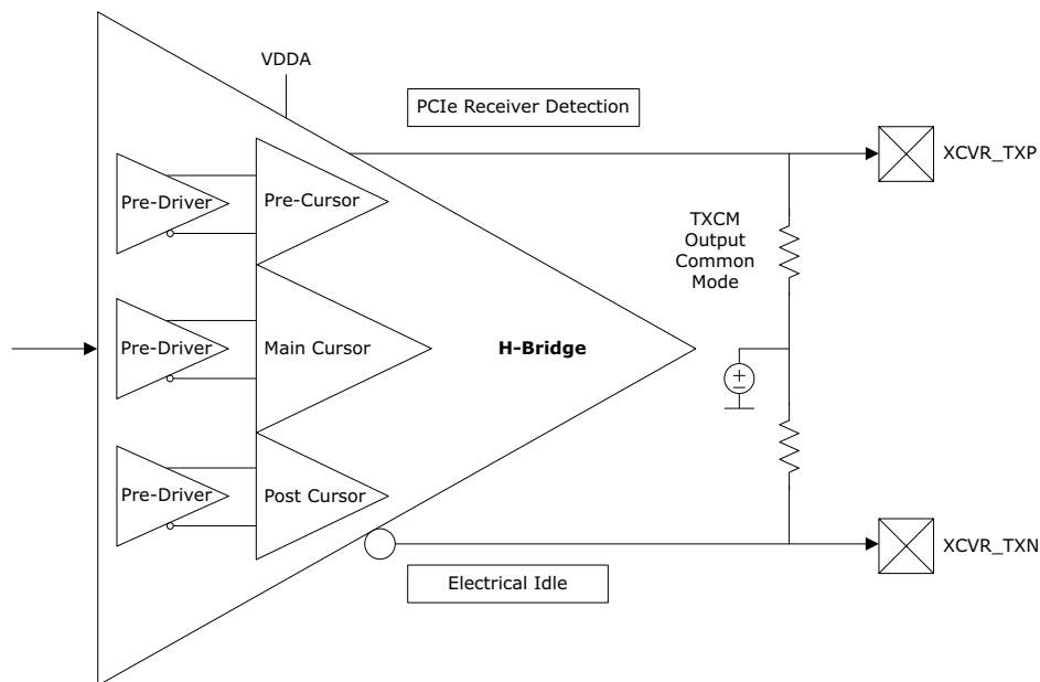
Figure 7 • Transmit Output Driver
