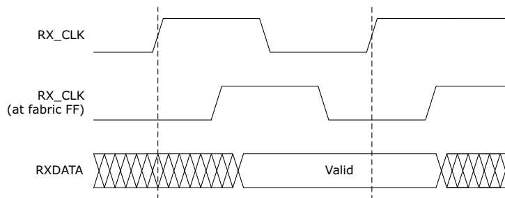
Figure 36 • Deterministic Transceiver Receive Timing Waveform
