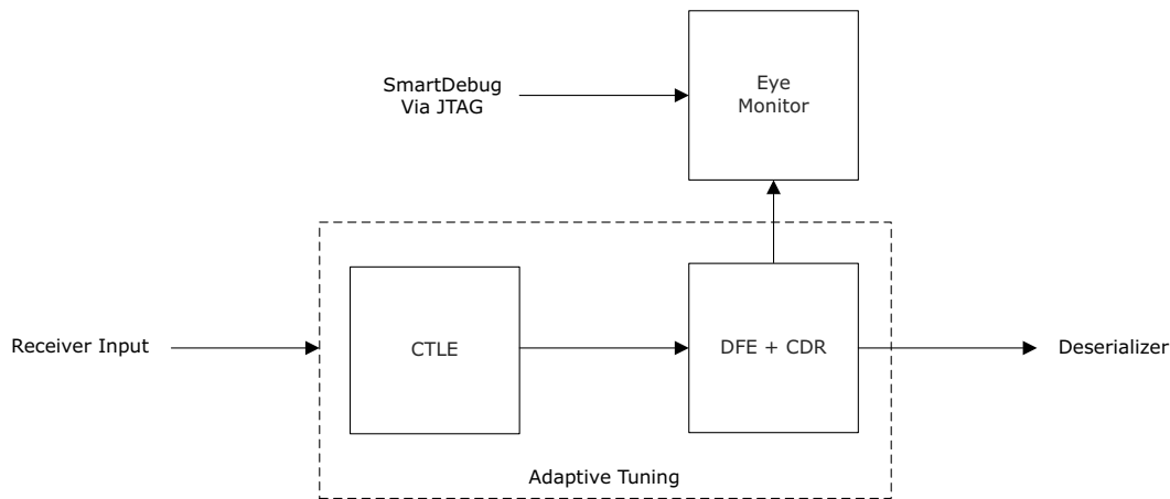
Figure 4 • Input Signal Path
