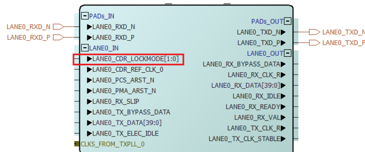
Figure 73 • XCVR Component With BMR Port Enabled
