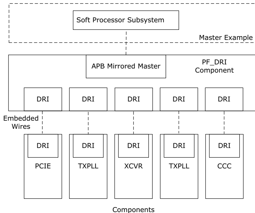
Figure 98 • PF_DRI Example
