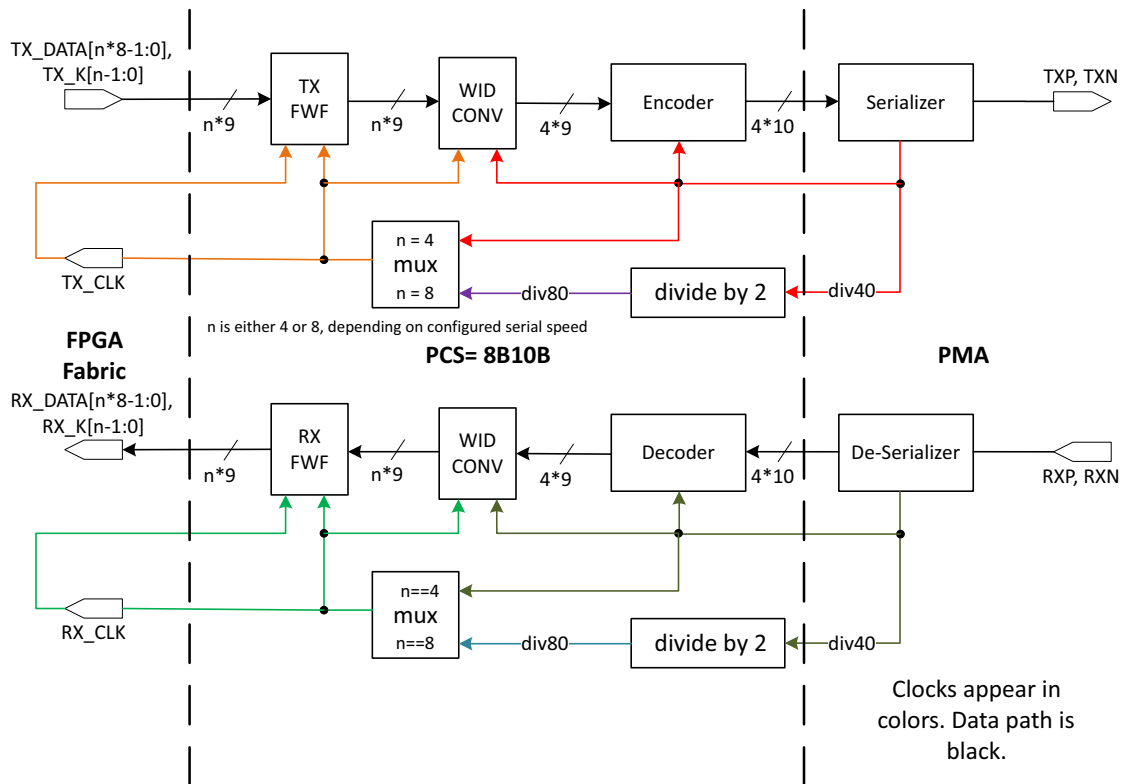
Figure 16 • 8b10b Data Path
