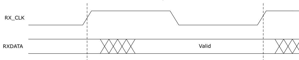
Figure 33 • Non-Deterministic Transceiver Receive Timing Waveform
