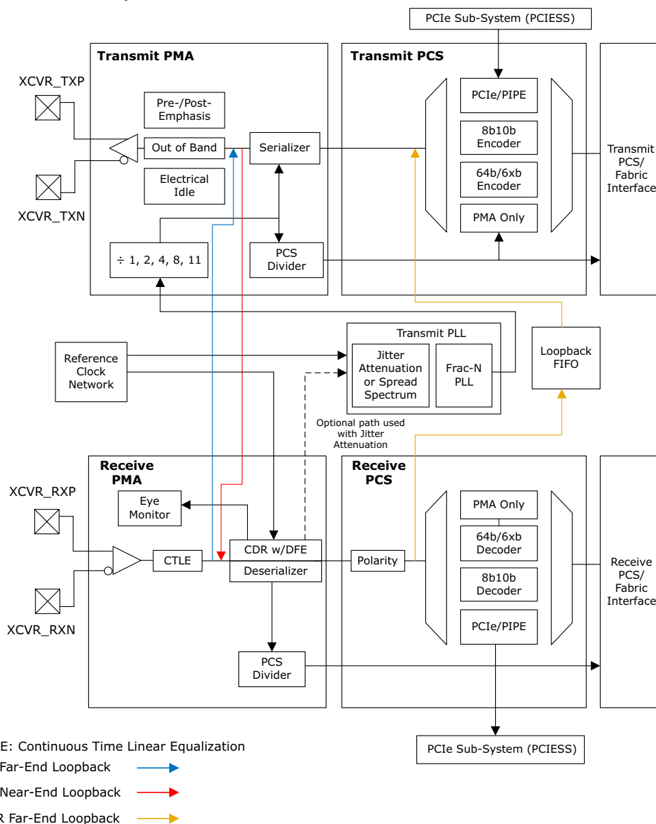
Figure 97 • Transceiver Loopbacks
