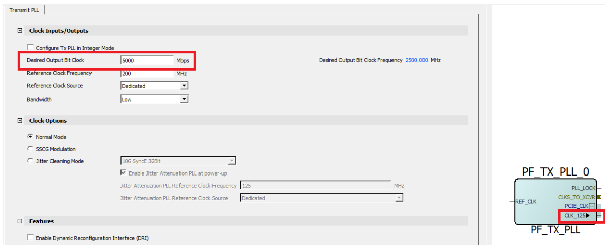
Figure 68 • CLK_125 GUI
