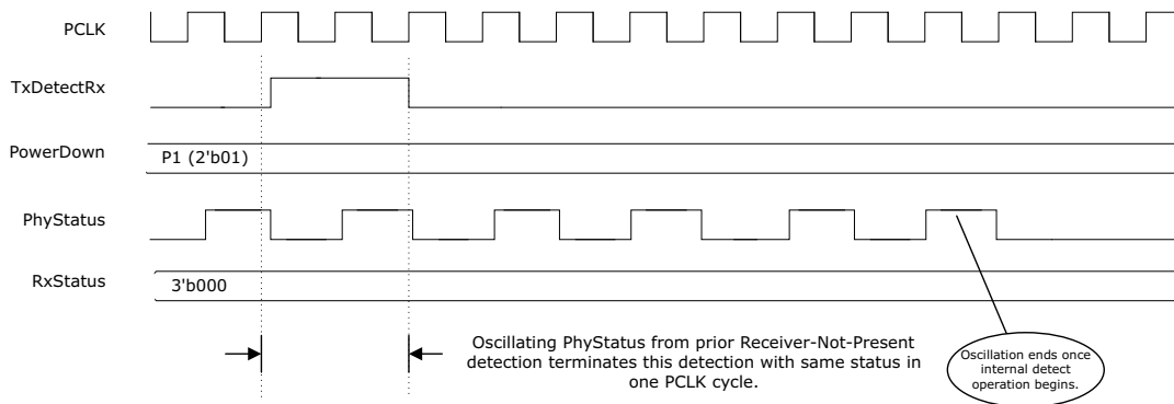
Figure 26 • Subsequent Receiver Detection Where Prior Status Was Receiver-Not-Present
