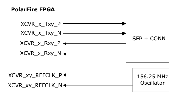
Figure 101 • Connectivity Between RT PolarFire Device to SFP+ Interface
