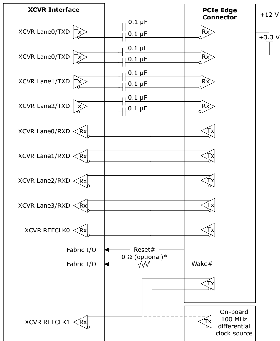
Figure 99 • Connectivity Between XCVR Interface and PCIe Edge Connector
