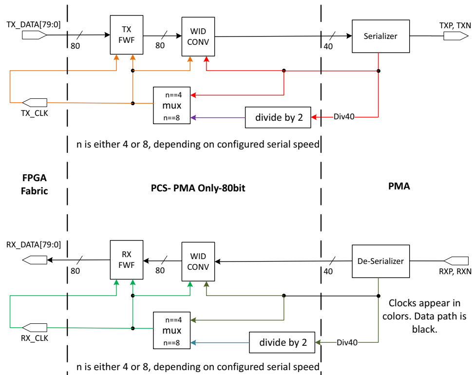
Figure 28 • PMA Only Data Path – 80-bits
