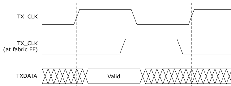
Figure 35 • Deterministic Transceiver Transmit Timing Waveform
