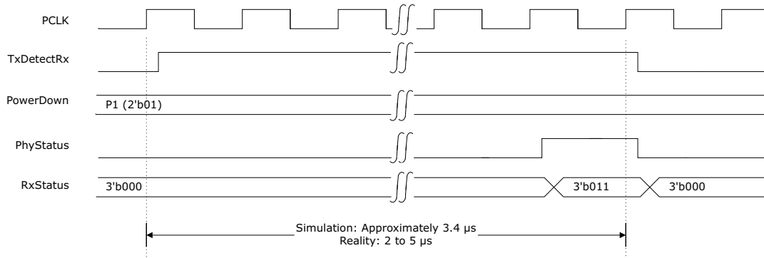
Figure 25 • Initial Receiver Detection For Receiver-Present
