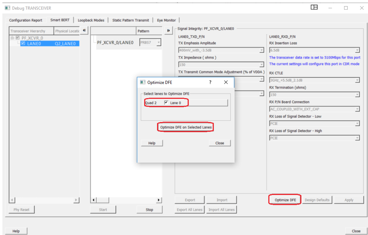
Figure 95 • Example of Optimize DFE
