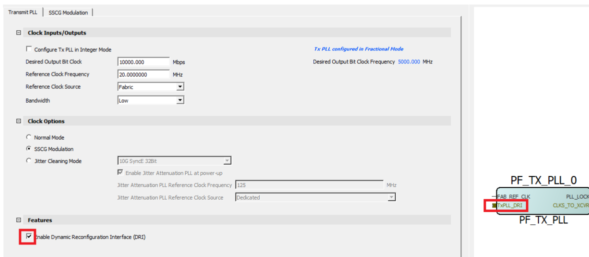
Figure 67 • Enable Dynamic reconfiguration Interface
