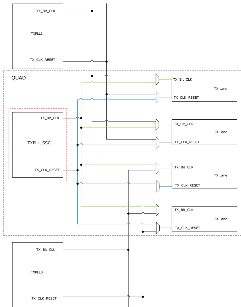
Figure 40 • Using TXPLL_SSC For Upto Four Lanes
