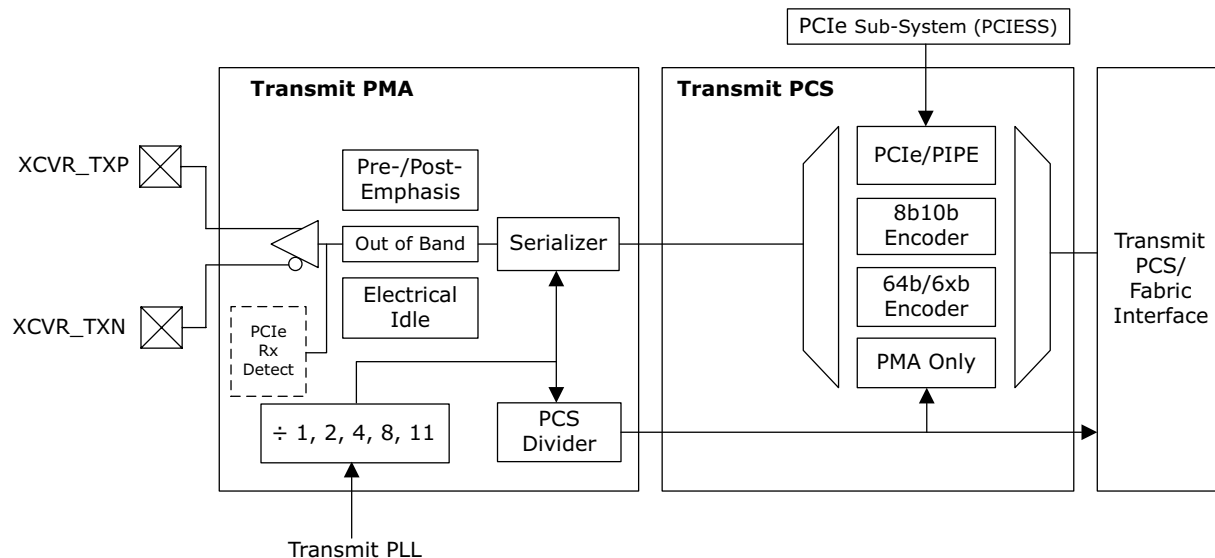
Figure 6 • Transceiver Transmitter
