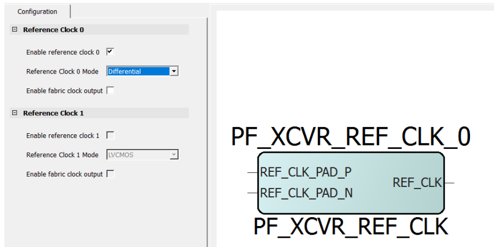
Figure 58 • PF_XCVR_REF_CLK With Differential Input and Single Output Clock
