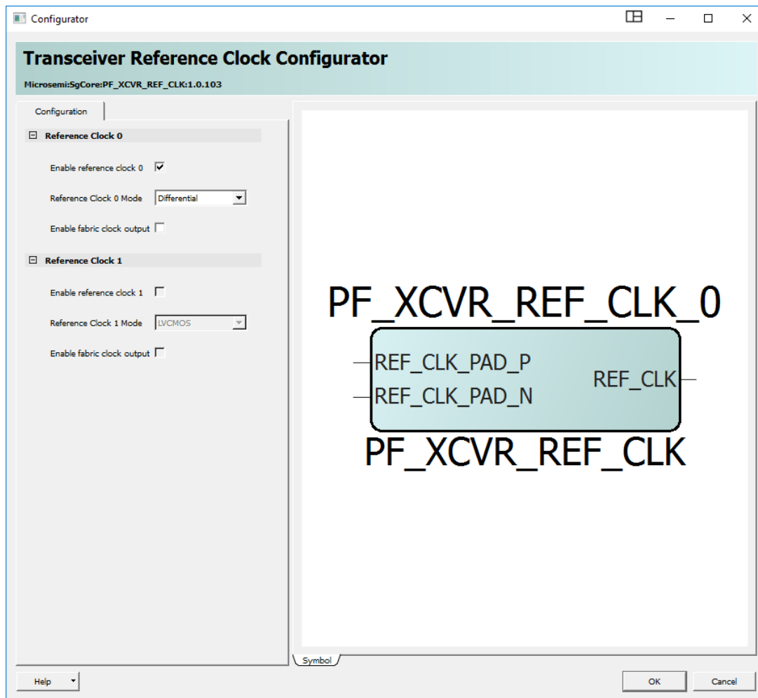
Figure 54 • Transceiver Reference Clock Configurator GUI
