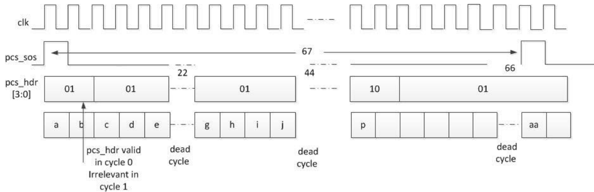
Figure 22 • 64b67b Transmit Sequence For 32-Bit Interface
