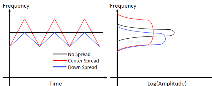
Figure 39 • Spread Spectrum Clocking Modulation Mode
