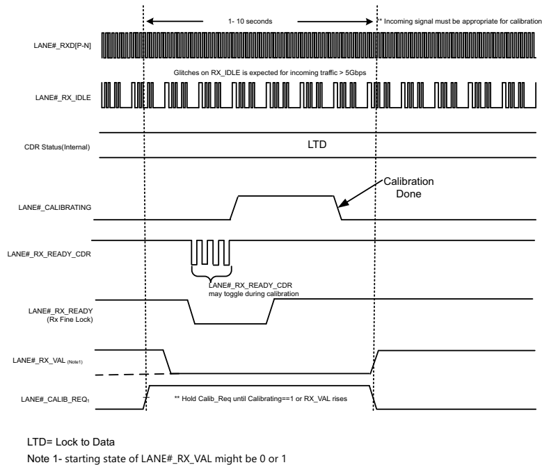
Figure 15 • On-Demand Calibration Waveform
