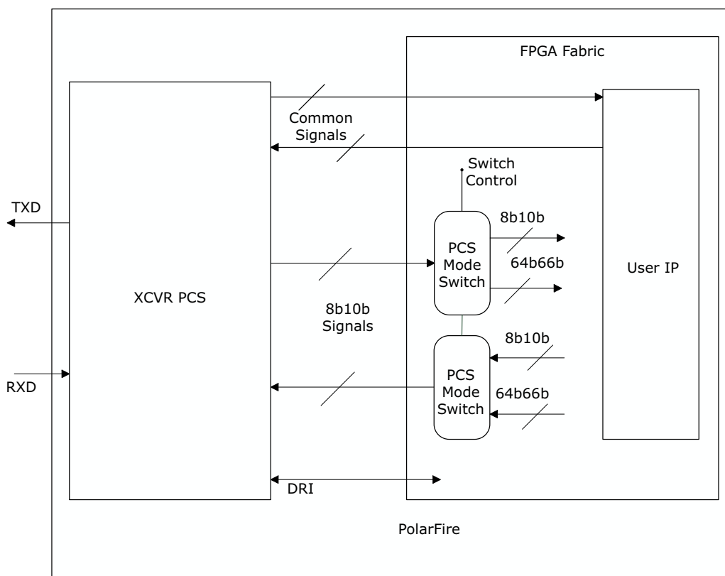
Figure 52 • PCS Rate Switch between 8b10b and 64b66b Mode
