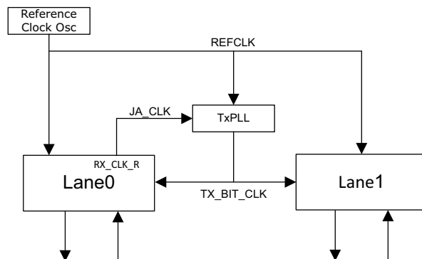
Figure 44 • Typical Jitter Attenuator Application Scheme
