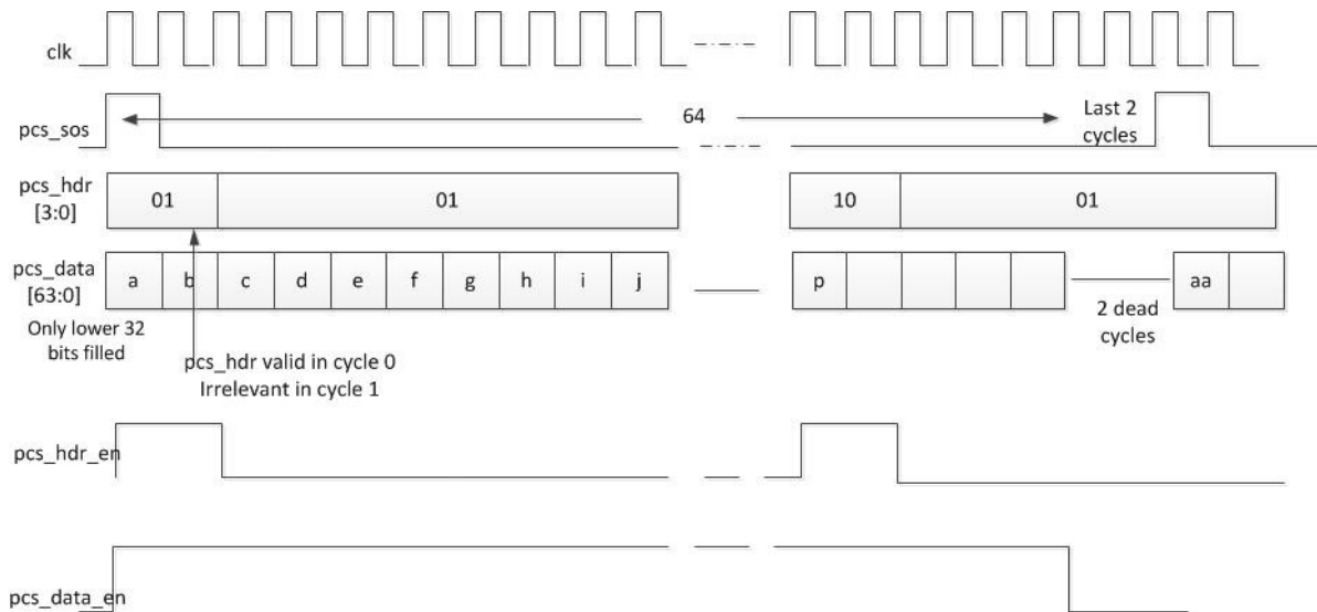
Figure 19 • 64b66b Receive Sequence For 64-Bit Interface
