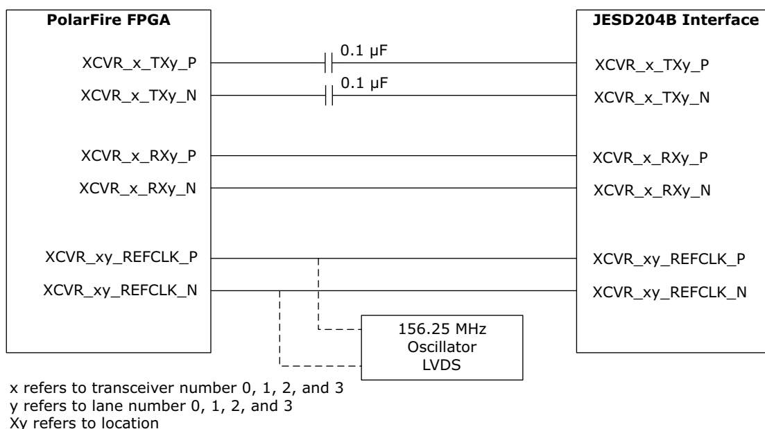
Figure 100 • Connectivity Between RT PolarFire Device and JESD204B Interface
