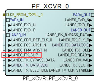
Figure 72 • XCVR Component With CDR Bit-Slip Port Enabled
