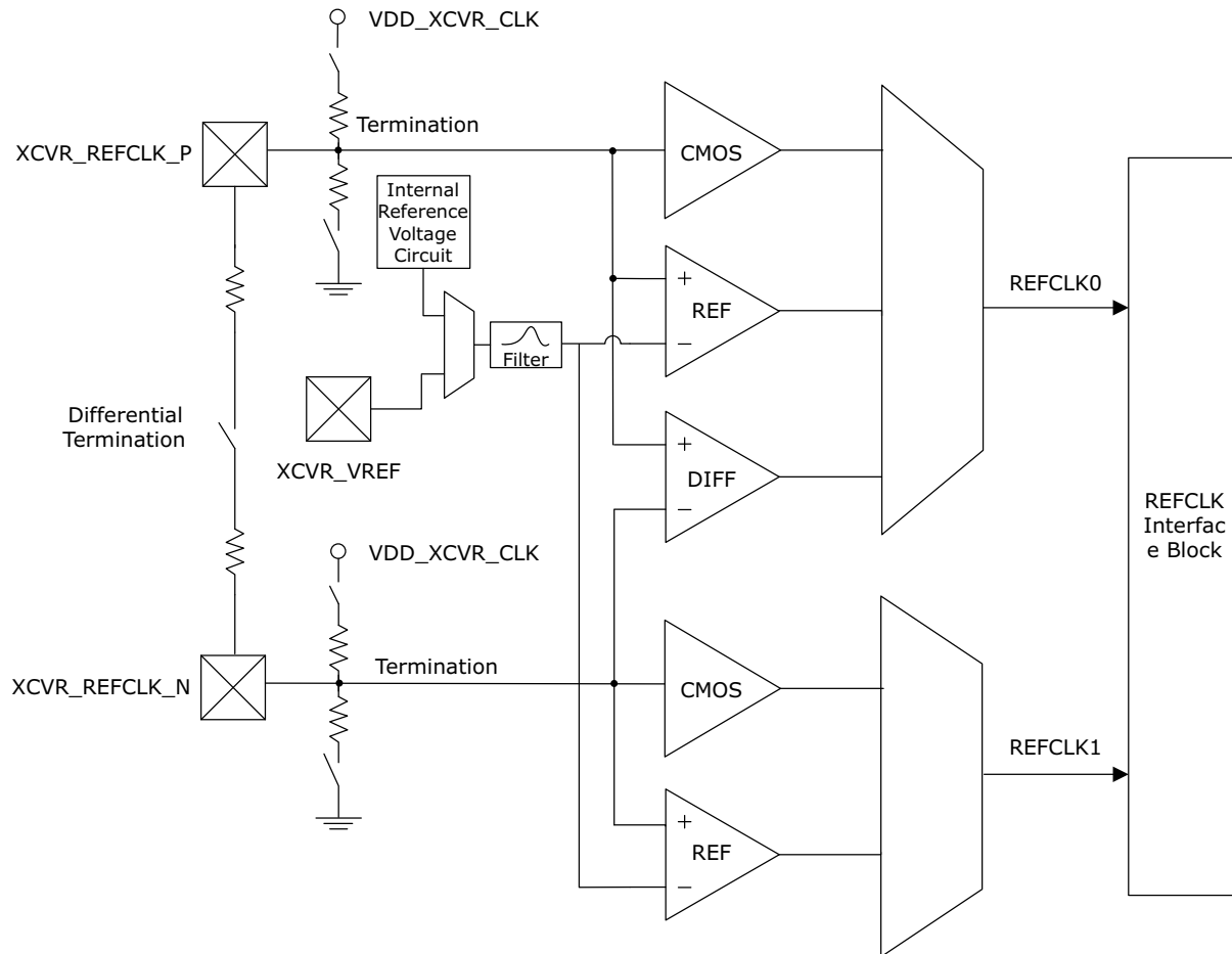
Figure 49 • Dedicated Transceiver Reference Clock Inputs
