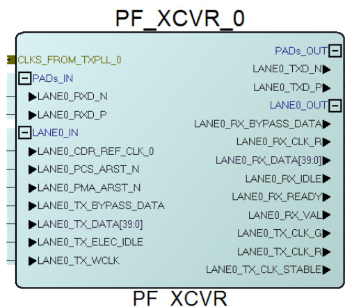
Figure 77 • 8b10b PCS Example SmartDesign Component
