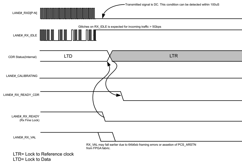
Figure 13 • Disruption of Serial Rx Data Stream
