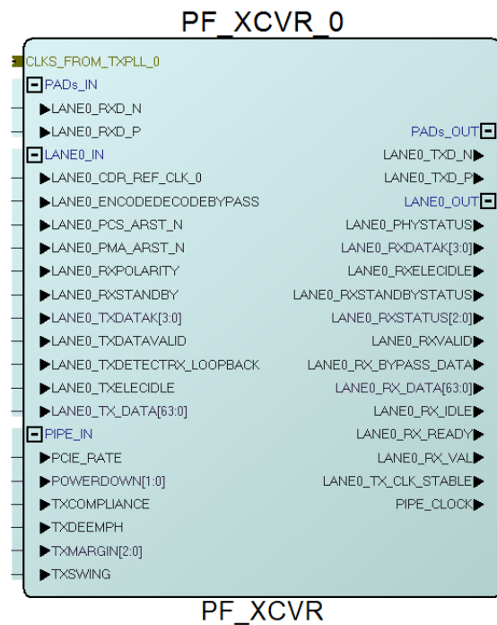
Figure 79 • Soft PIPE PCS Example SmartDesign Component
