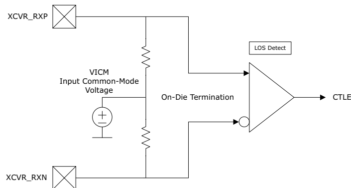
Figure 3 • Receiver Input Buffer
