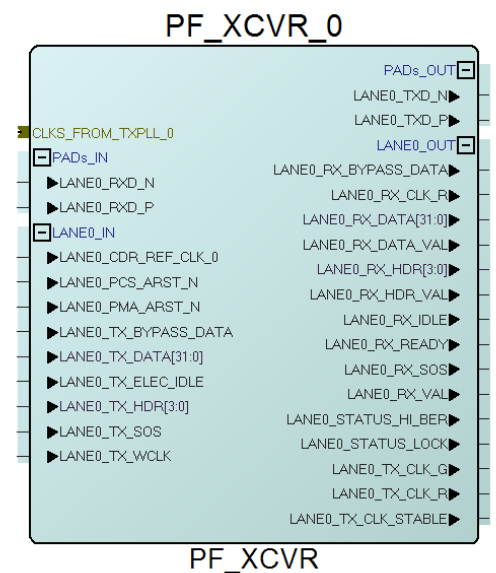
Figure 78 • 64b66b PCS Example SmartDesign Component
