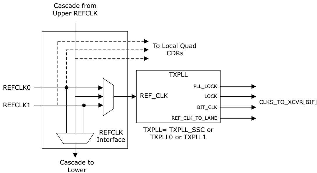
Figure 43 • Reference Clock (REFCLK) Interface to Transmit PLL
