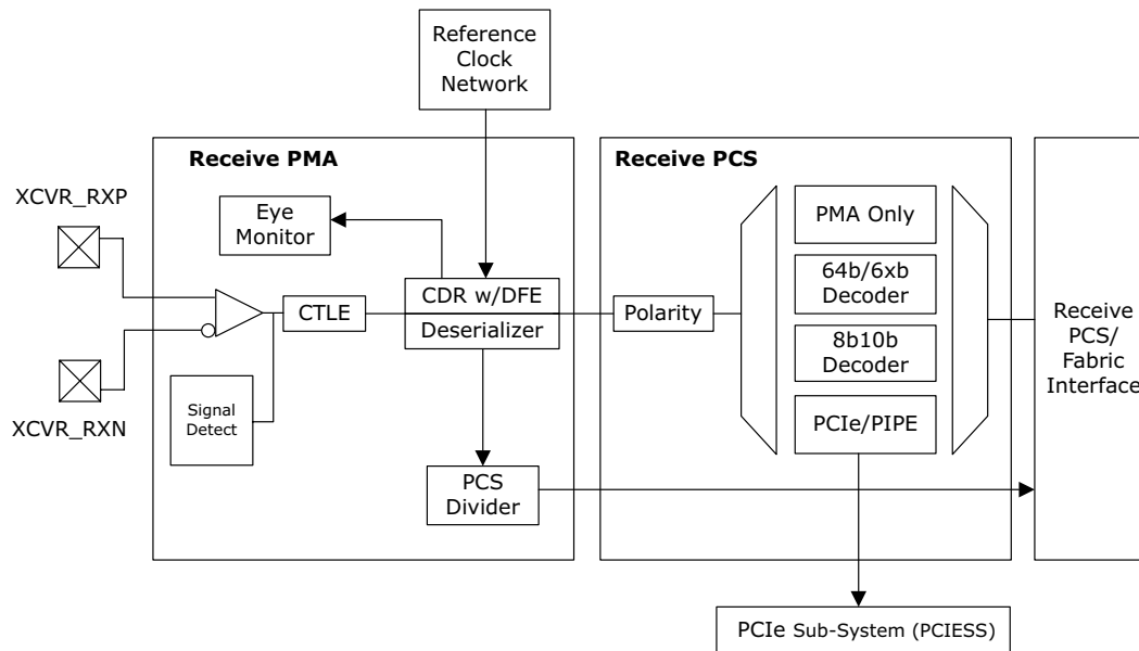
Figure 2 • Transceiver Receiver
