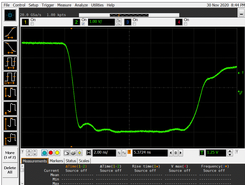
Figure 17b DUT 7372 Post-Annealing Falling Edge
