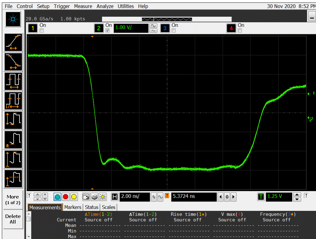
Figure 14b DUT 7419 Post-Annealing Falling Edge
