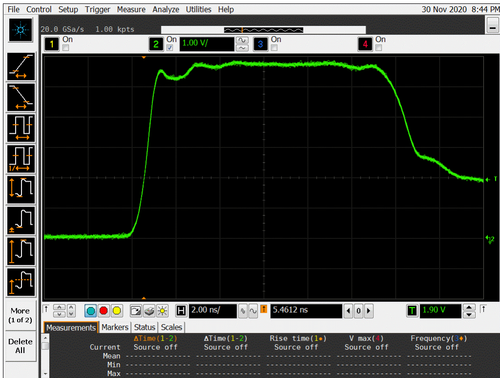
Figure 12b DUT 7372 Post-Annealing Rising Edge
