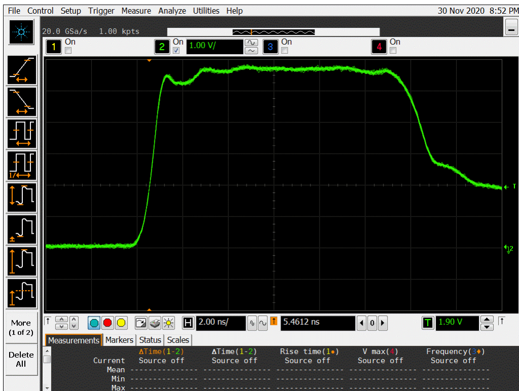
Figure 9b DUT 7419 Post-Annealing Rising Edge
