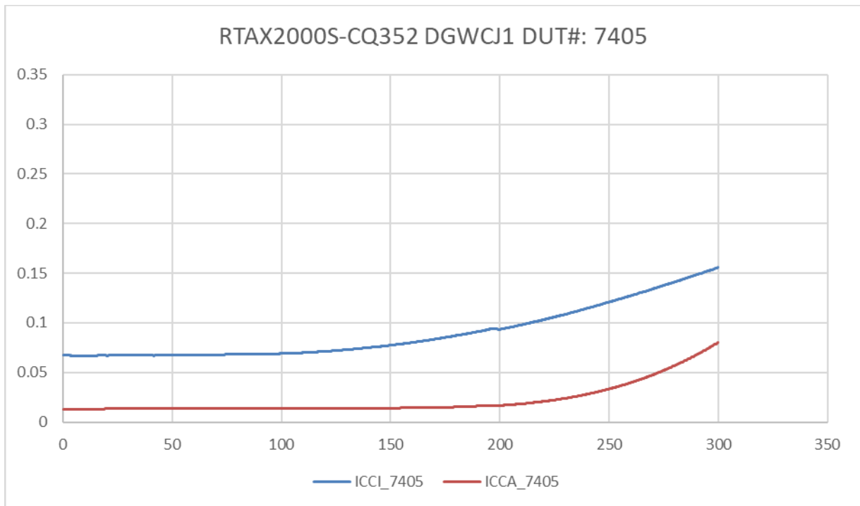
Figure 2 DUT 7405 Influx ICCA and ICCI
