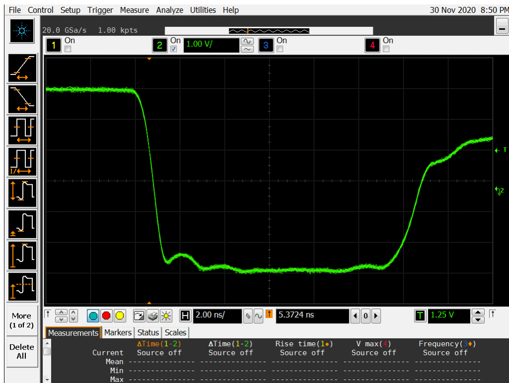
Figure 13b DUT 7405 Post-Annealing Falling Edge
