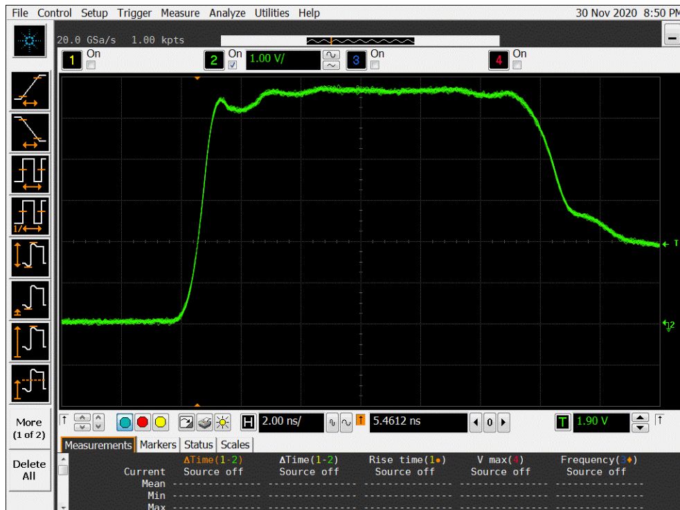
Figure 8b DUT 7405 Post-Annealing Rising Edge
