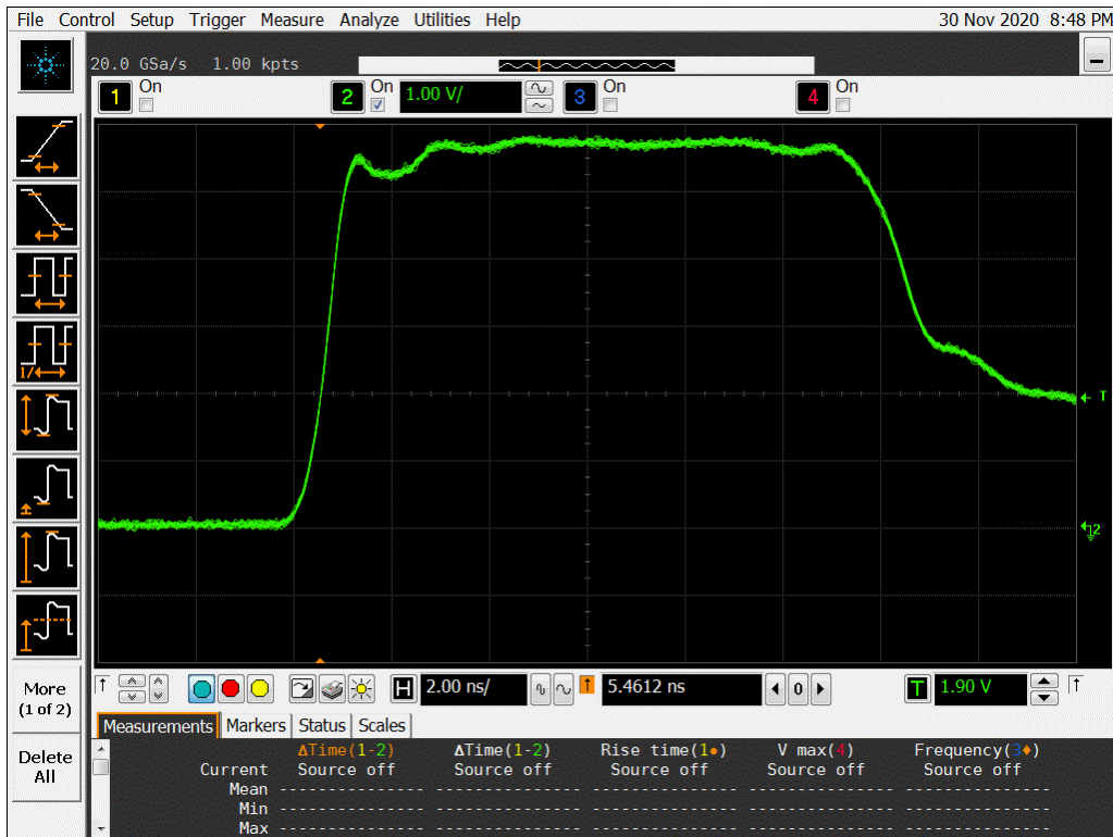
Figure 11b DUT 7402 Post-Annealing Rising Edge
