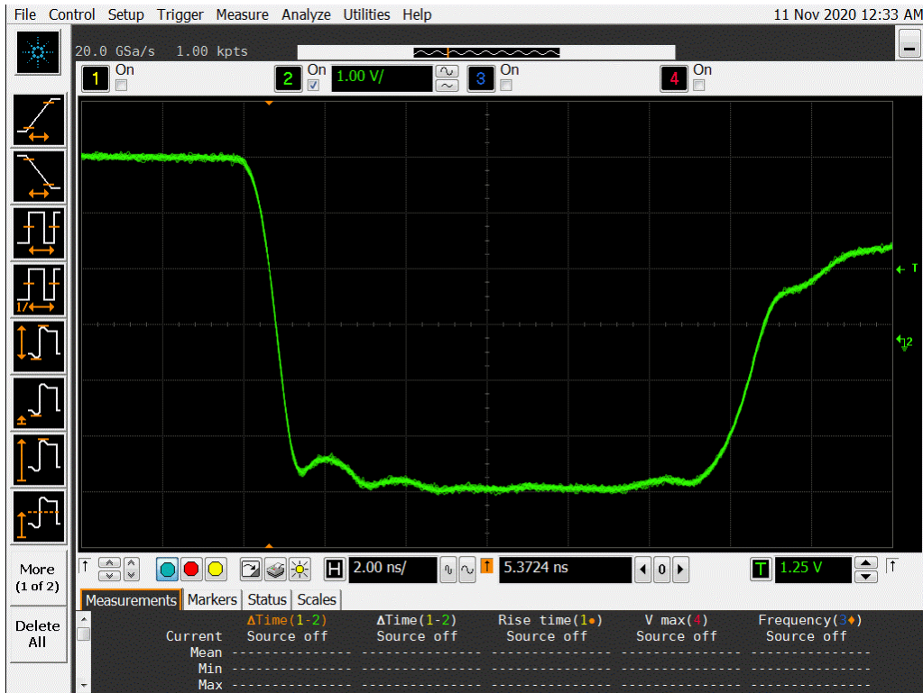
Figure 17a DUT 7372 Pre-Irradiation Falling Edge
