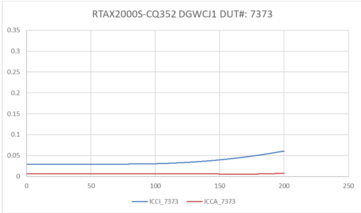
Figure 4 DUT 7373 Influx ICCA and ICCI
