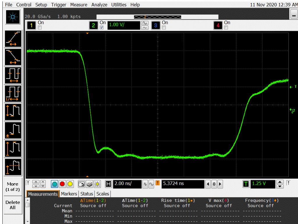
Figure 13a DUT 7405 Pre-Radiation Falling Edge
