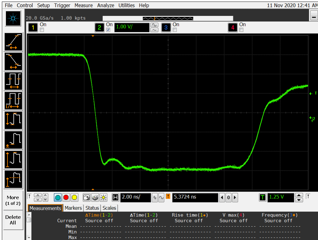
Figure 14a DUT 7419 Pre-Irradiation Falling Edge
