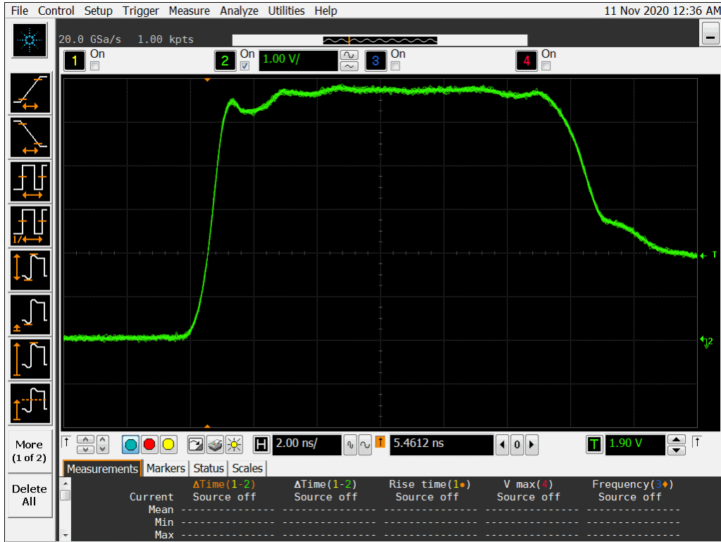
Figure 11a DUT 7402 Pre-Irradiation Rising Edge
