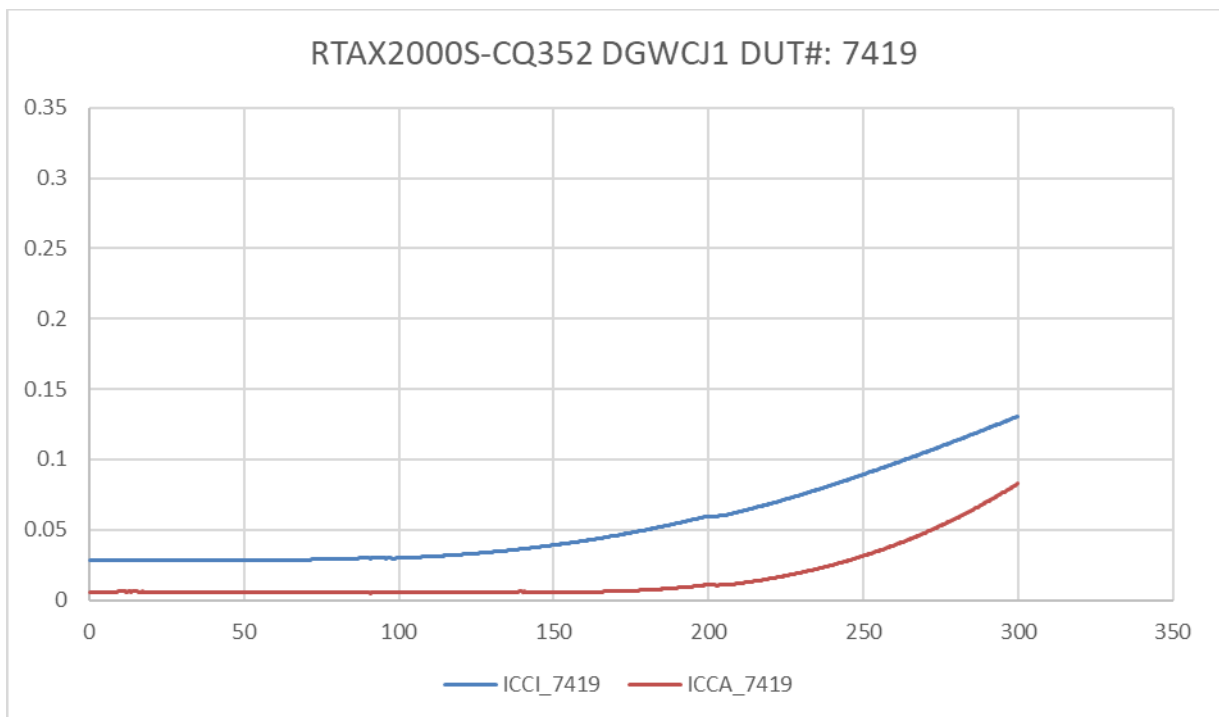
Figure 3 DUT 7419 Influx ICCA and ICCI
