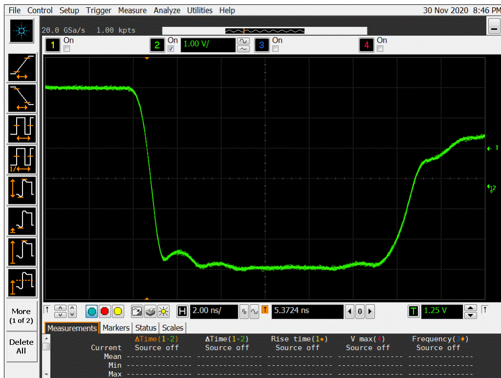
Figure 15b DUT 7373 Post-Annealing Falling Edge
