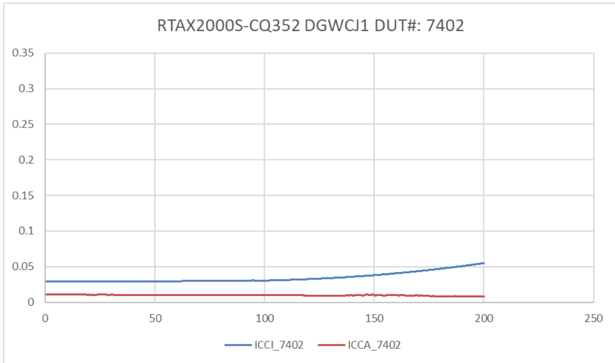
Figure 5 DUT 7402 Influx ICCA and ICCI
