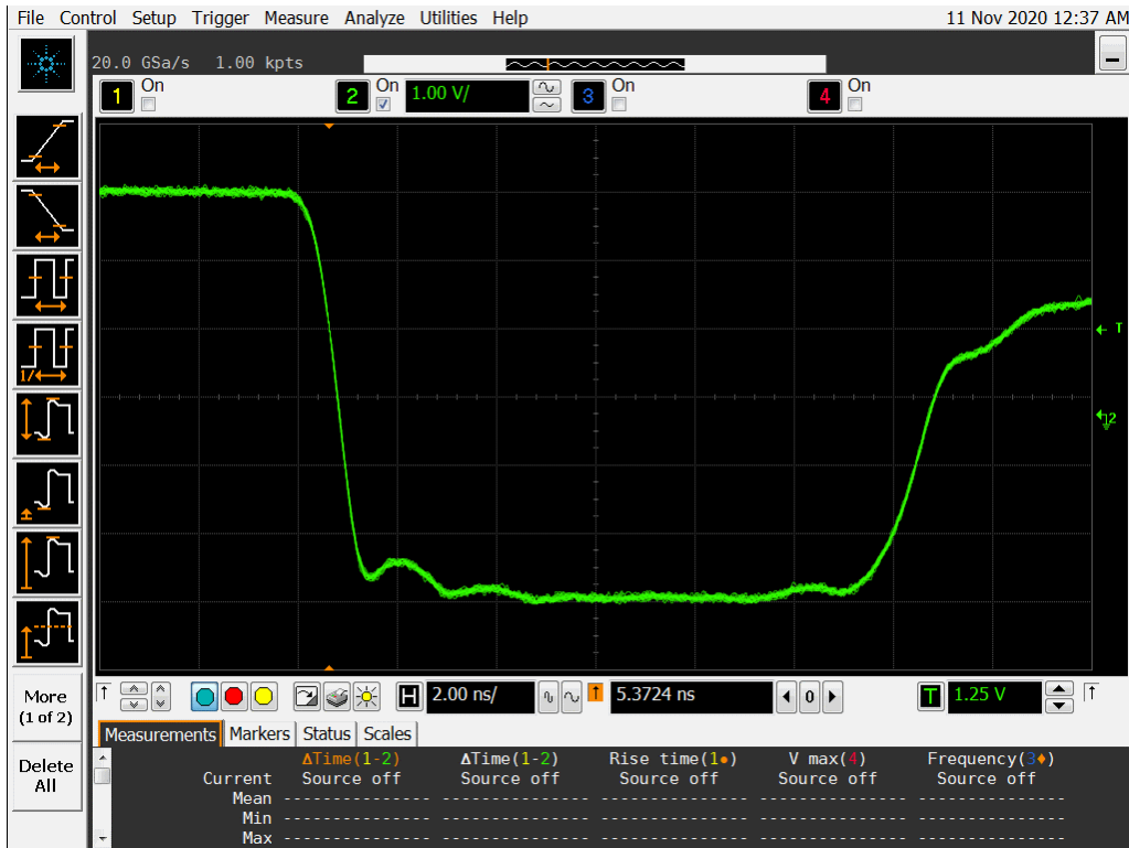
Figure 16a DUT 7402 Pre-Irradiation Falling Edge
