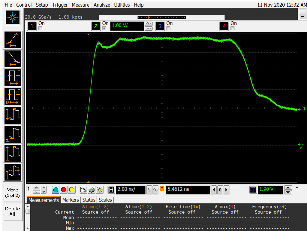
Figure 12a DUT 7372 Pre-Irradiation Rising Edge
