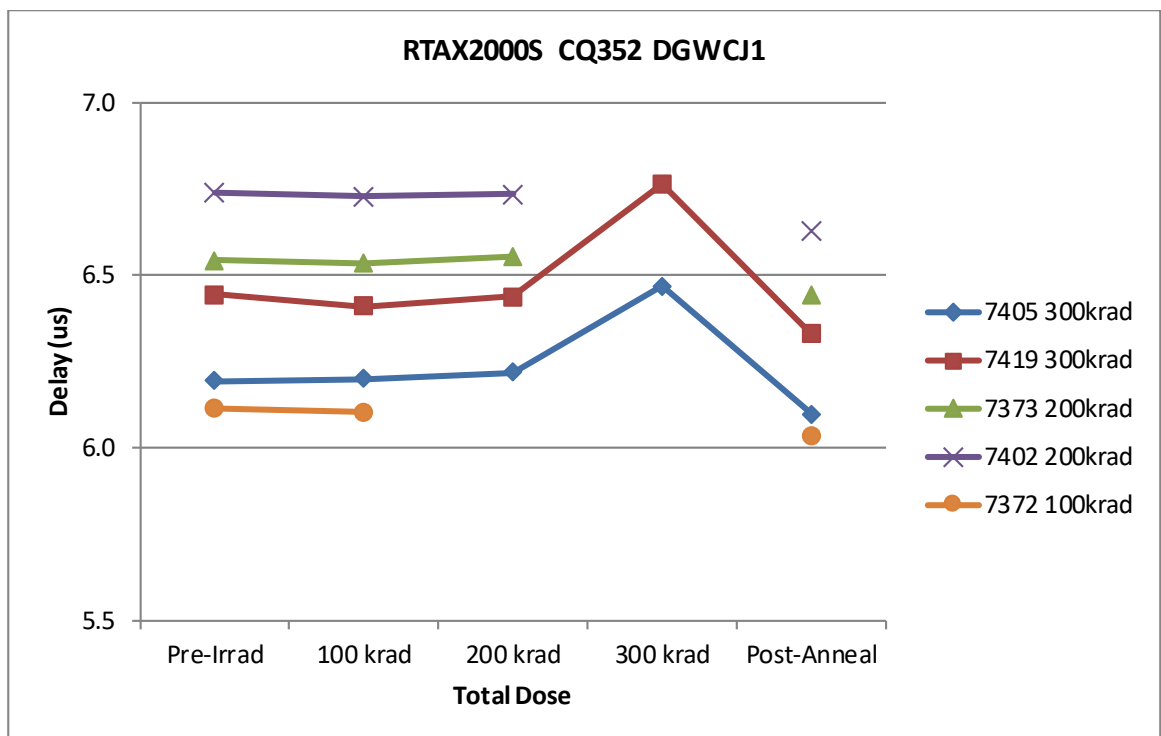
Figure 7 In-Situ Propagation Delay versus Total Dose
