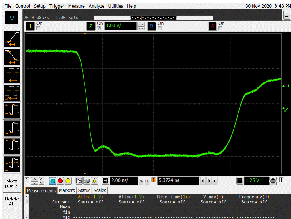
Figure 16b DUT 7402 Post-Annealing Falling Edge
