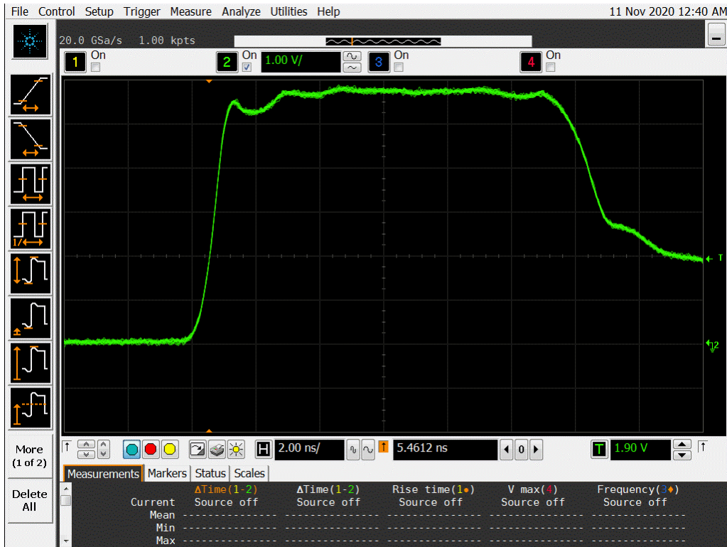
Figure 9a DUT 7419 Pre-Irradiation Rising Edge
