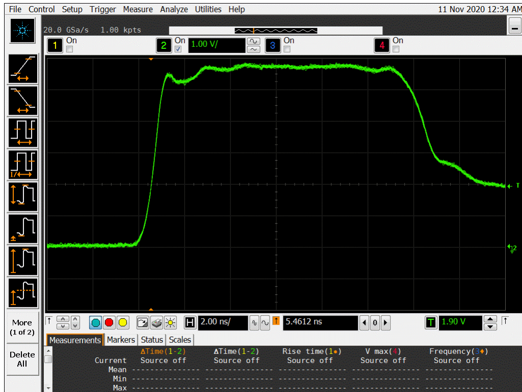
Figure 10a DUT 7373 Pre-Radiation Rising Edge
