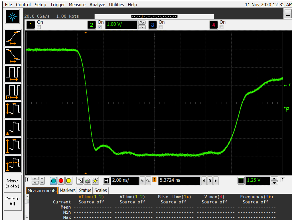
Figure 15a DUT 7373 Pre-Irradiation Falling Edge
