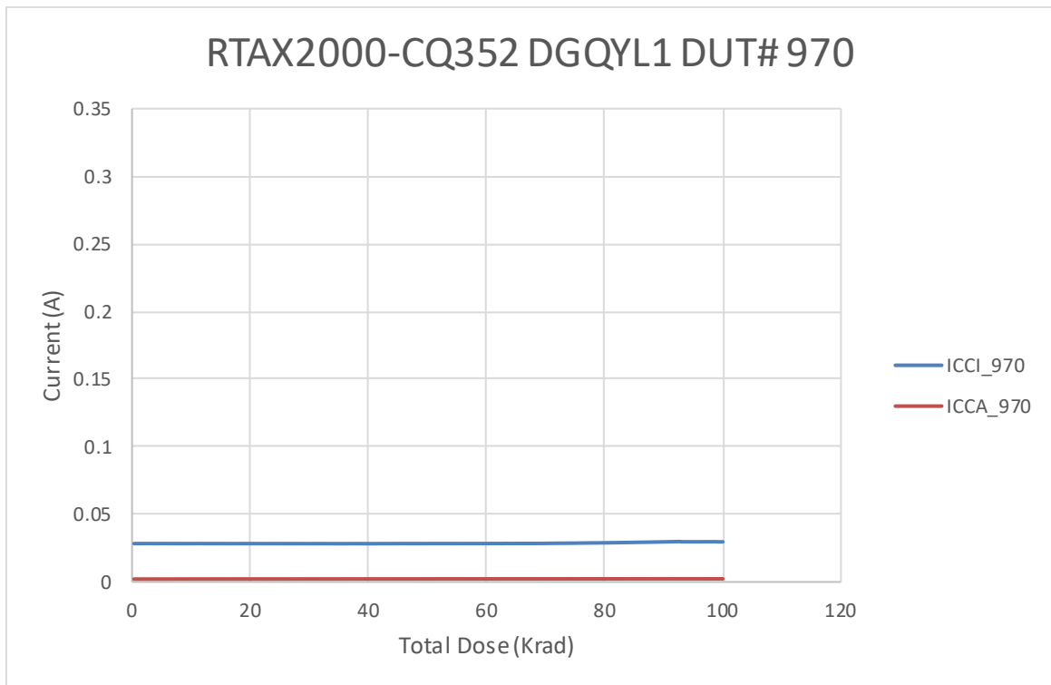
Figure 3 DUT 970 Influx ICCA and ICCI
