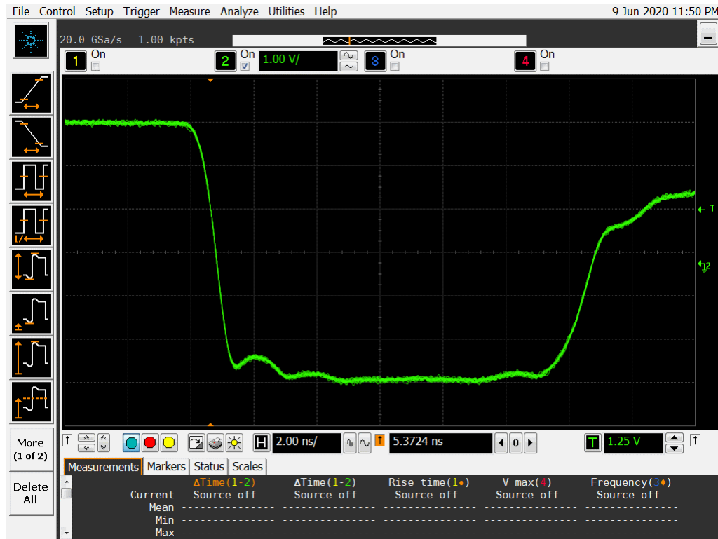
Figure 15a DUT 1014 Pre-Radiation Falling Edge
