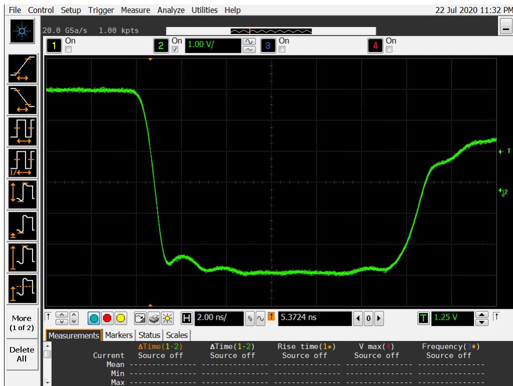
Figure 15b DUT 1014 Post-Annealing Falling Edge
