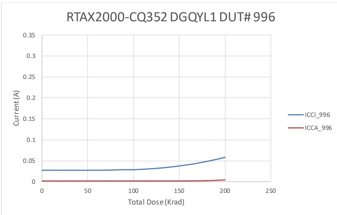
Figure 5 DUT 996 Influx ICCA and ICCI
