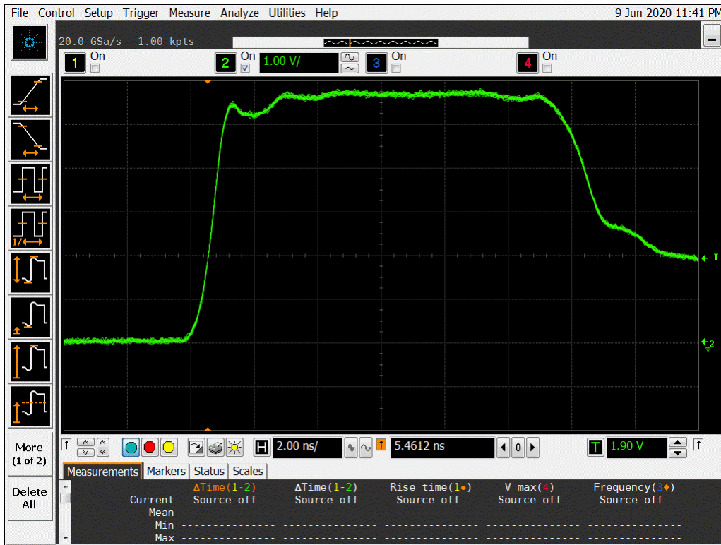
Figure 14a DUT 970 Pre-Irradiation Rising Edge
