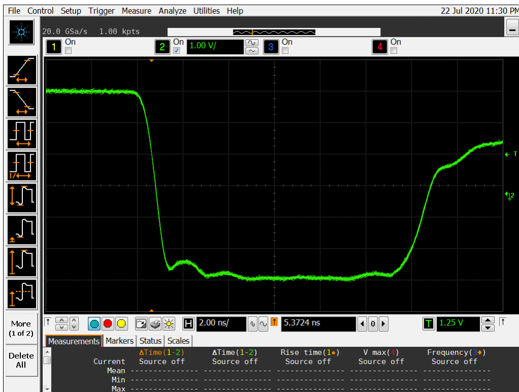
Figure 18b DUT 996 Post-Annealing Falling Edge
