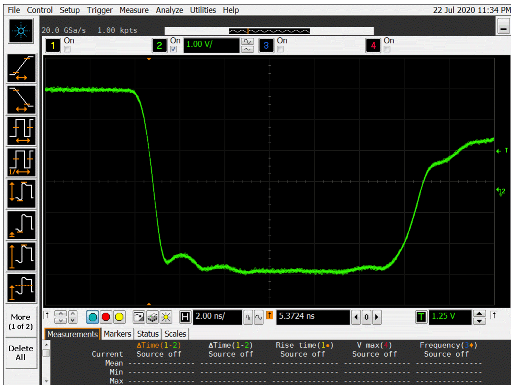
Figure 16b DUT 1018 Post-Annealing Falling Edge
