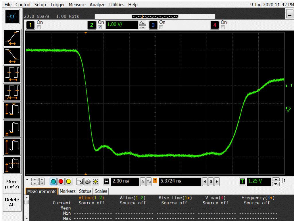
Figure 20a DUT 970 Pre-Irradiation Falling Edge
