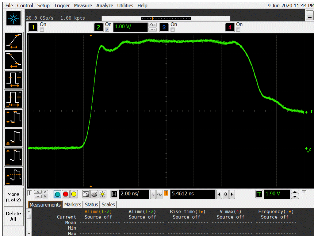
Figure 11a DUT 994 Pre-Radiation Rising Edge
