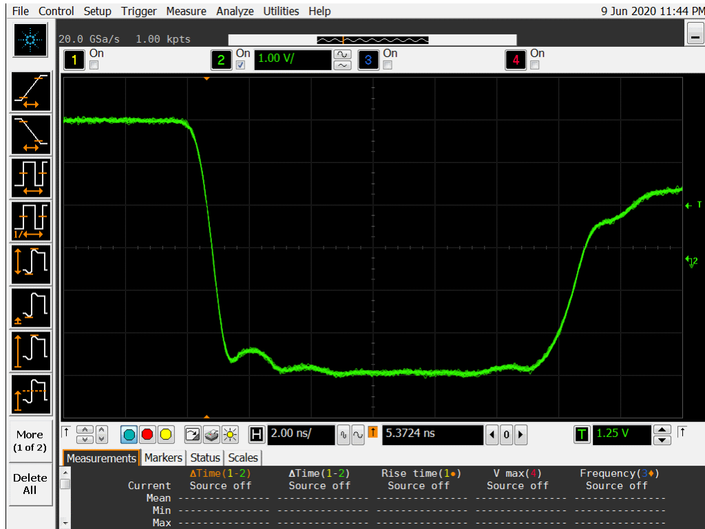
Figure 17a DUT 994 Pre-Irradiation Falling Edge
