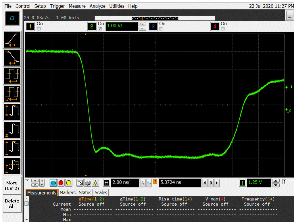
Figure 20b DUT 970 Post-Annealing Falling Edge
