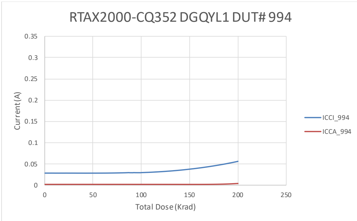
Figure 4 DUT 994 Influx ICCA and ICCI
