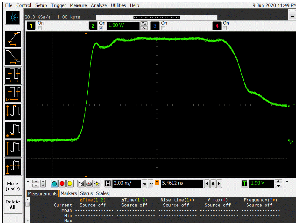
Figure 9a DUT 1014 Pre-Irradiation Rising Edge
