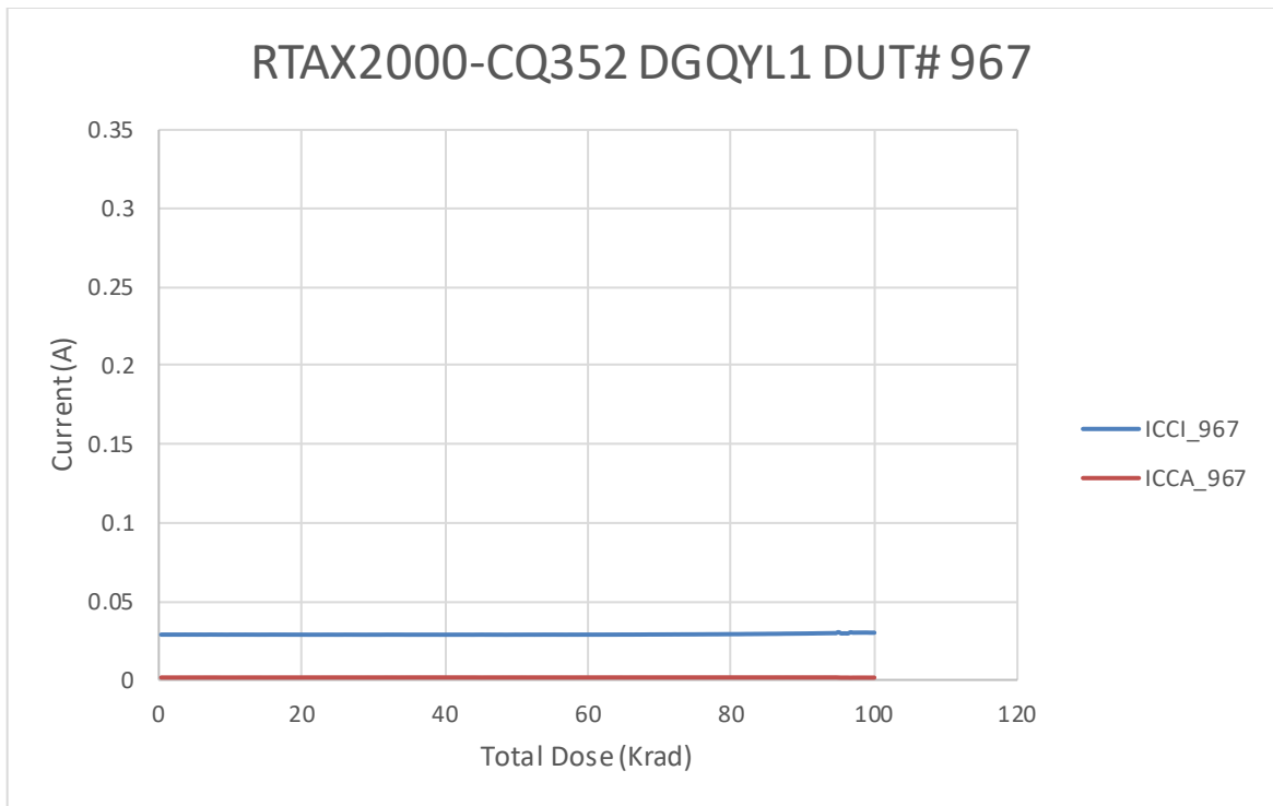
Figure 2 DUT 967 Influx ICCA and ICCI
