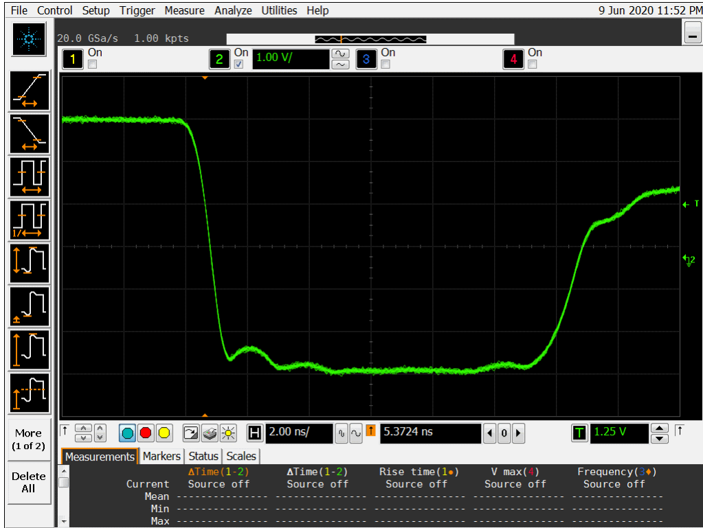
Figure 16a DUT 1018 Pre-Irradiation Falling Edge
