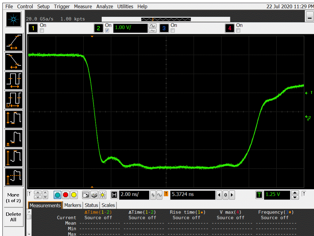
Figure 17b DUT 994 Post-Annealing Falling Edge
