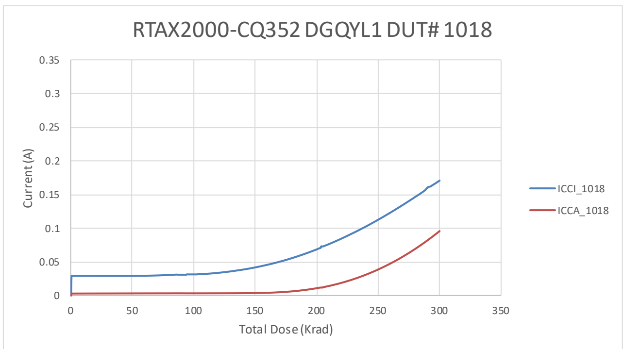
Figure 7 DUT 1018 Influx ICCA and ICCI
