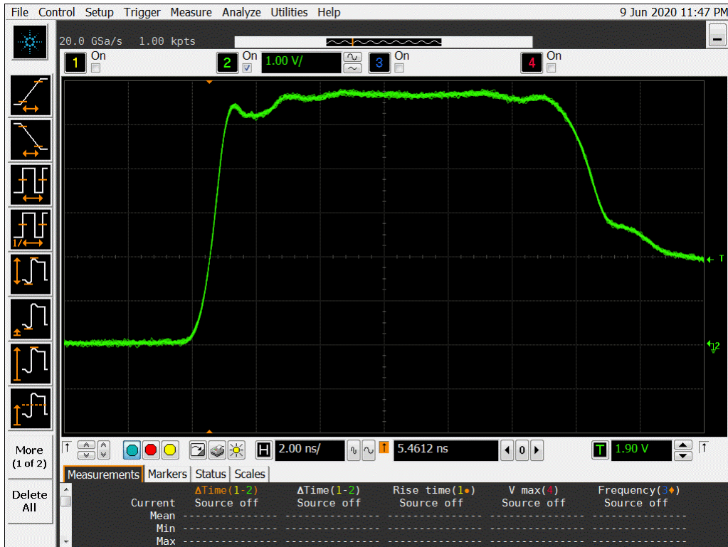
Figure 12a DUT 996 Pre-Irradiation Rising Edge
