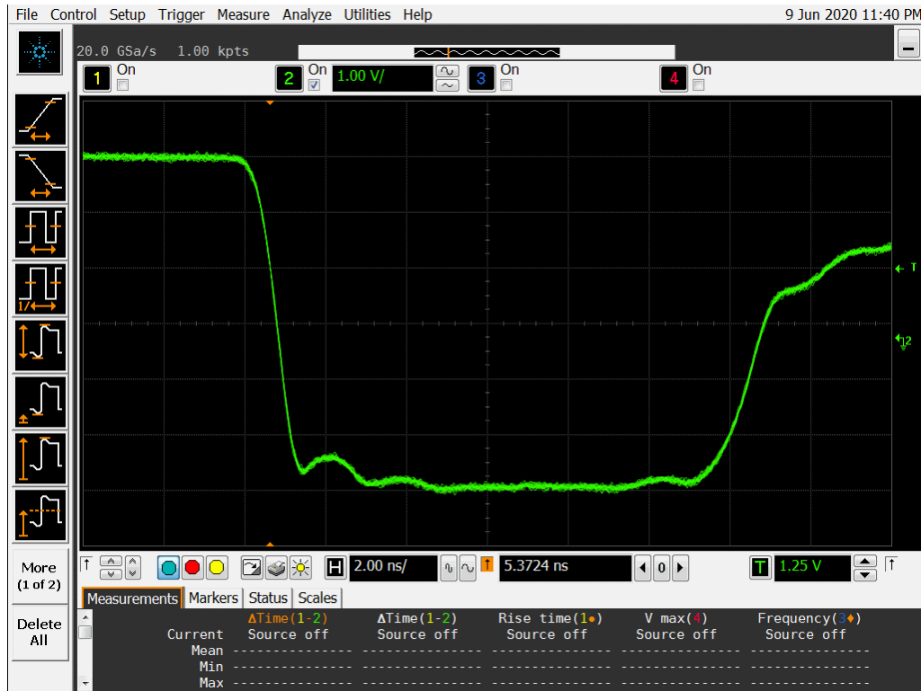
Figure 19a DUT 967 Pre-Irradiation Falling Edge
