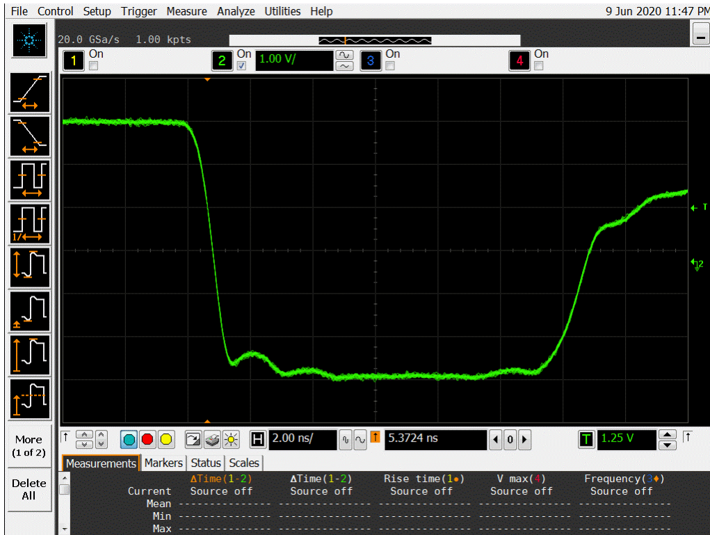
Figure 18a DUT 996 Pre-Irradiation Falling Edge
