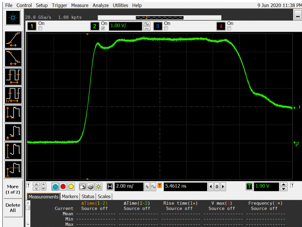
Figure 13a DUT 967 Pre-Irradiation Rising Edge
