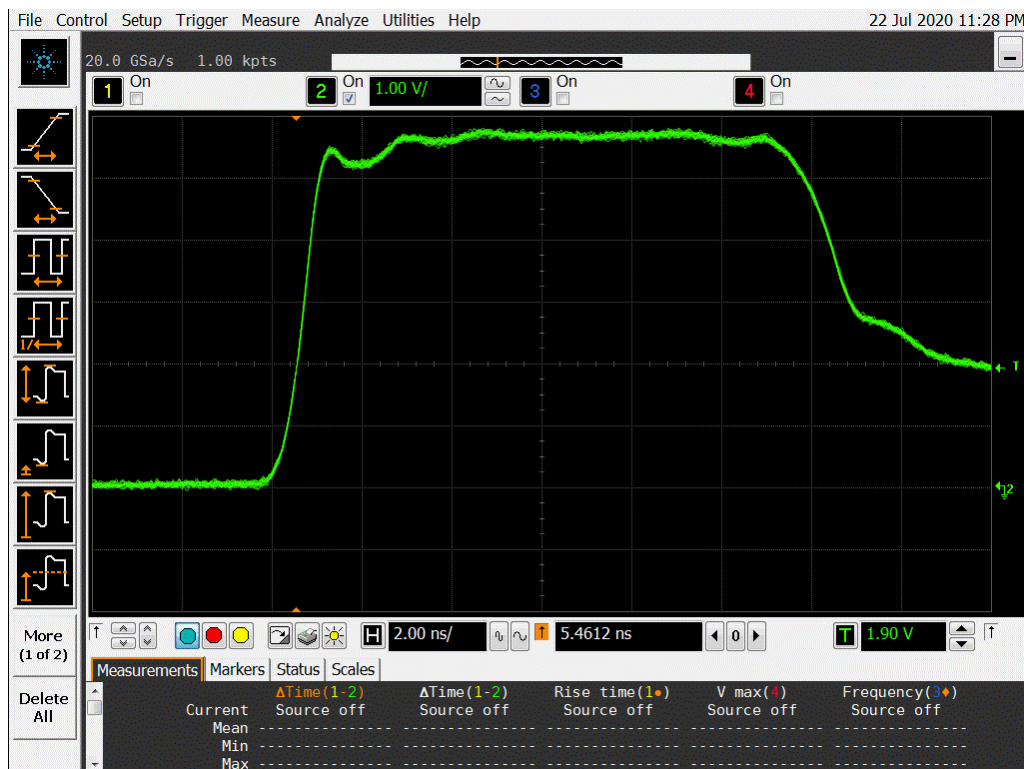
Figure 11b DUT 994 Post-Annealing Rising edge
