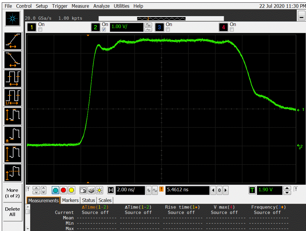
Figure 12b DUT 996 Post-Annealing Rising Edge
