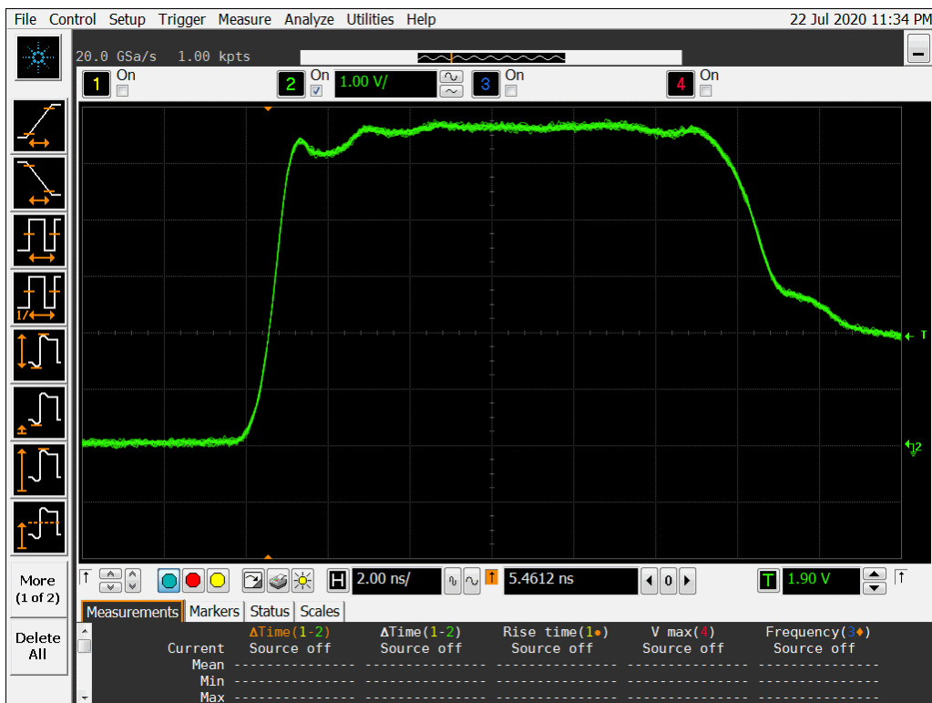
Figure 10b DUT 1018 Post-Annealing Rising Edge
