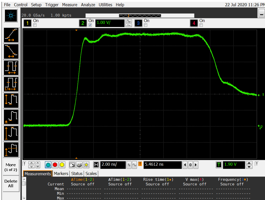
Figure 14b DUT 970 Post-Annealing Rising Edge
