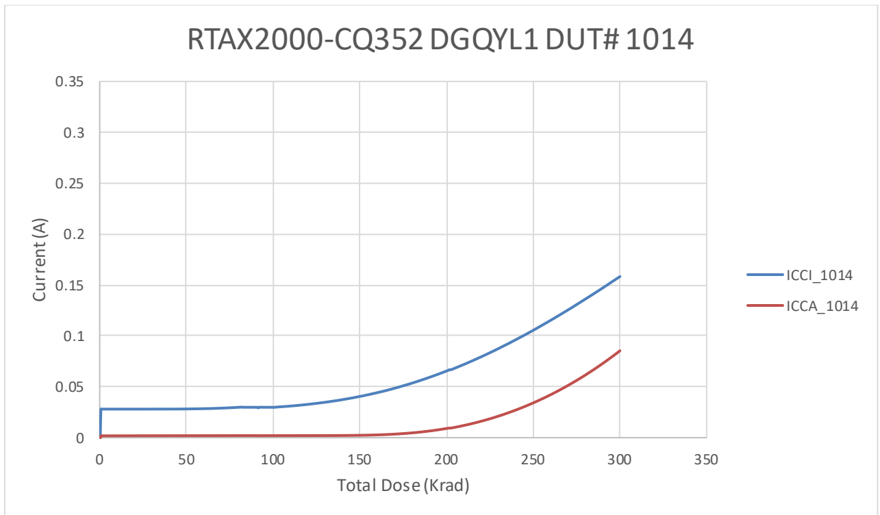
Figure 6 DUT1014 Influx ICCA and ICCI
