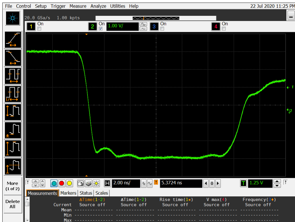
Figure 19b DUT 967 Post-Annealing Falling Edge
