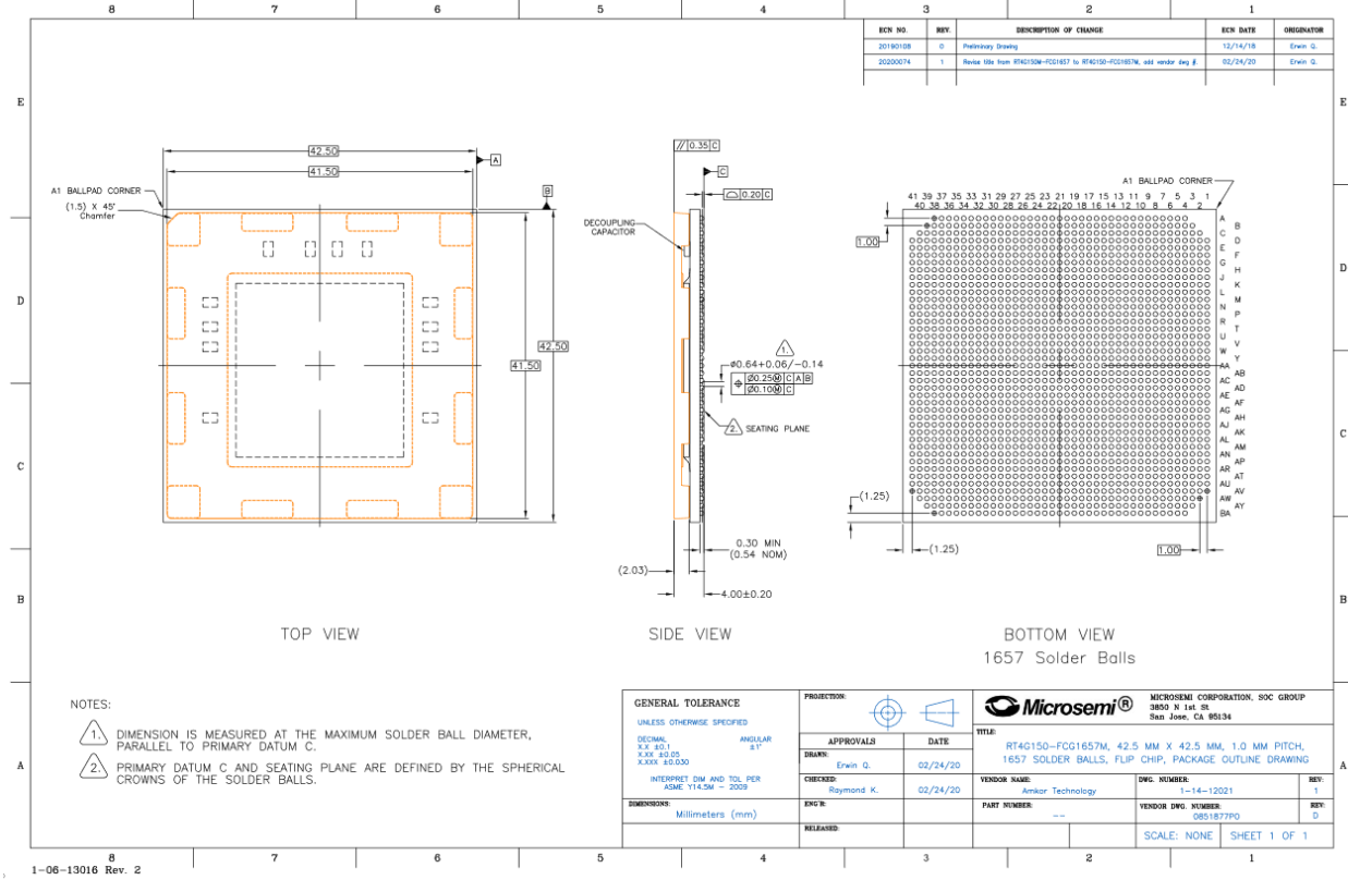
Figure 1-1. Package Mechanical Drawing
