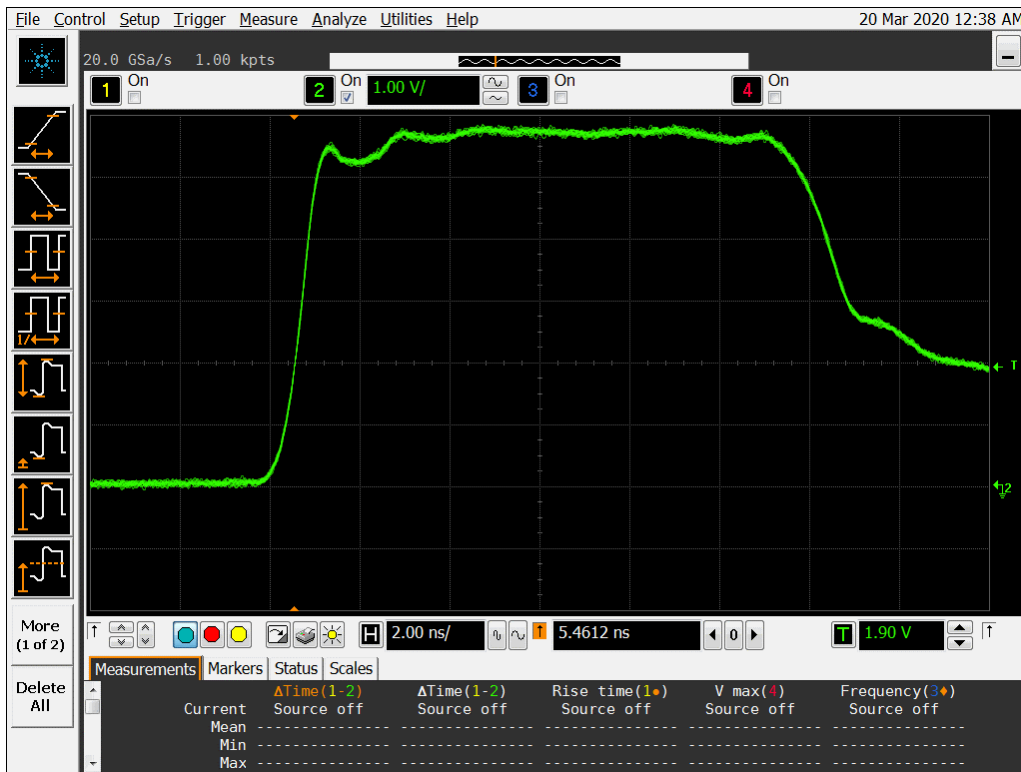
Figure 12b DUT 13798 Post-Annealing Rising Edge
