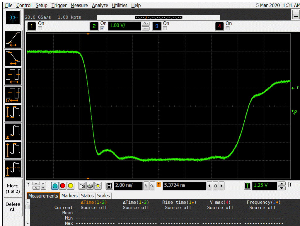
Figure 13a DUT 13822 Pre-Radiation Falling Edge
