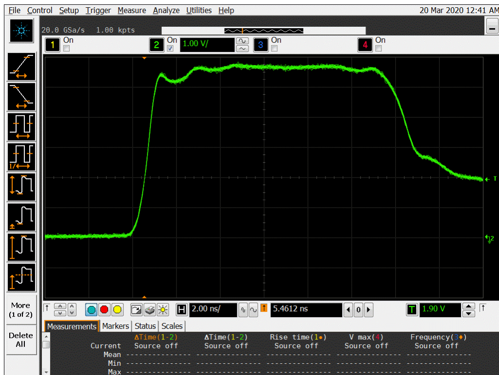
Figure 10b DUT 13801 Post-Annealing Rising edge
