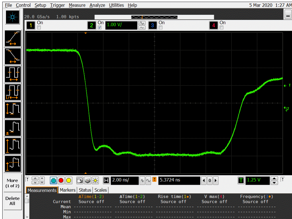
Figure 14a DUT 13801 Pre-Irradiation Falling Edge
