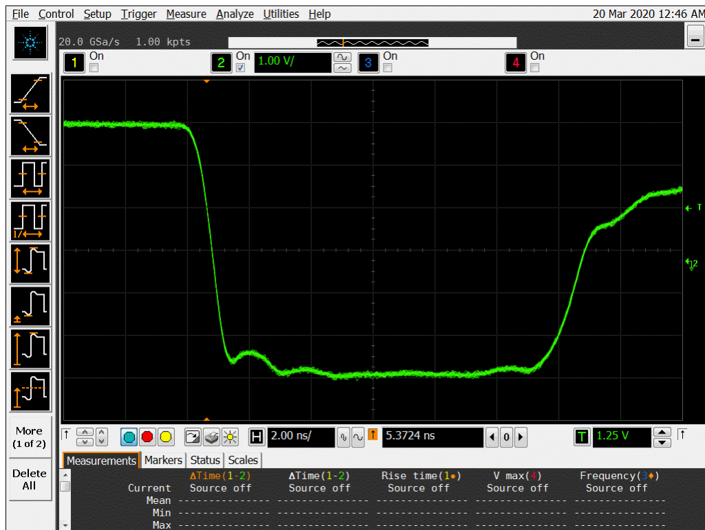
Figure 13b DUT 13822 Post-Annealing Falling Edge
