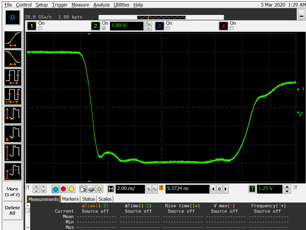
Figure 15a DUT 13812 Pre-Irradiation Falling Edge
