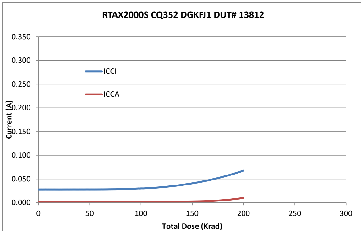
Figure 4 DUT 13812 Influx ICCA and ICCI
