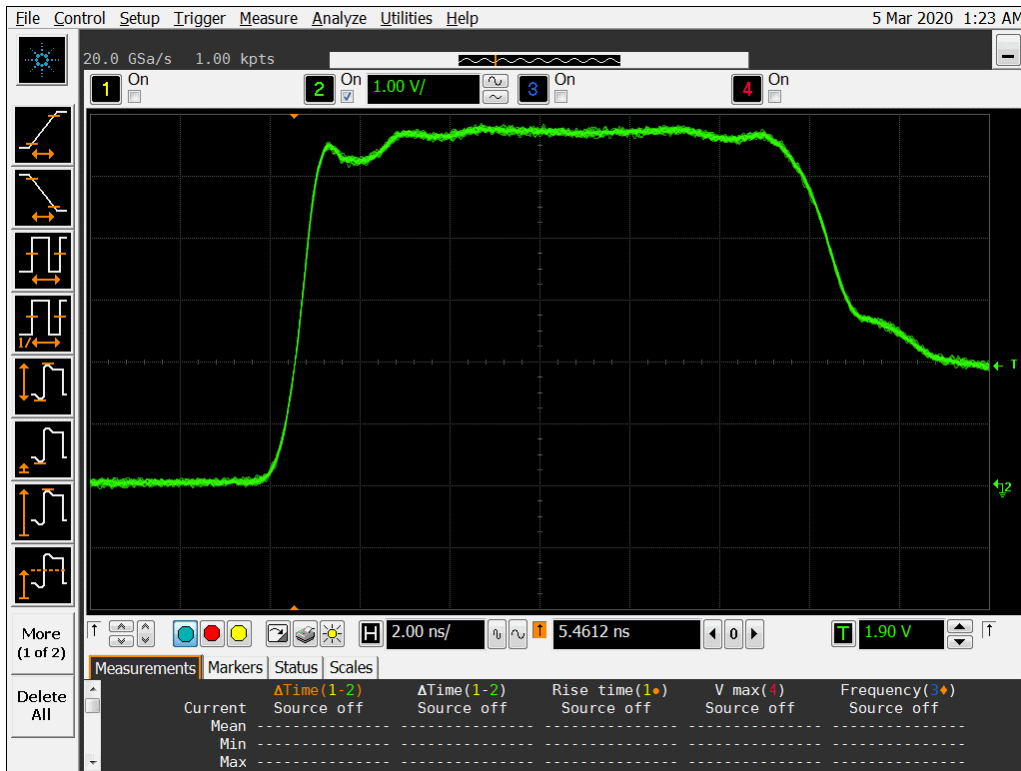
Figure 12a DUT 13798 Pre-Irradiation Rising Edge
