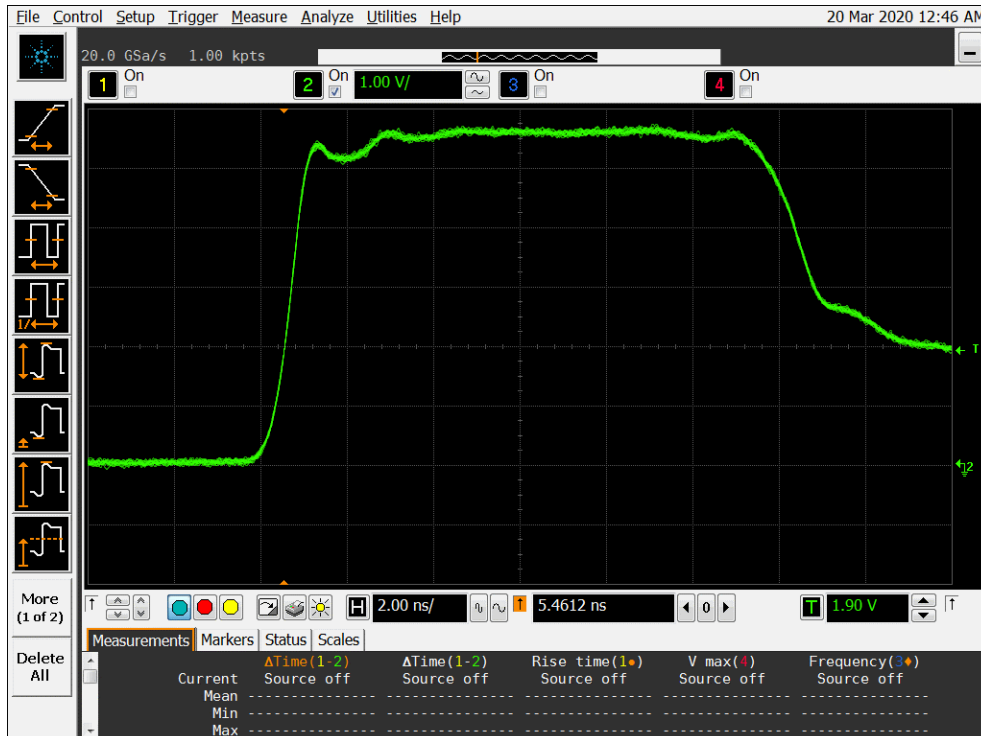
Figure 9b DUT 13822 Post-Annealing Rising Edge
