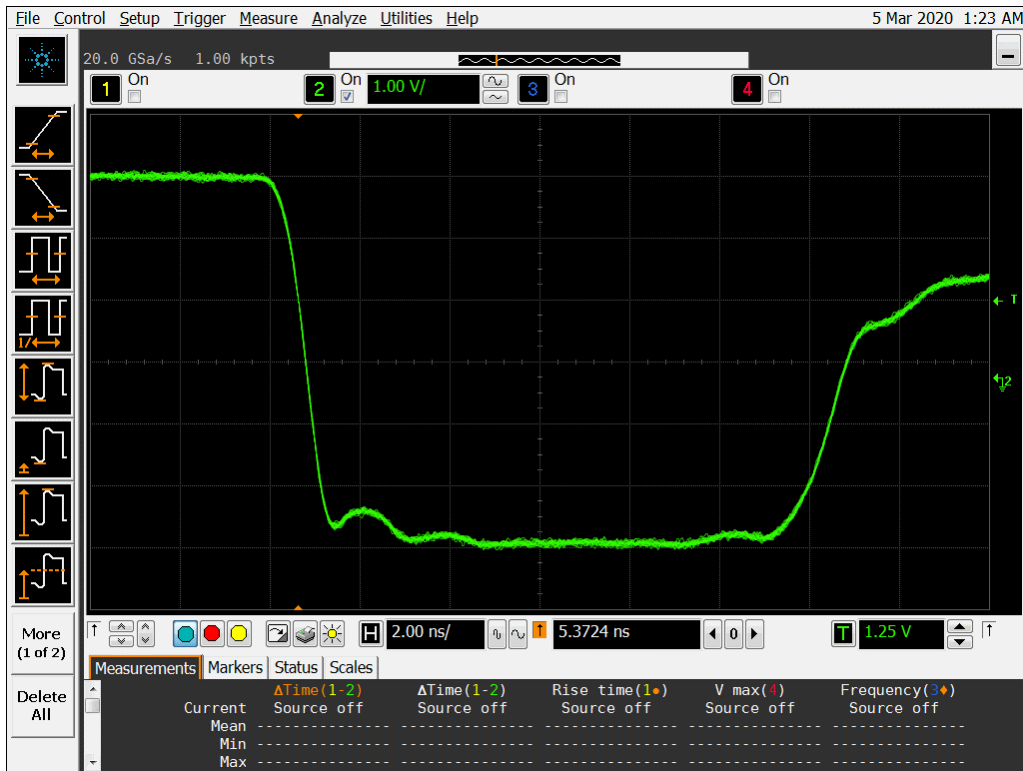
Figure 16a DUT 13798 Pre-Irradiation Falling Edge
