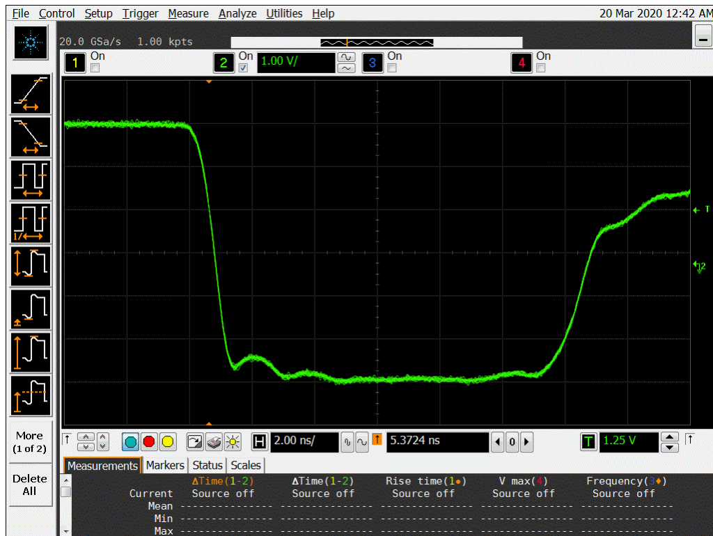
Figure 14b DUT 13801 Post-Annealing Falling Edge
