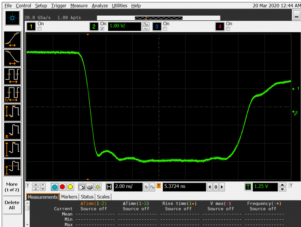
Figure 15b DUT 13812 Post-Annealing Falling Edge
