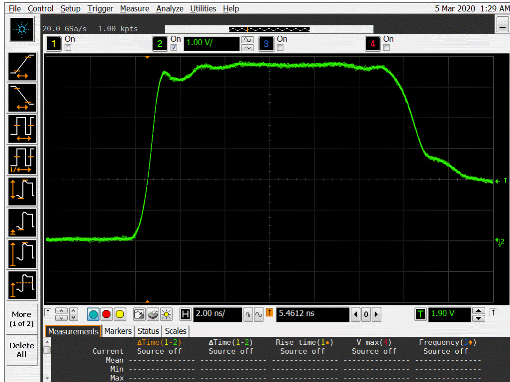
Figure 11a DUT 13812 Pre-Irradiation Rising Edge
