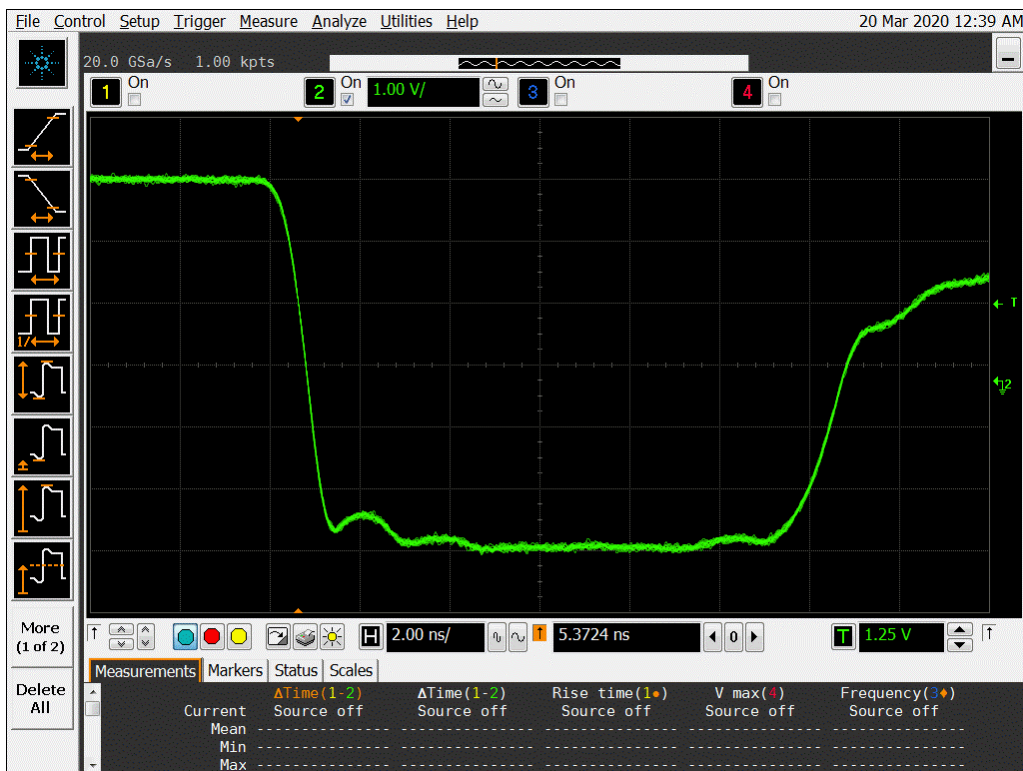
Figure 16b DUT 13798 Post-Annealing Falling Edge
