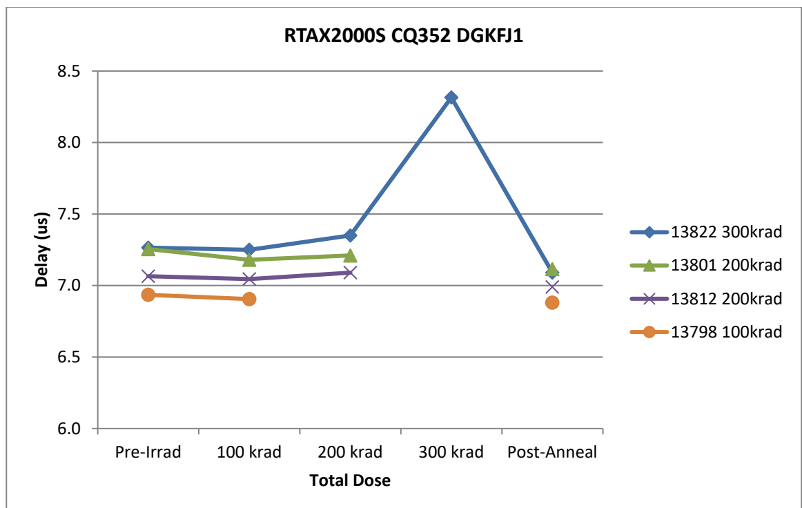
Figure 6 In-Situ Propagation Delay versus Total Dose
