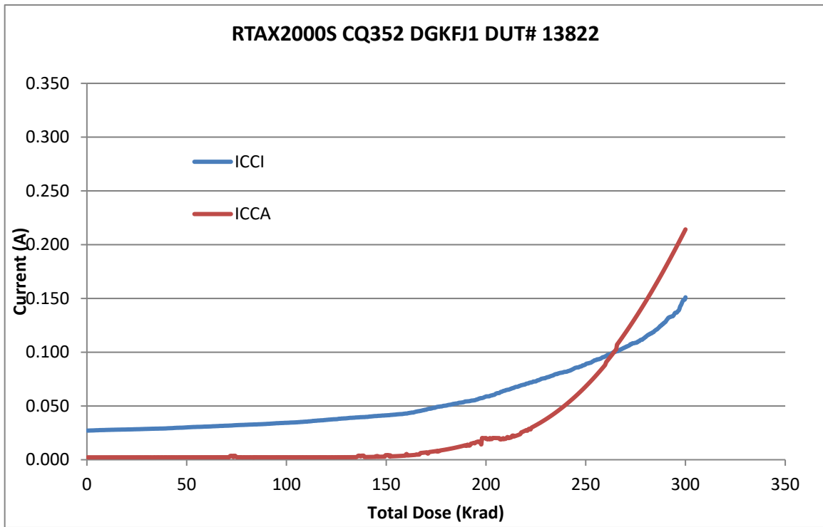
Figure 2 DUT 13822 Influx ICCA and ICCI
