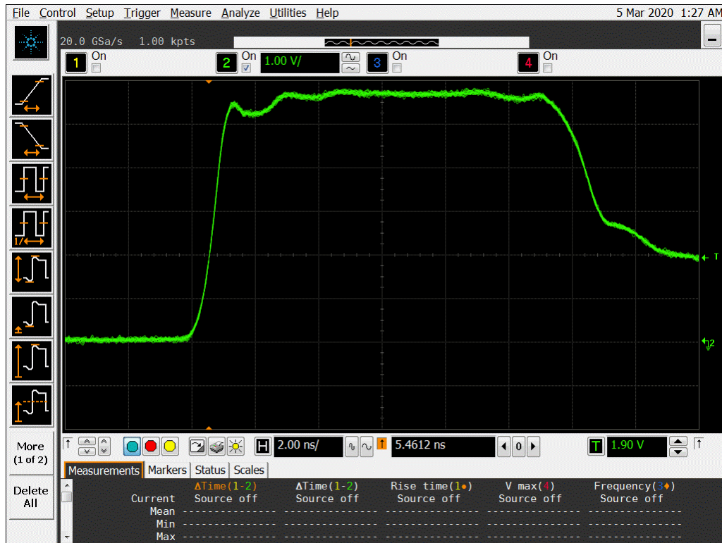
Figure 10a DUT 13801 Pre-Radiation Rising Edge
