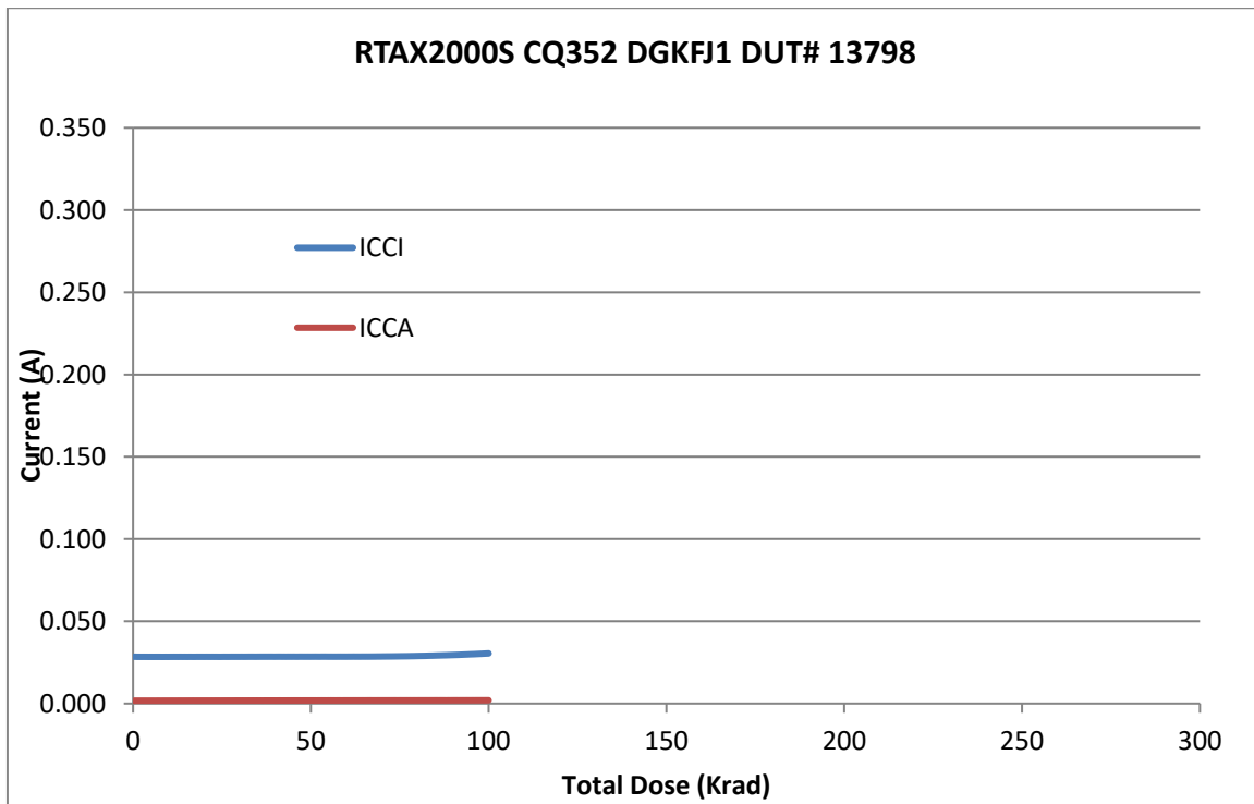
Figure 5 DUT 13798 Influx ICCA and ICCI
