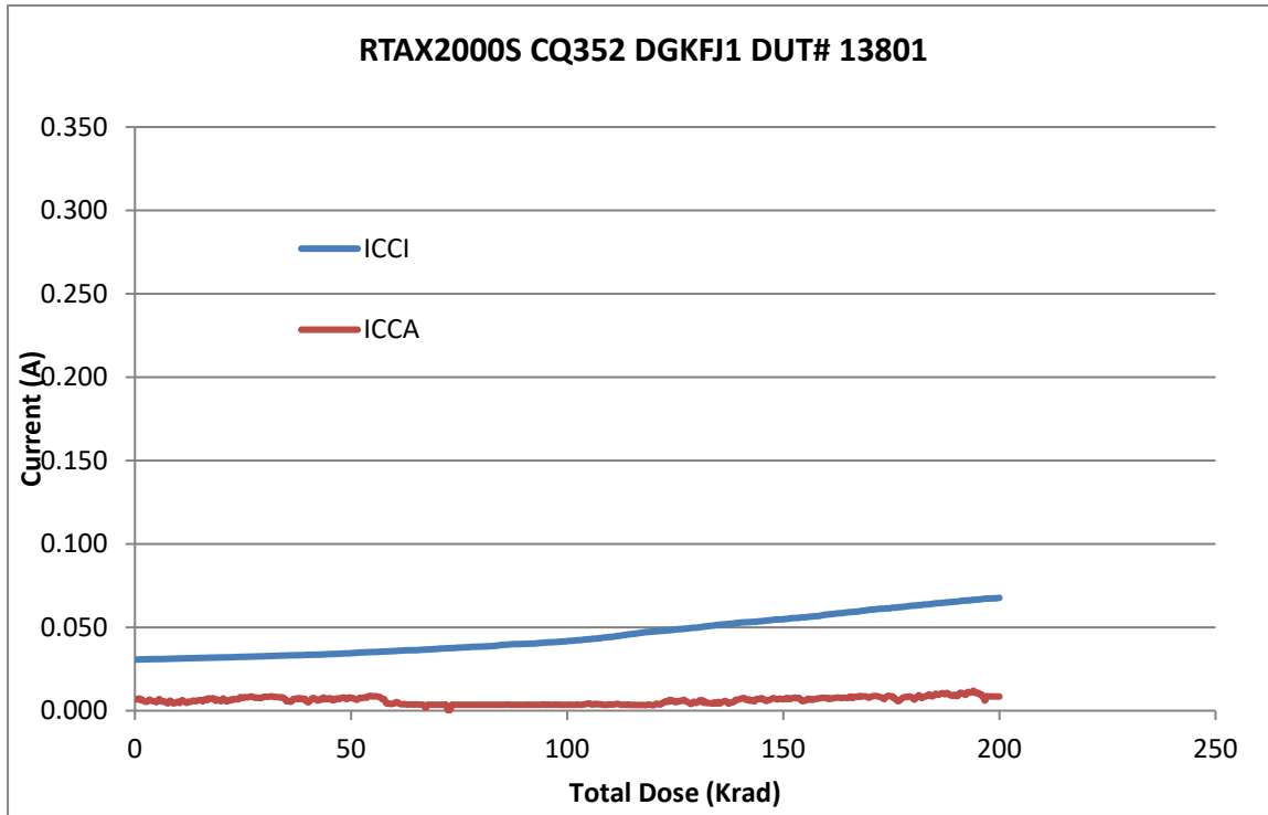
Figure 3 DUT 13801 Influx ICCA and ICCI
