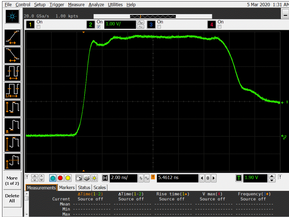
Figure 9a DUT 13822 Pre-Irradiation Rising Edge
