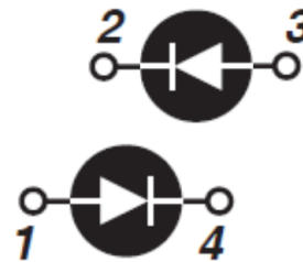
Figure 2 • Anti-parallel MSC2X50SDA070J
