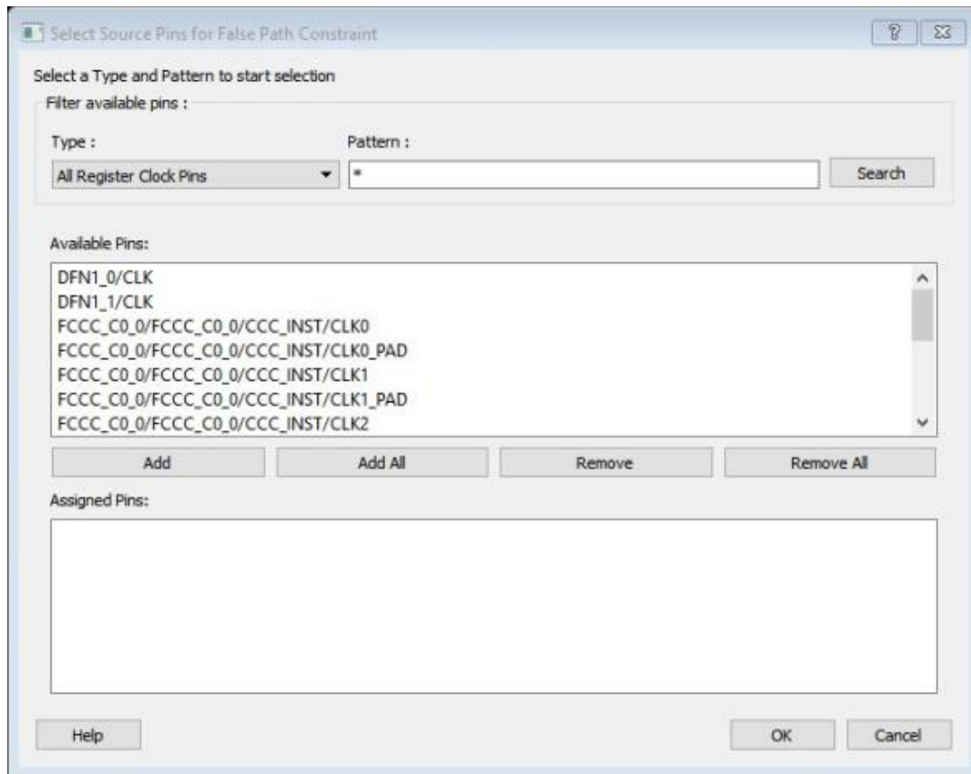
Figure 64 · Select Source Pins for False Path Constraint Dialog Box
