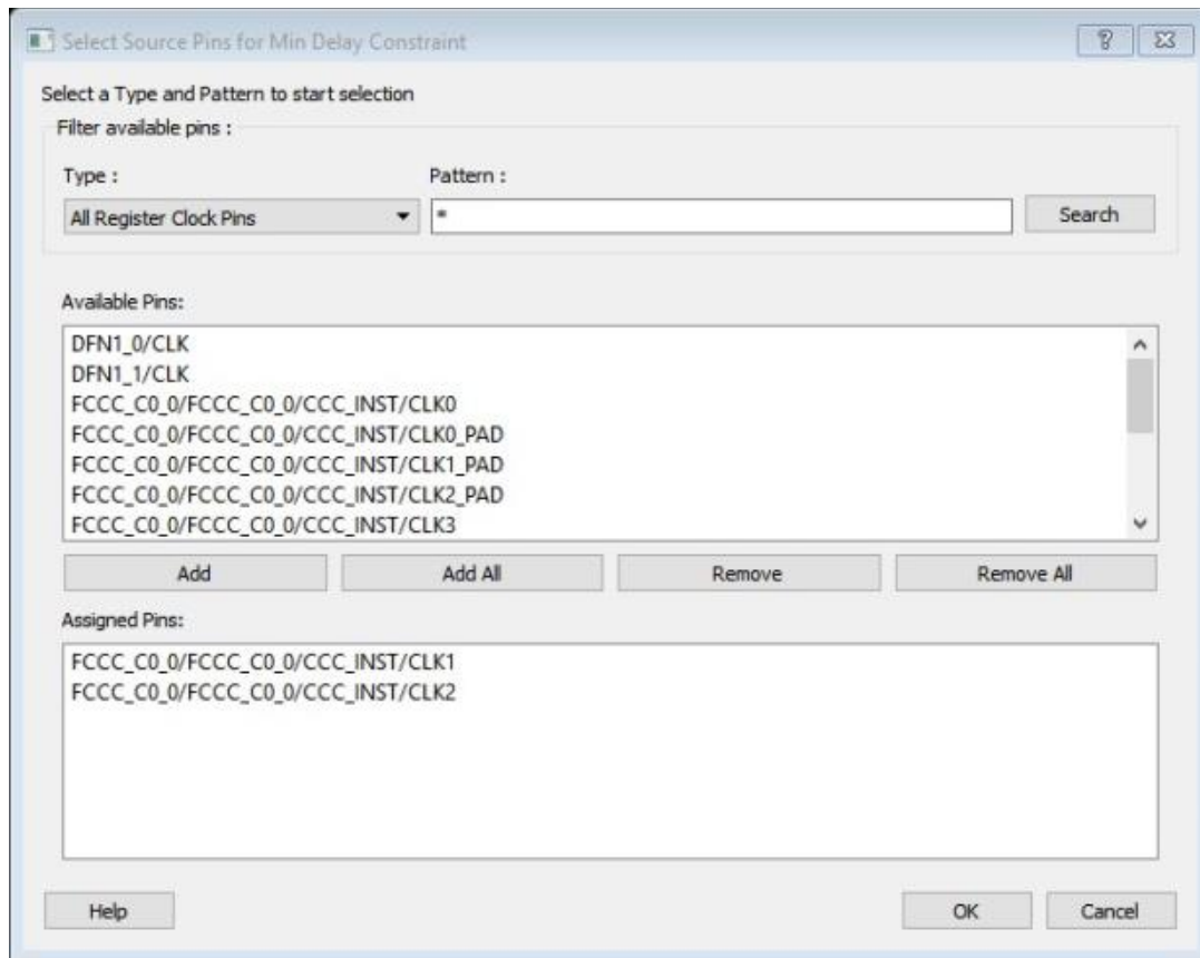
Figure 60 · Select Source Pins for Min Delay Constraint Dialog Box
