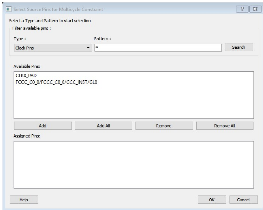
Figure 62 · Select Source Pins for Multicycle Constraint Dialog Box
