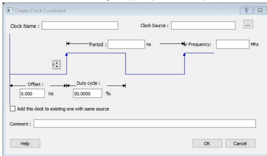
Figure 65 · Create Clock Constraint Dialog Box
