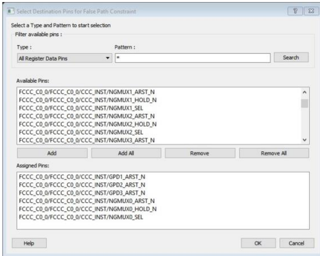
Figure 31 · Select Destination Pins for False Path Constraint Dialog Box
