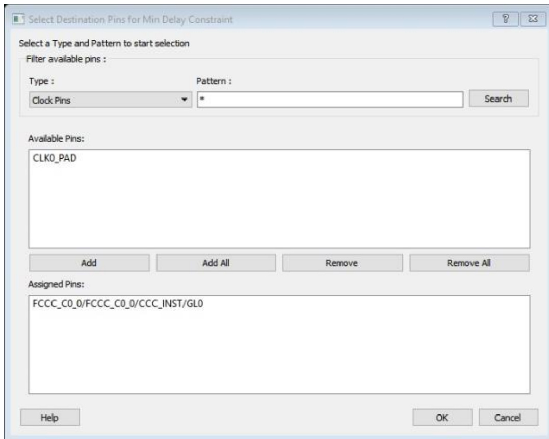
Figure 23 · Select Destination Pins for Min Delay Constraint Dialog Box
