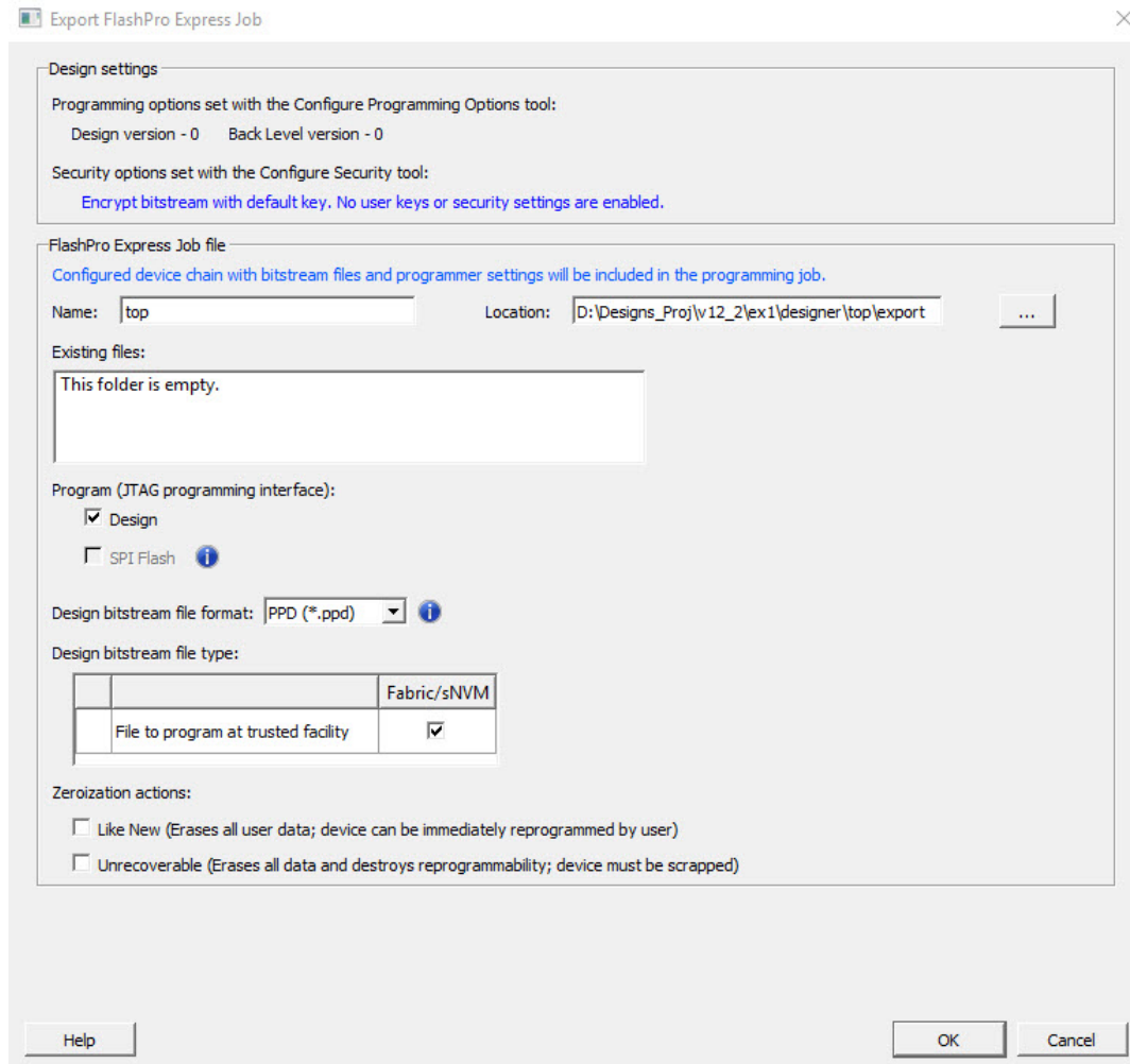
Figure 3 · Export FlashPro Express Job
