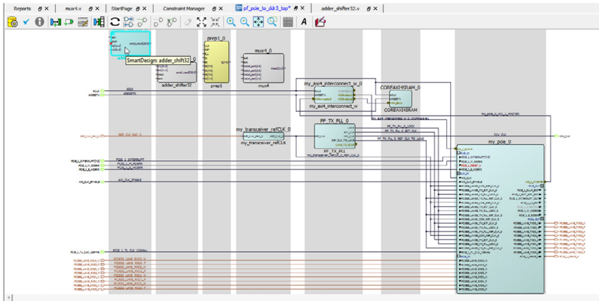
Figure 1 • SmartDesign Canvas
