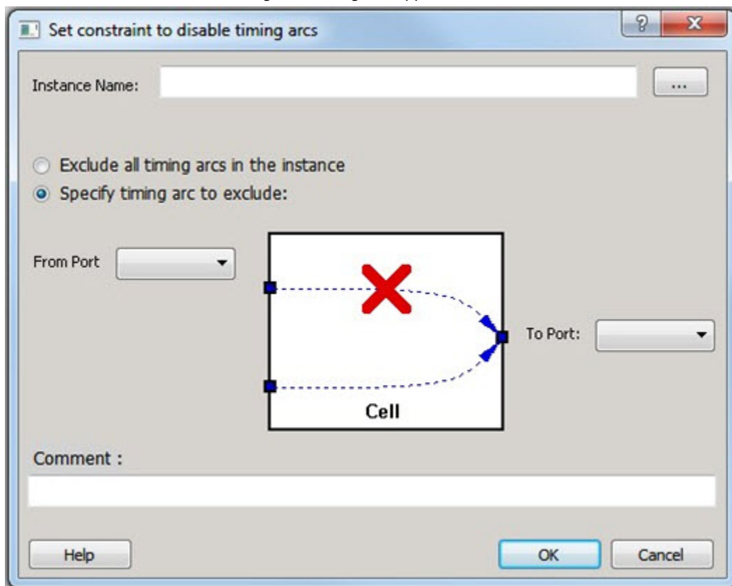
Figure 31 · Set constraint to disable timing arcs Dialog Box
