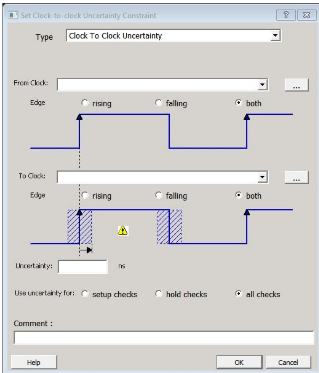
Figure 37 · Set Clock-to-Clock Uncertainty Constraint Dialog Box
