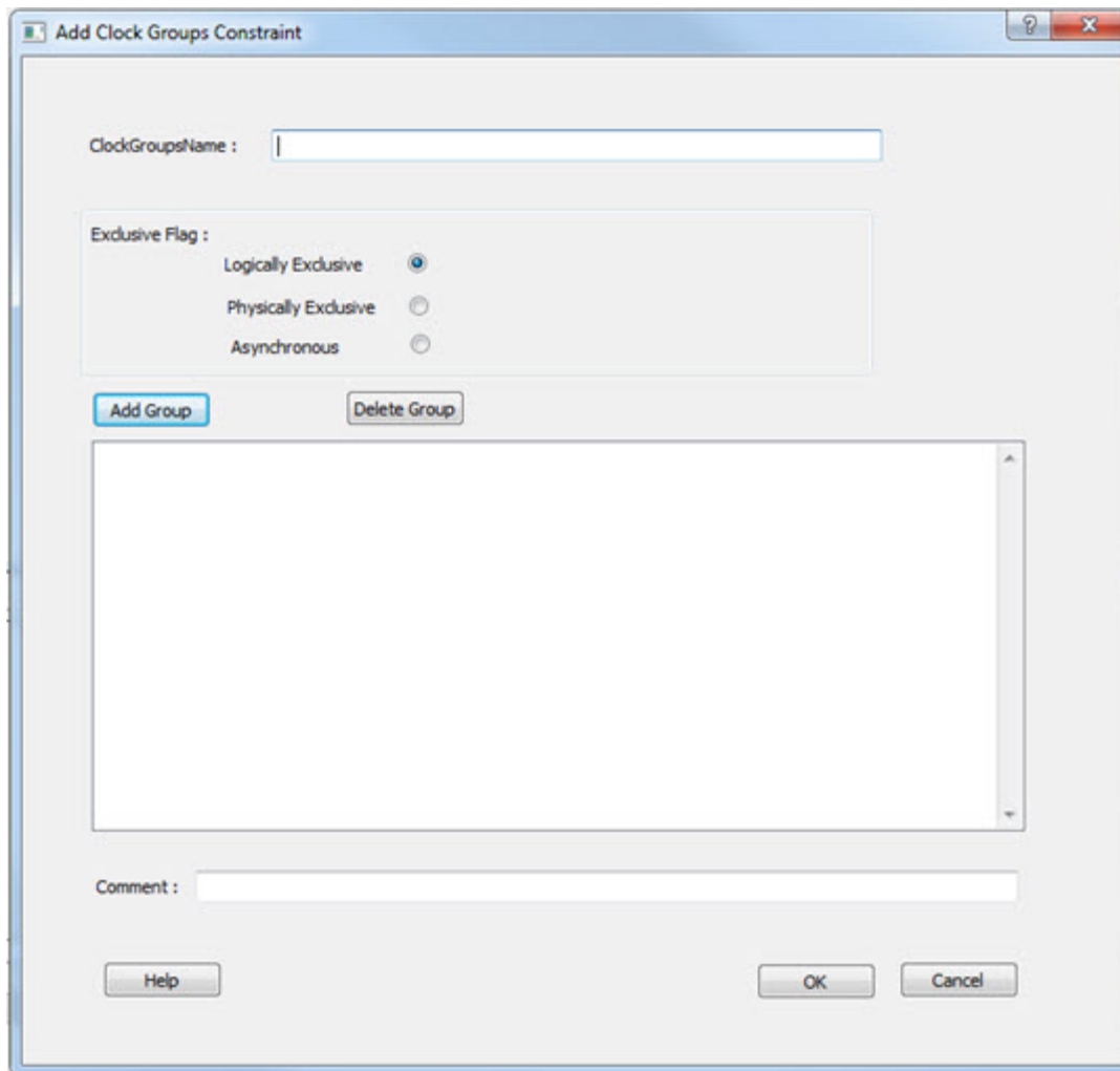
Figure 40 · Add Clock Groups Constraints Dialog Box
