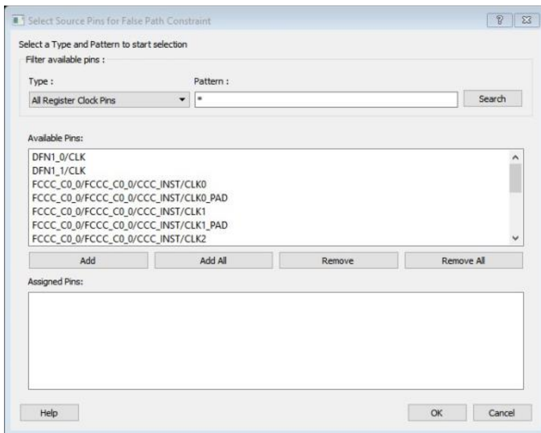
Figure 62 · Select Source Pins for False Path Constraint Dialog Box
