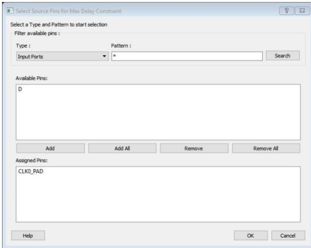
Figure 16 · Select Source Pins for Max Delay Constraint Dialog Box
