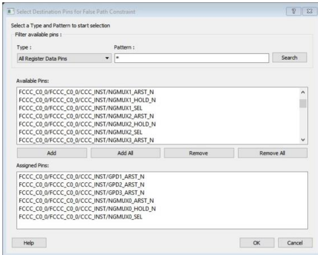
Figure 30 · Select Destination Pins for False Path Constraint Dialog Box
