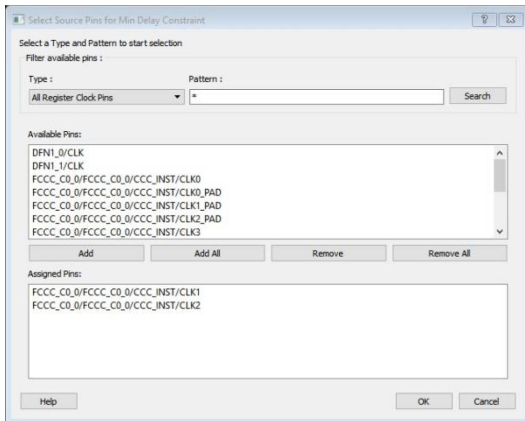
Figure 20 · Select Source Pins for Min Delay Constraint Dialog Box
