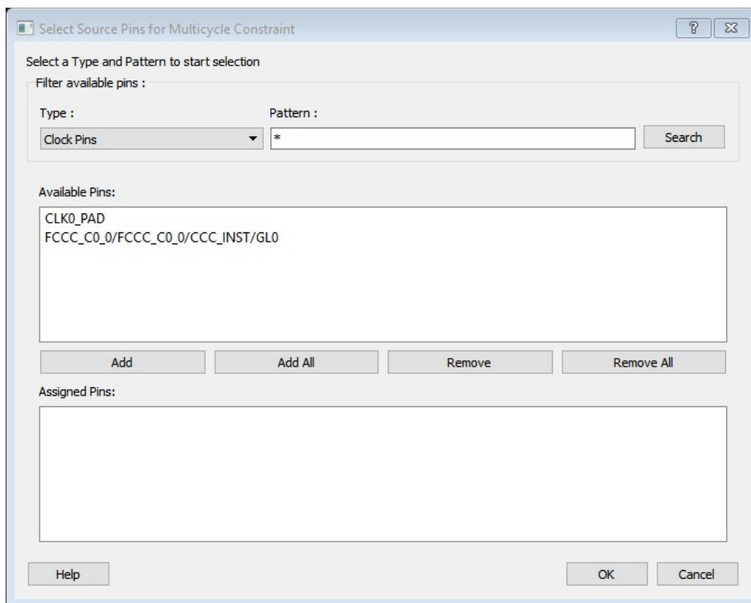
Figure 24 · Select Source Pins for Multicycle Constraint Dialog Box
