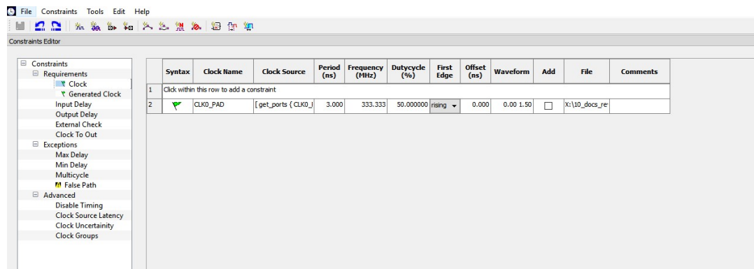
Figure 64 · Timing Constraint View
