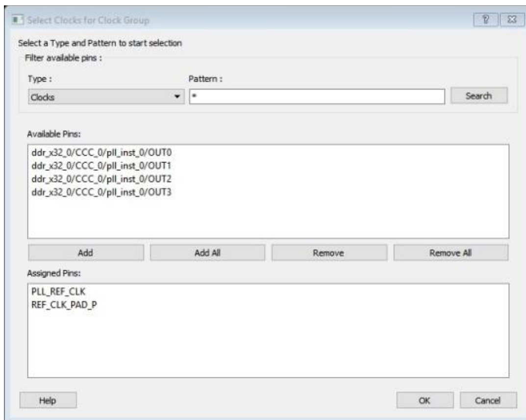
Figure 41 · Add Clocks For Clock Group Dialog Box
