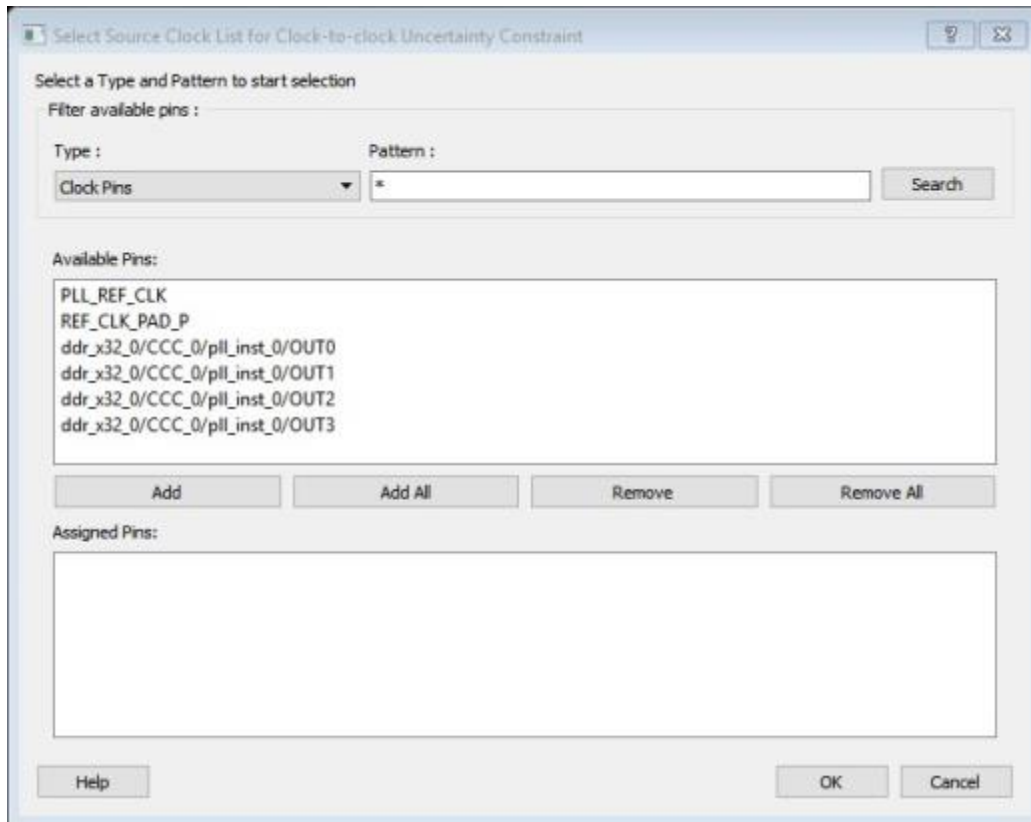
Figure 38 · Select Source Clock List for Clock-to-Clock Uncertainty Dialog Box
