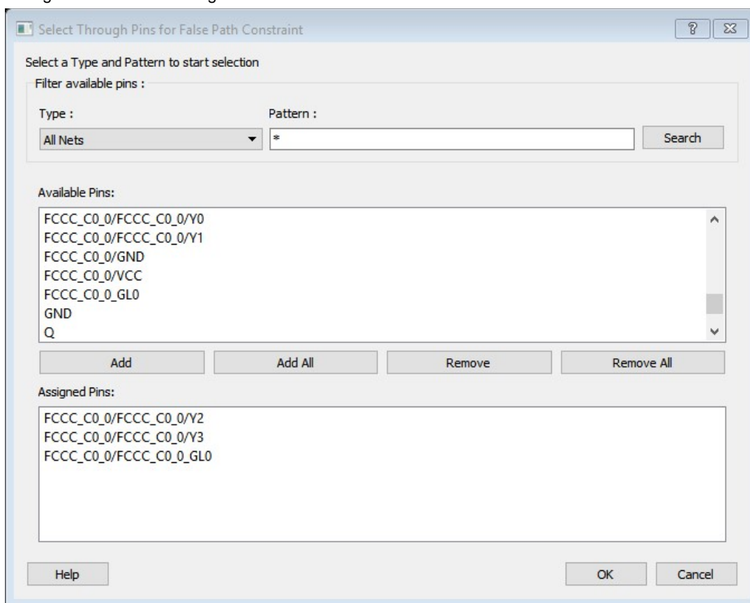
Figure 53 · Select Through Pins for False Path Constraint Dialog Box
