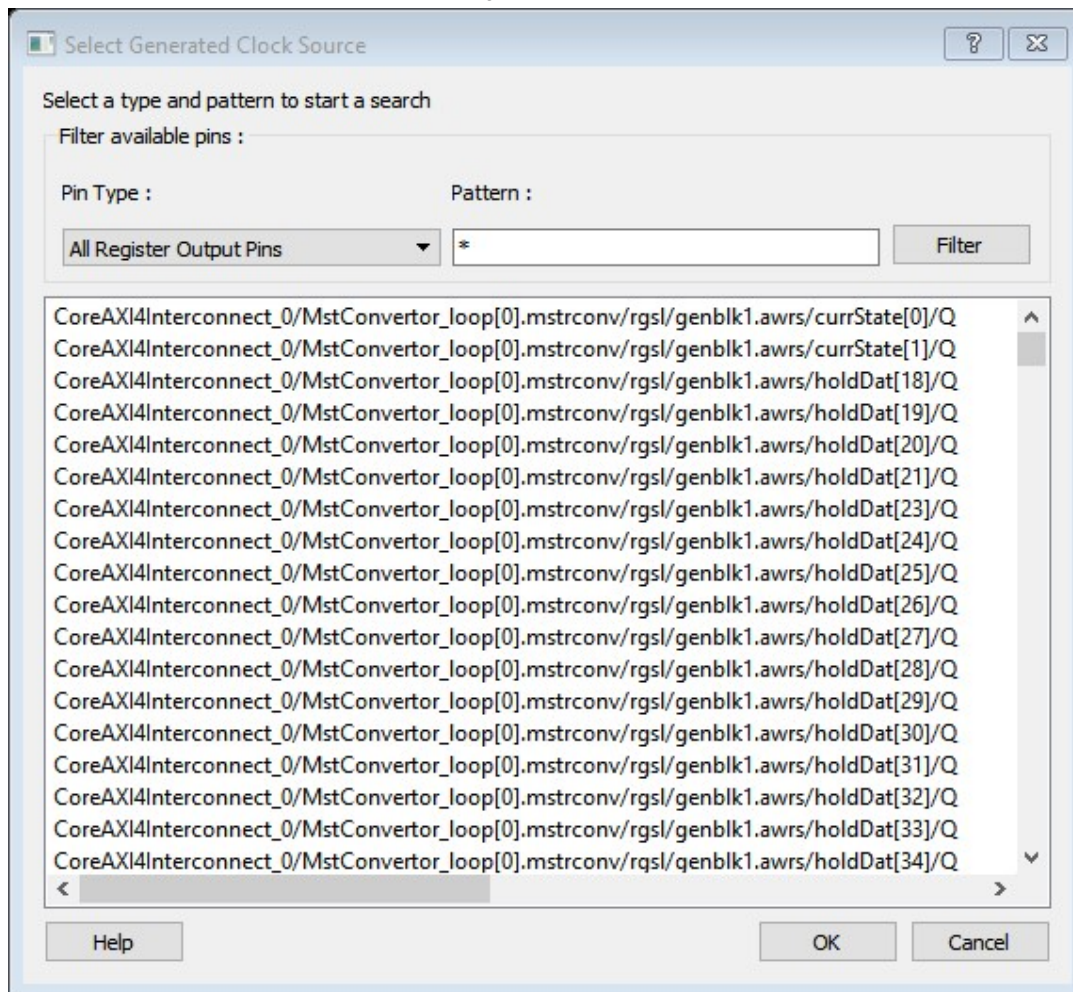
Figure 56 · Select Generated Clock Source Dialog Box
