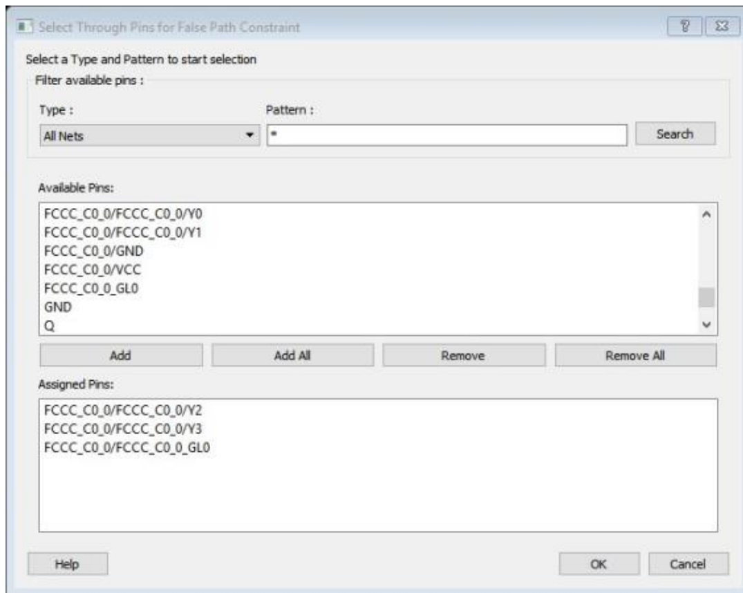
Figure 29 · Select Through Pins for False Path Constraint Dialog Box
