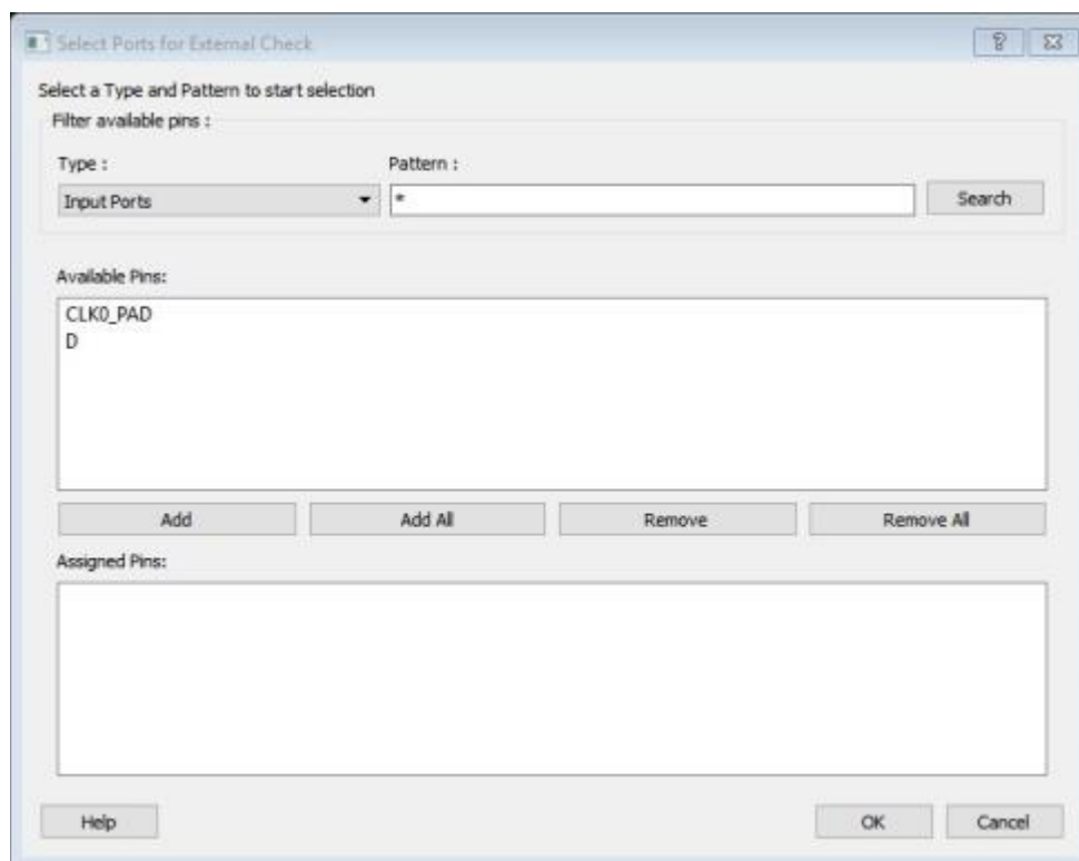
Figure 12 · Select Ports for External Check Dialog Box
