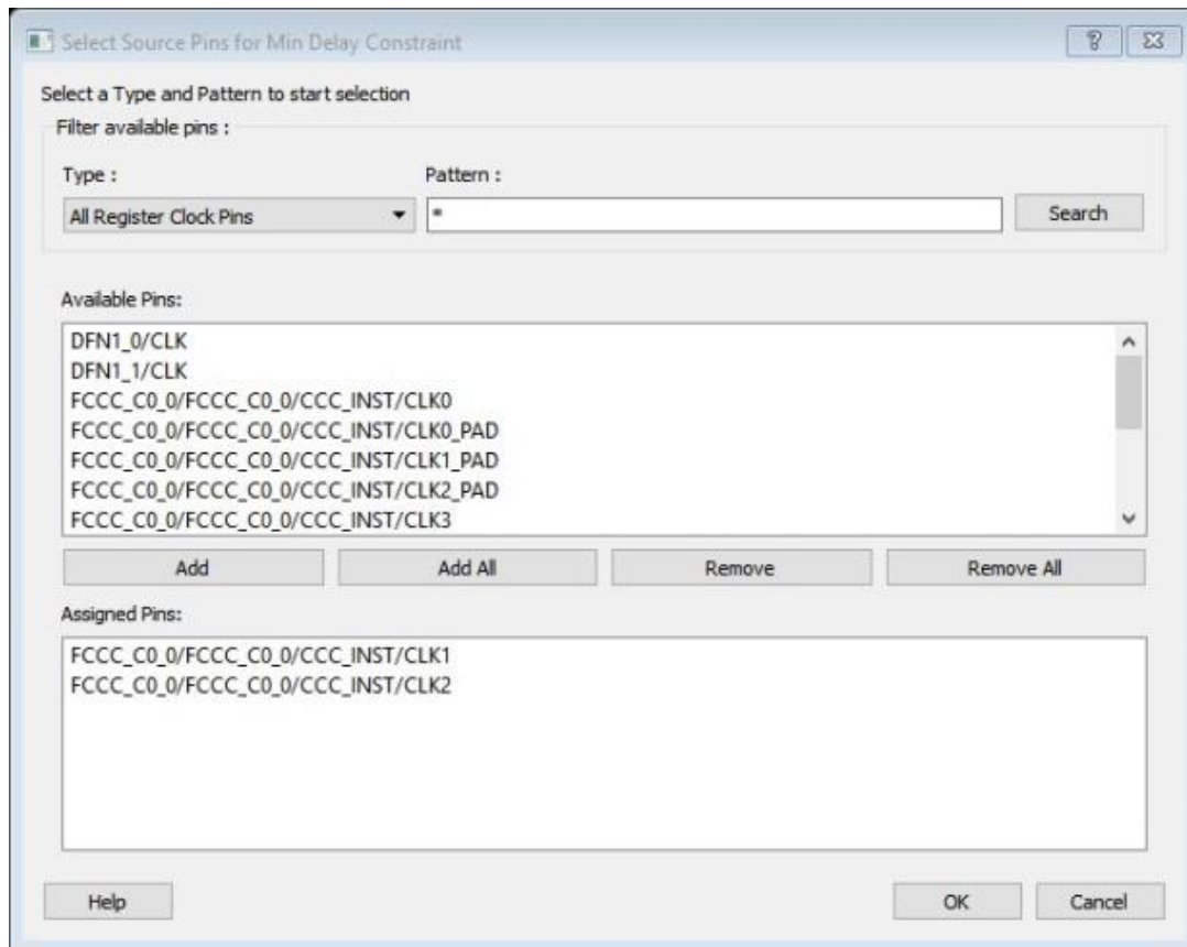
Figure 58 · Select Source Pins for Min Delay Constraint Dialog Box
