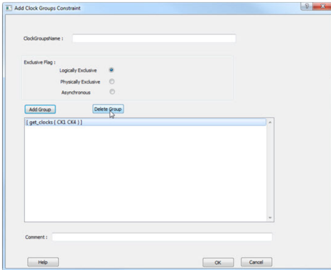
Figure 42 · Delete Group
