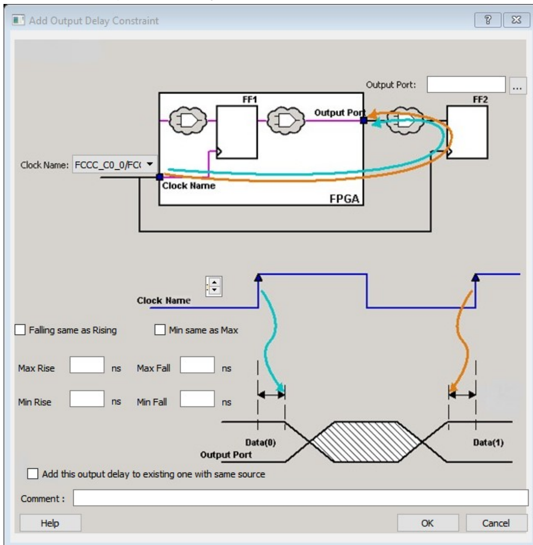
Figure 9 · Add Output Delay Constraint Dialog Box
