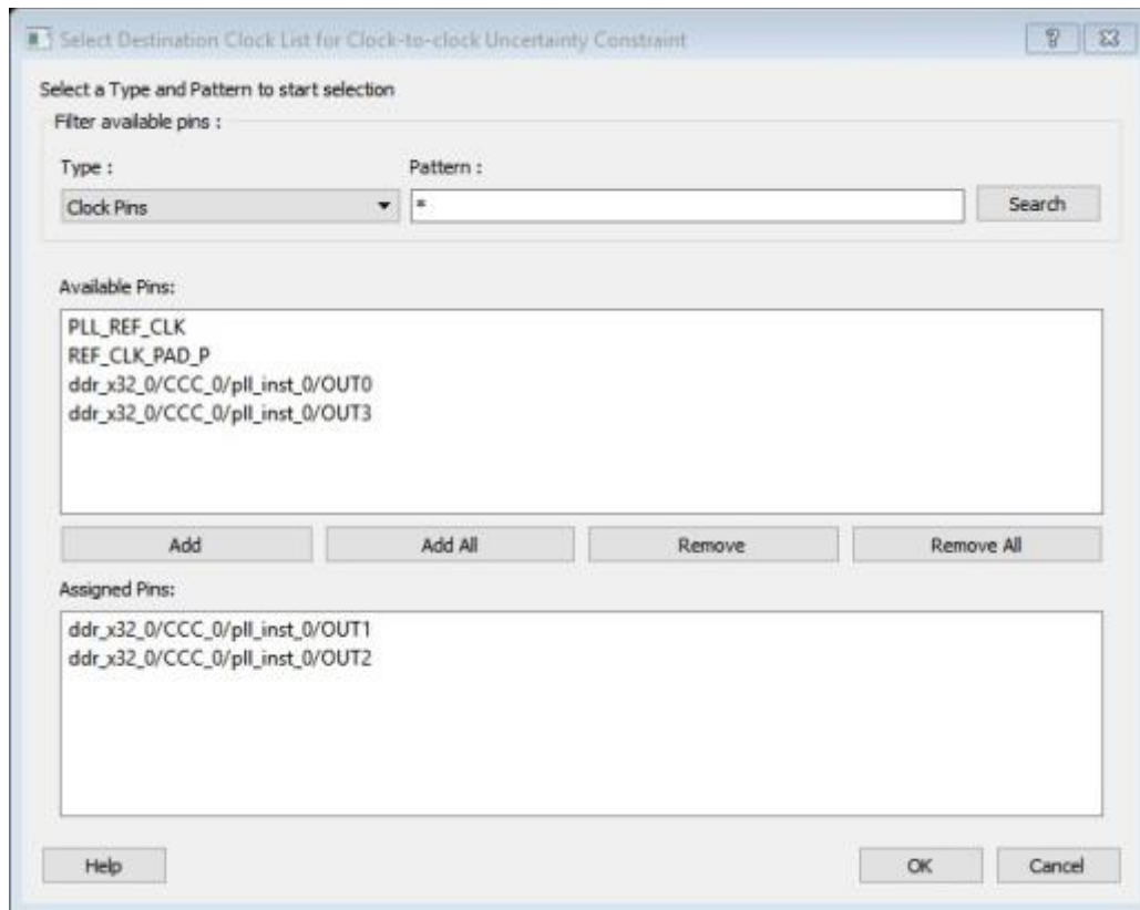
Figure 39 · Select Destination Clock List for Clock-to-Clock Uncertainty Constraint Dialog Box The Pin Type selection is for Clock Pins only.
