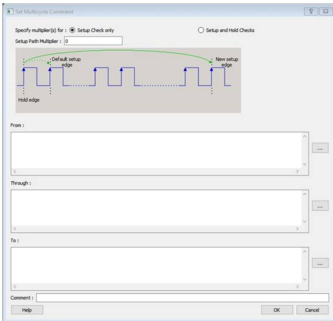
Figure 59 · Set Multicycle Constraint Dialog Box
