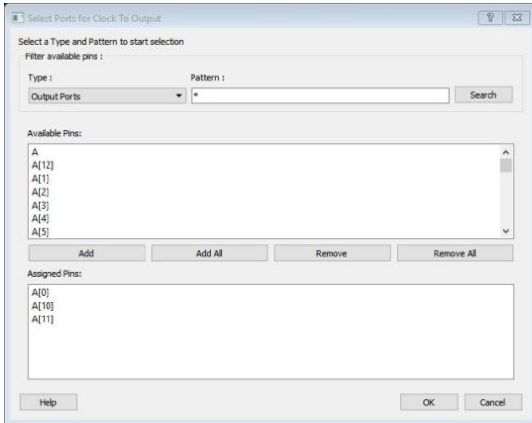
Figure 14 · Select Ports for Clock To Output Dialog Box
