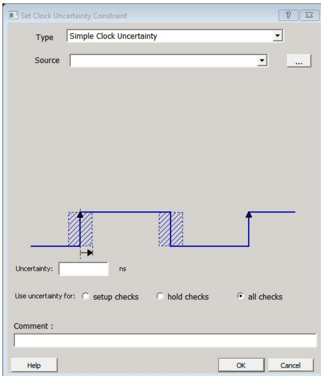
Figure 35 · Simple Clock Uncertainty constraint dialog box
