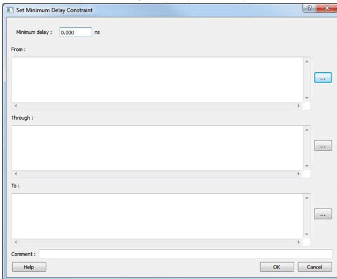
Figure 57 · Set Minimum Delay Constraint Dialog Box
