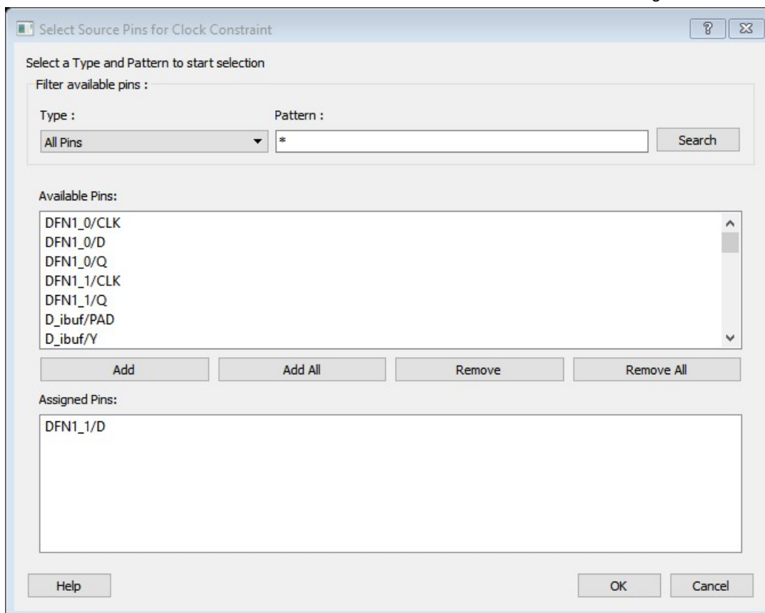
Figure 52 · Select Source Pins for Clock Constraint
