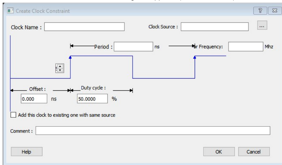
Figure 63 · Create Clock Constraint Dialog Box
