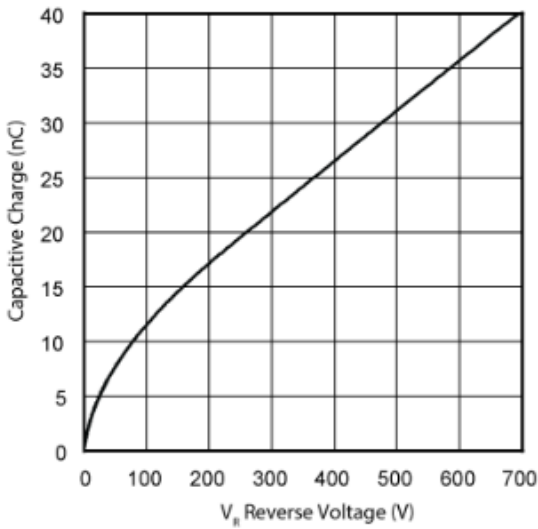
Figure 6 • Total Capacitive Charge vs. Reverse Voltage
