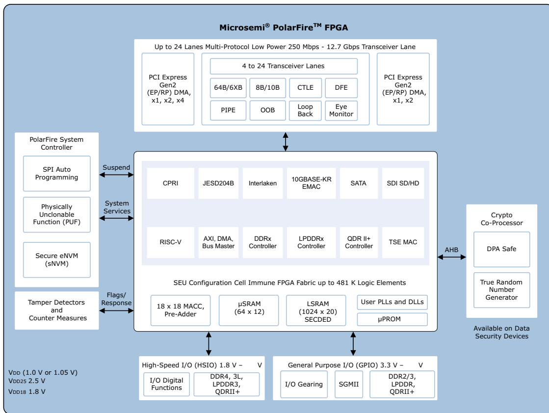
Figure 1 • Design Architecture
