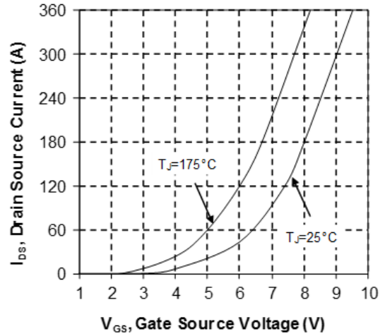
Figure 6 • Transfer Characteristics
