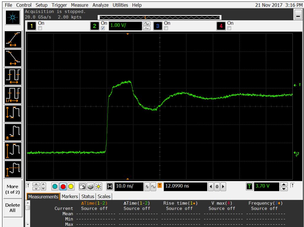
Figure 10a DUT 11027 Pre-Irradiation Rising Edge.
