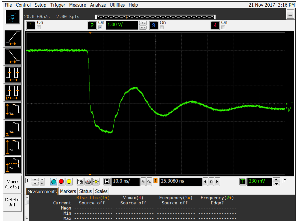
Figure 16a DUT 11027 Pre-Irradiation Falling Edge.
