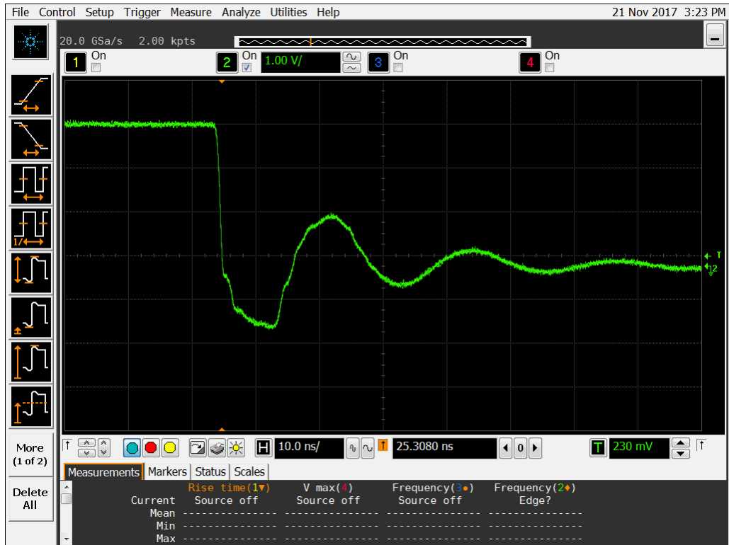
Figure 14a DUT 11044 Pre-Irradiation Falling Edge.
