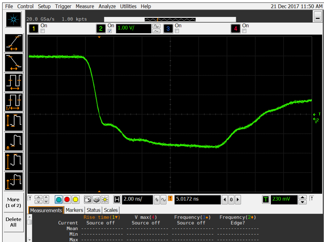
Figure 16b DUT 11027 Post-Annealing Falling Edge.
