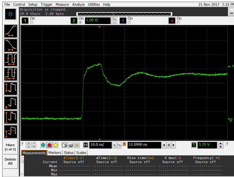
Figure 8a DUT 11044 Pre-Irradiation Rising Edge.
