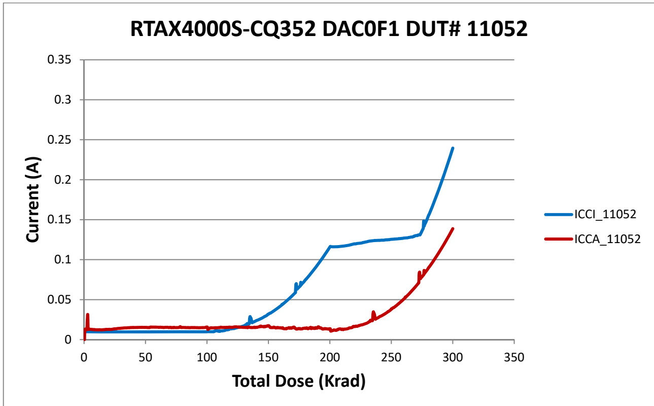
Figure 3 DUT 11052 Influx ICCI and ICCA
