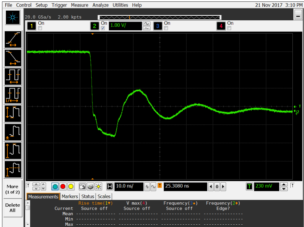
Figure 18a DUT 11019 Pre-Irradiation Falling Edge.
