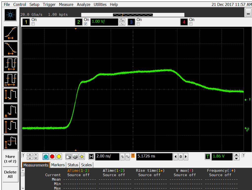
Figure 9b DUT 11052 Post-Annealing Rising Edge.
