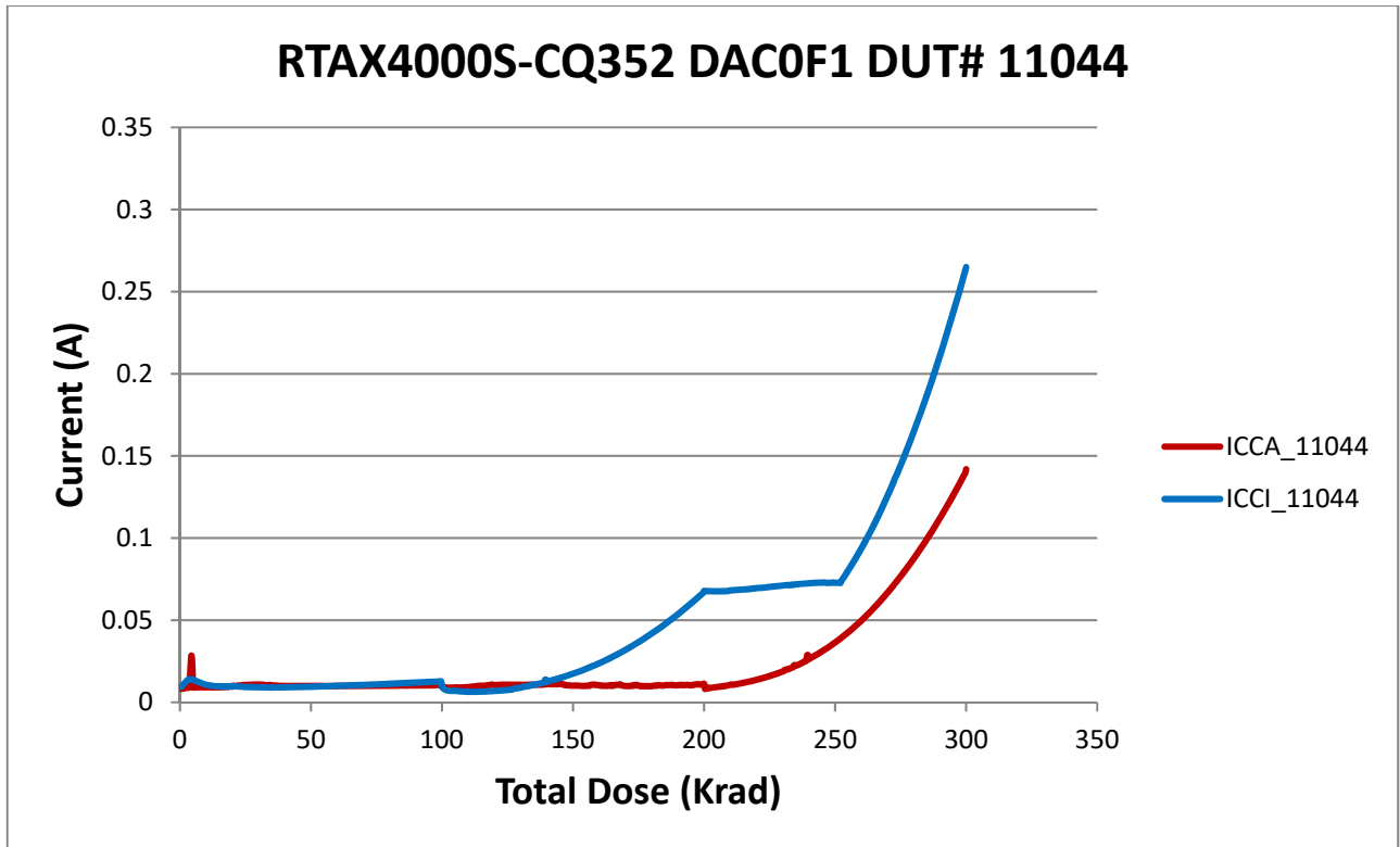
Figure 2 DUT 11044 Influx ICCI and ICCA
