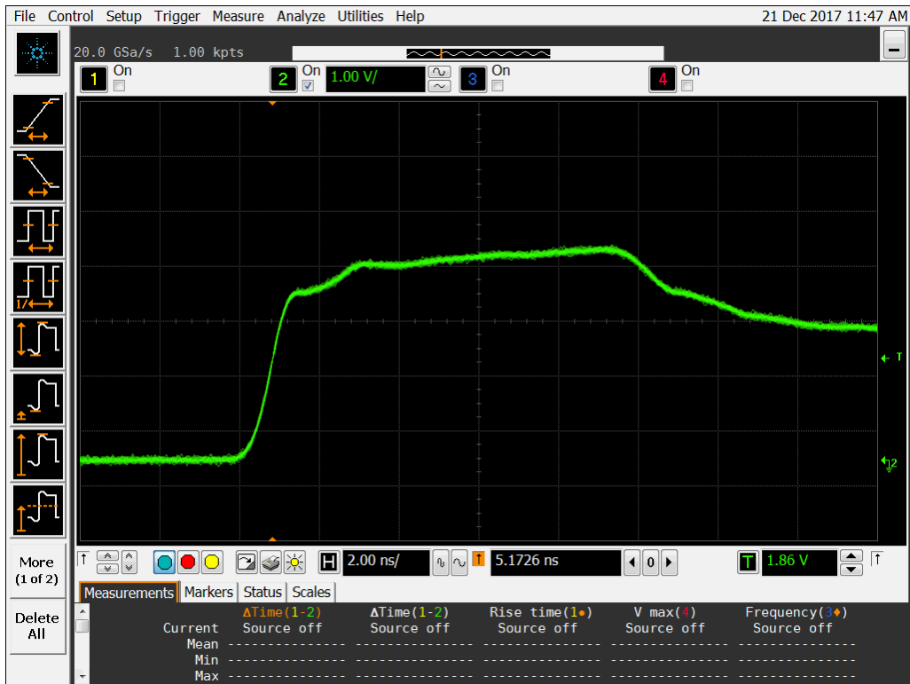
Figure 13b DUT 11021 Post-Annealing Rising Edge.
