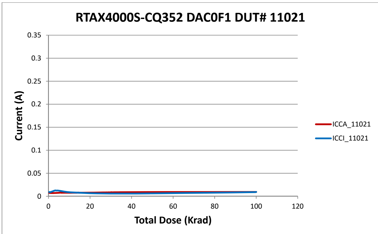
Figure 7 DUT 11021 Influx ICCI and ICCA
