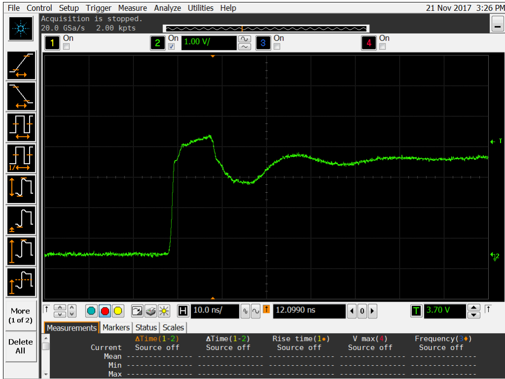
Figure 9a DUT 11052 Pre-irradiation Rising Edge.
