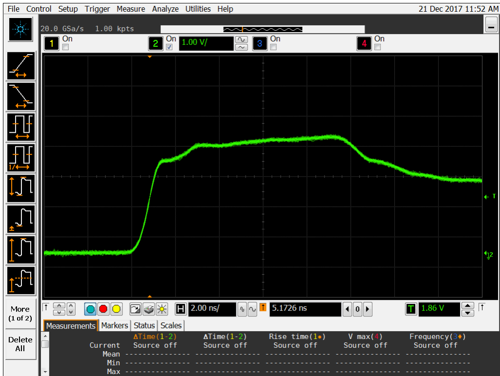
Figure 11b DUT 11030 Post-Annealing Rising Edge.
