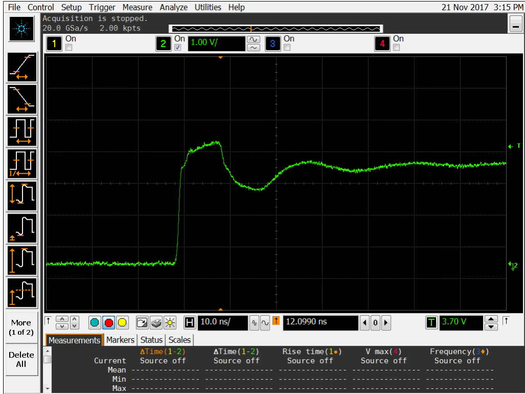
Figure 13a DUT 11021 Pre-Irradiation Rising Edge.
