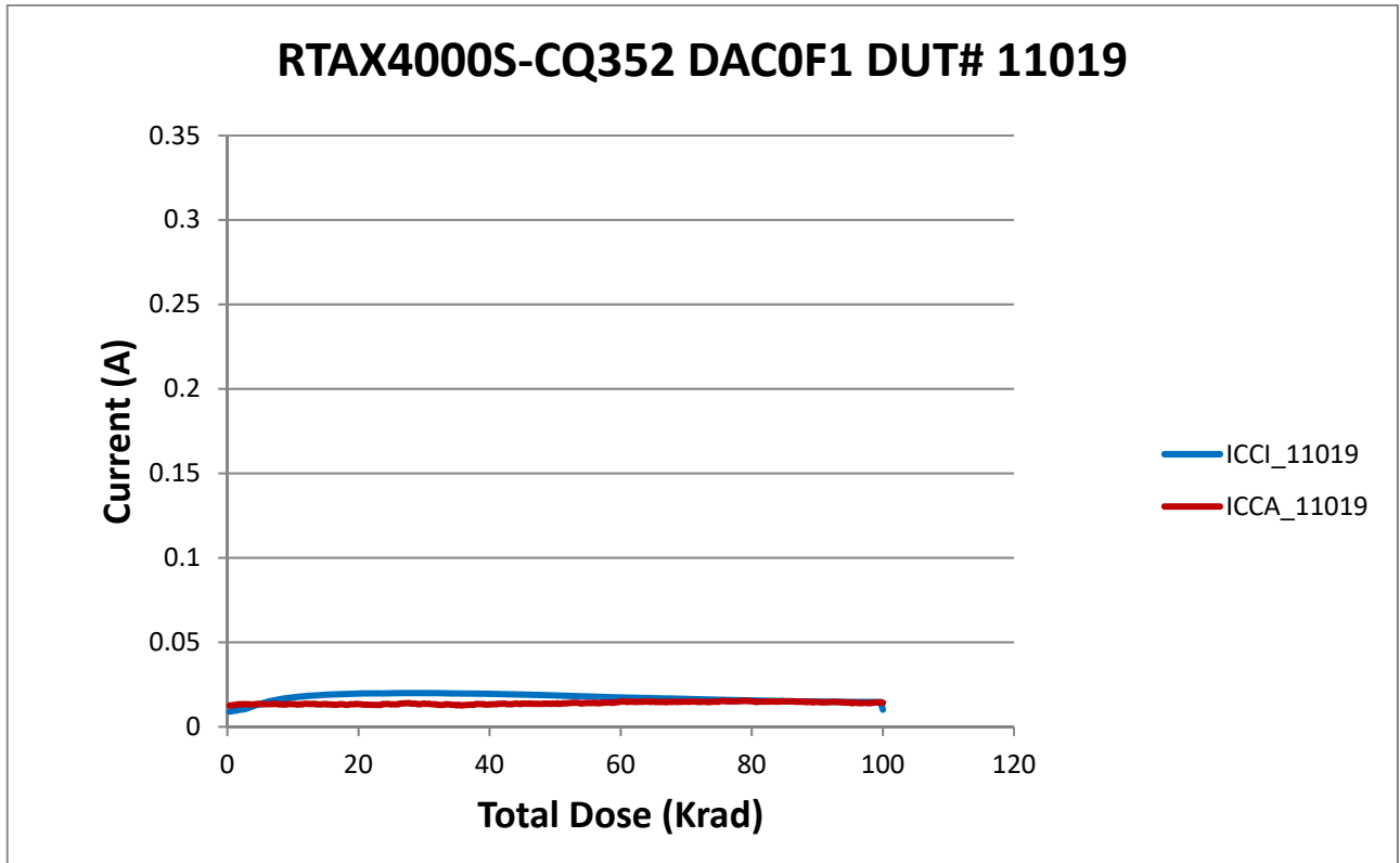
Figure 6 DUT 11019 Influx ICCI and ICCA
