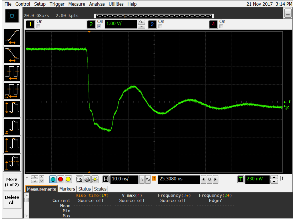
Figure 19a DUT 11021 Pre-Irradiation Falling Edge.
