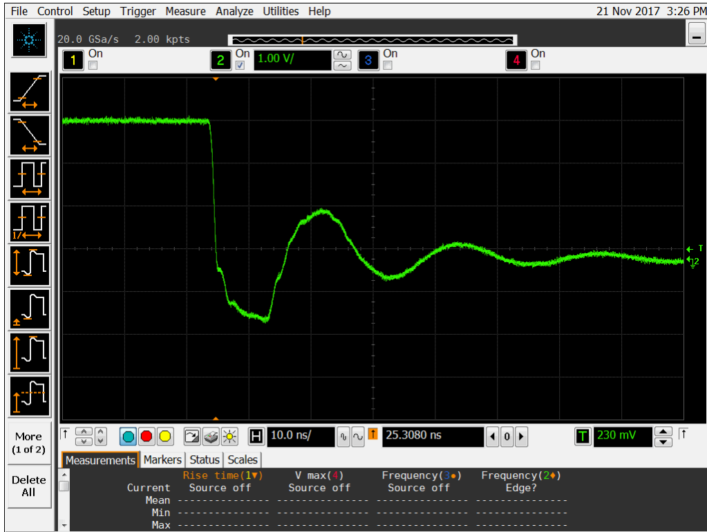
Figure 15a DUT 11052 Pre-Irradiation Falling Edge.
