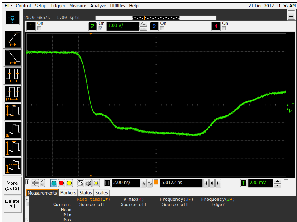
Figure 14b DUT 11044 Post-Annealing Falling Edge.
