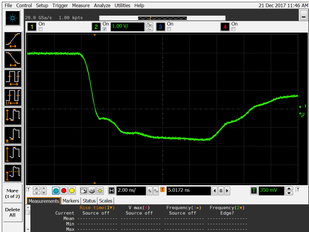
Figure 19b DUT 11021 Post-Annealing Falling Edge.
