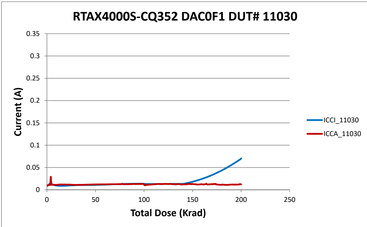
Figure 5 DUT 11030 Influx ICCI and ICCA
