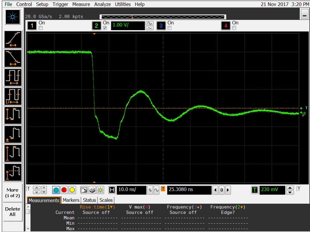
Figure 17a DUT 11030 Pre-Irradiation Falling Edge.
