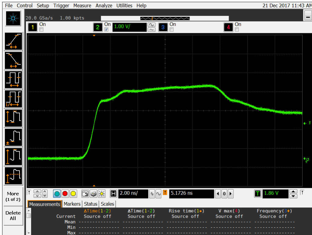
Figure 12b DUT 11019 Post-Annealing Rising Edge.
