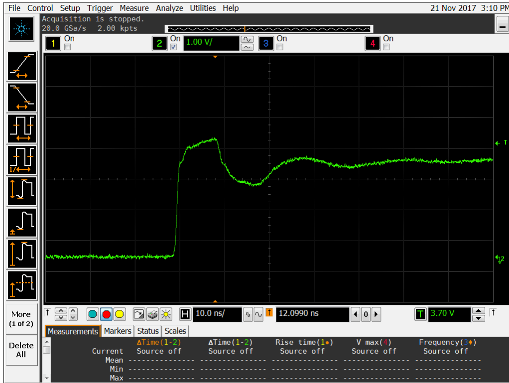
Figure 12a DUT 11019 Pre-Irradiation Rising Edge.
