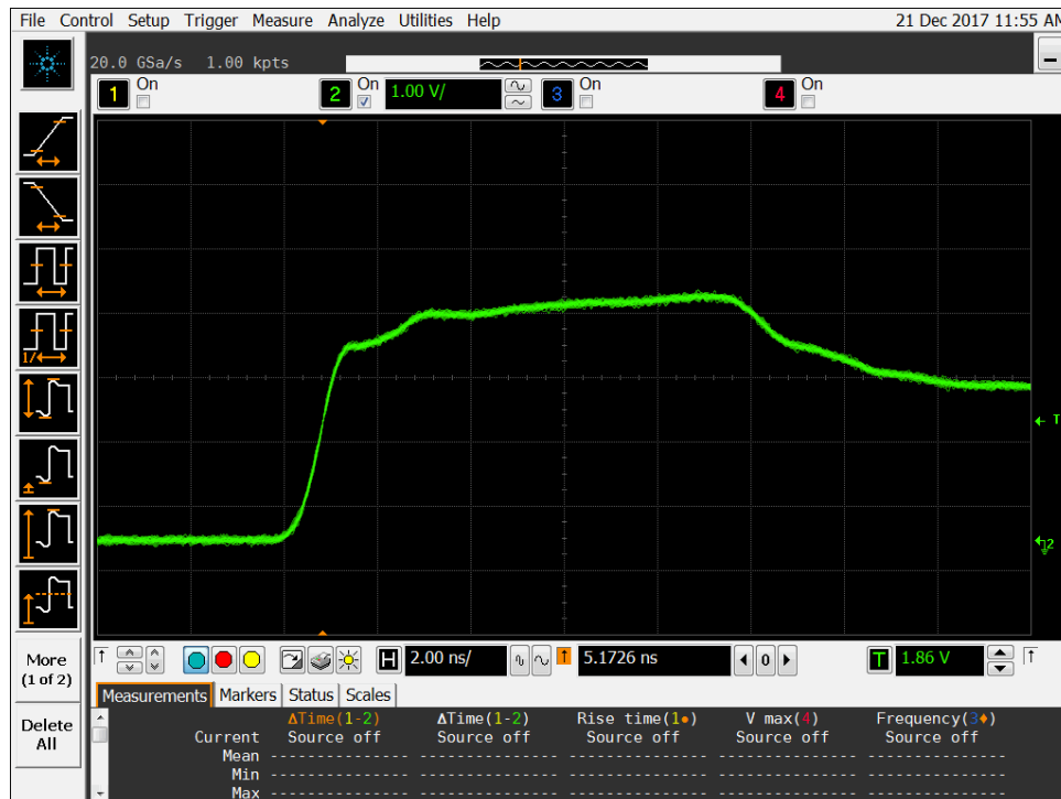
Figure 8b DUT 11044 Post-Annealing Rising Edge.
