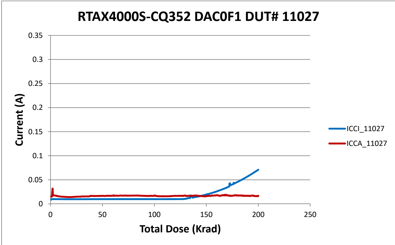
Figure 4 DUT 11027 Influx ICCI and ICCA
