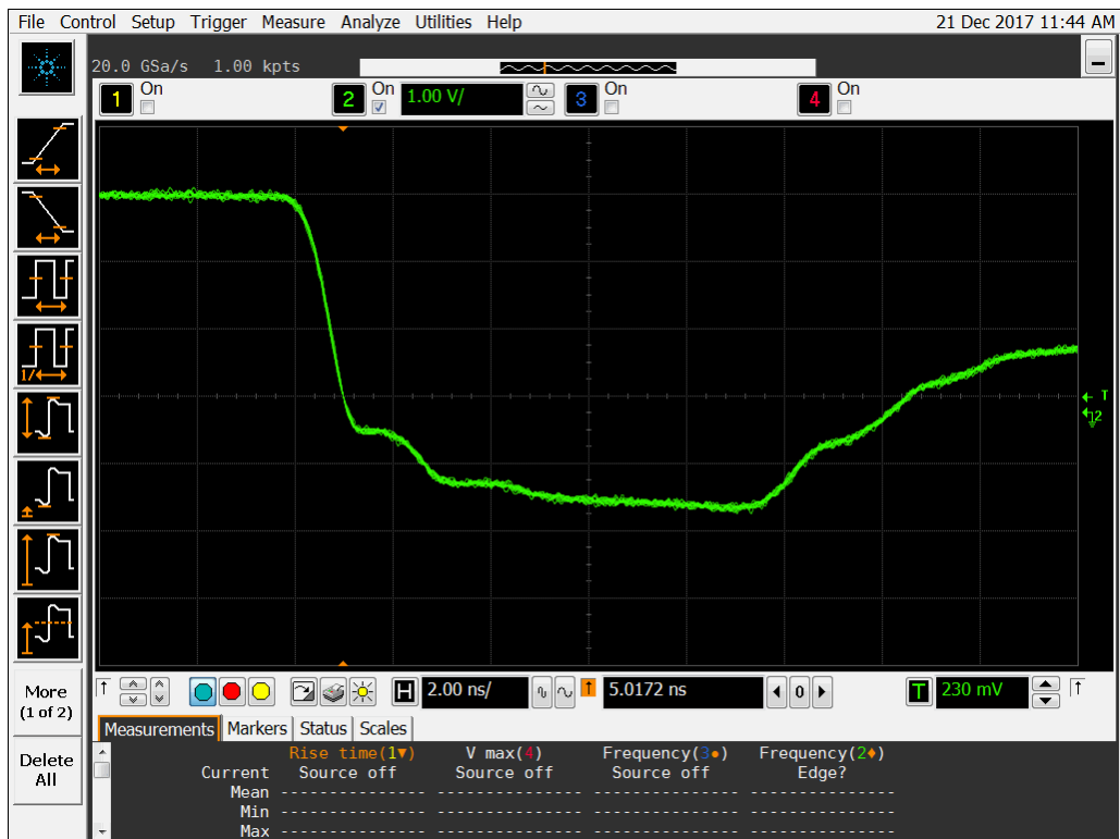
Figure 18b DUT 11019 Post-Annealing Falling Edge.
