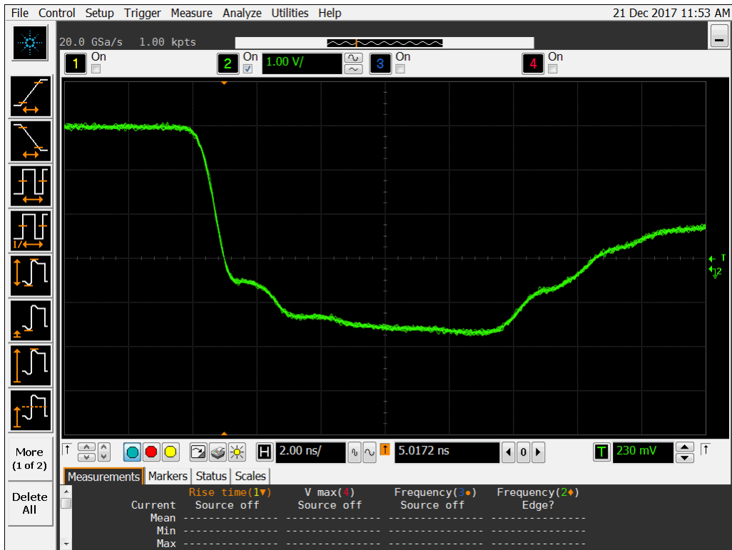
Figure 17b DUT 11030 Post-Annealing Falling Edge.
