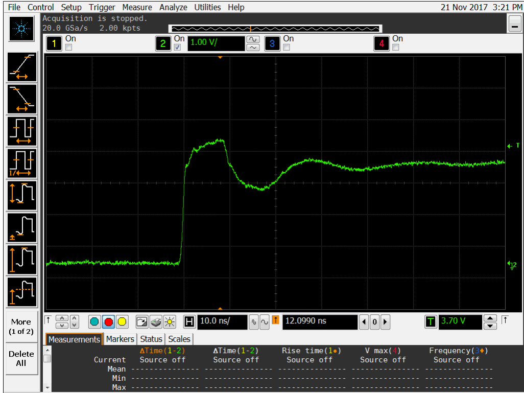
Figure 11a DUT 11030 Pre-Irradiation Rising Edge.
