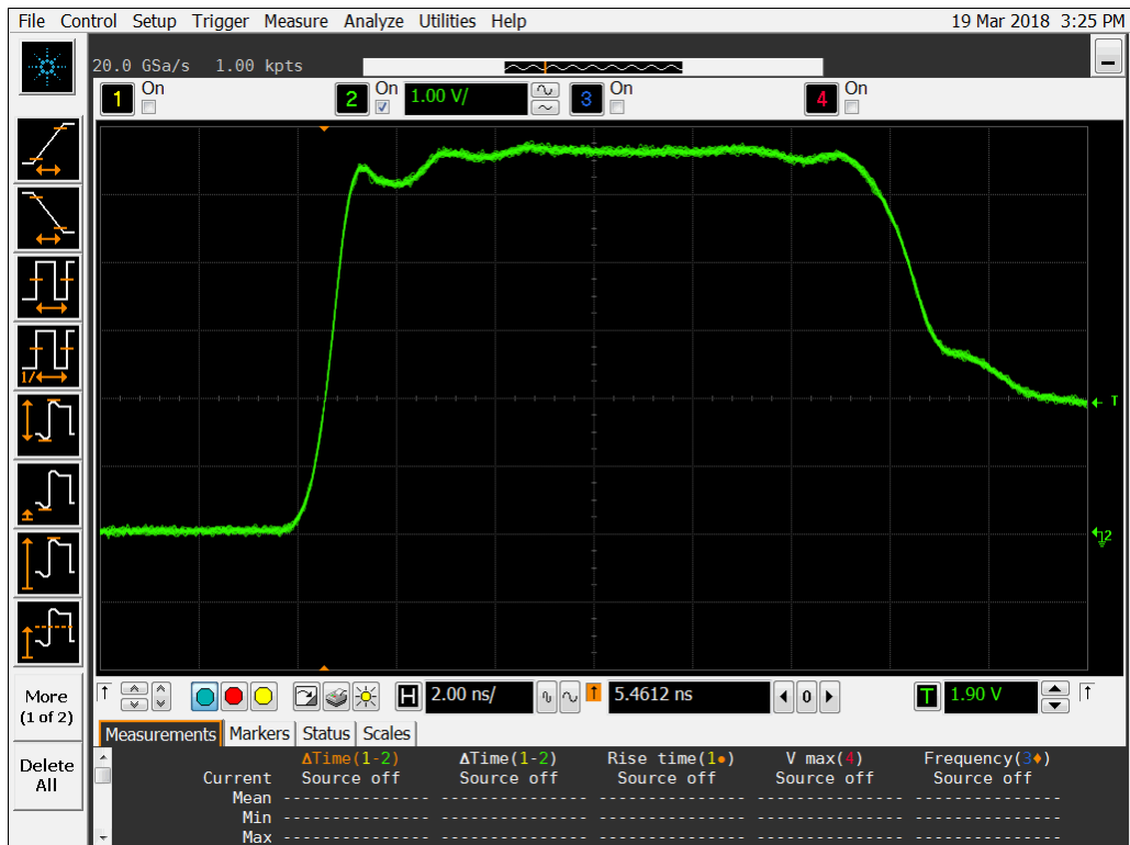
Figure 13b DUT 15877 Post-Annealing Rising Edge
