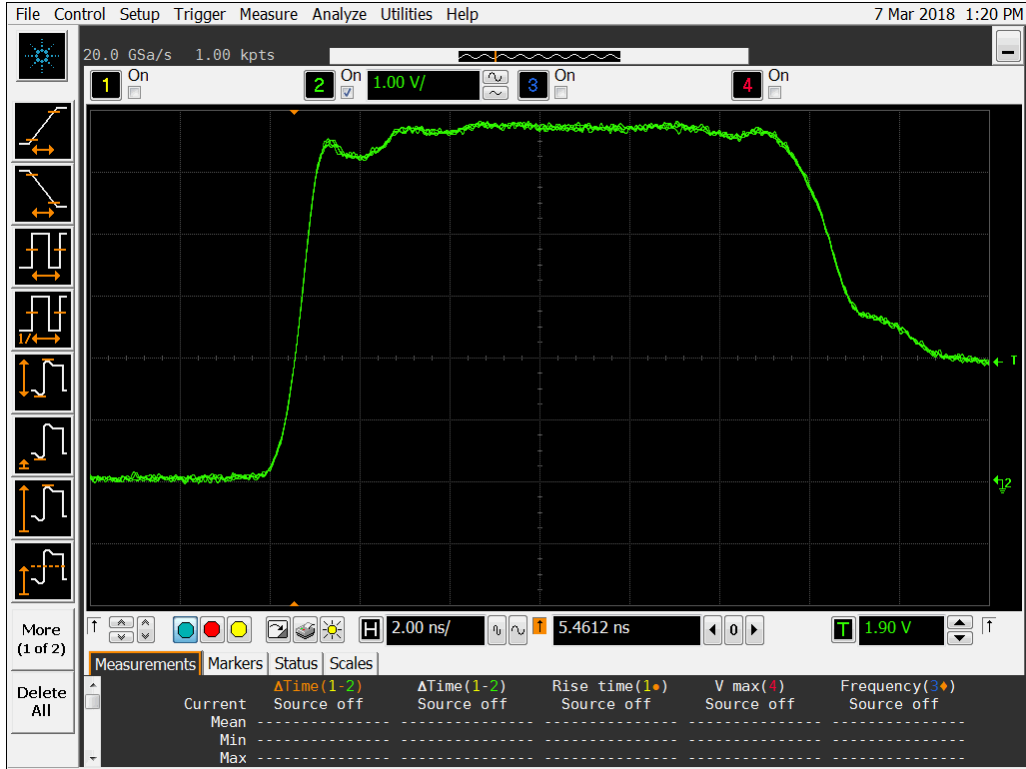
Figure 12a DUT 15913 Pre-Irradiation Rising Edge
