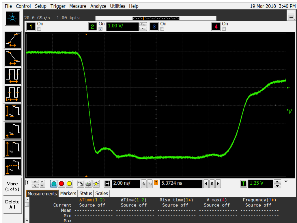
Figure 15b DUT 15914 Post-Annealing Falling Edge
