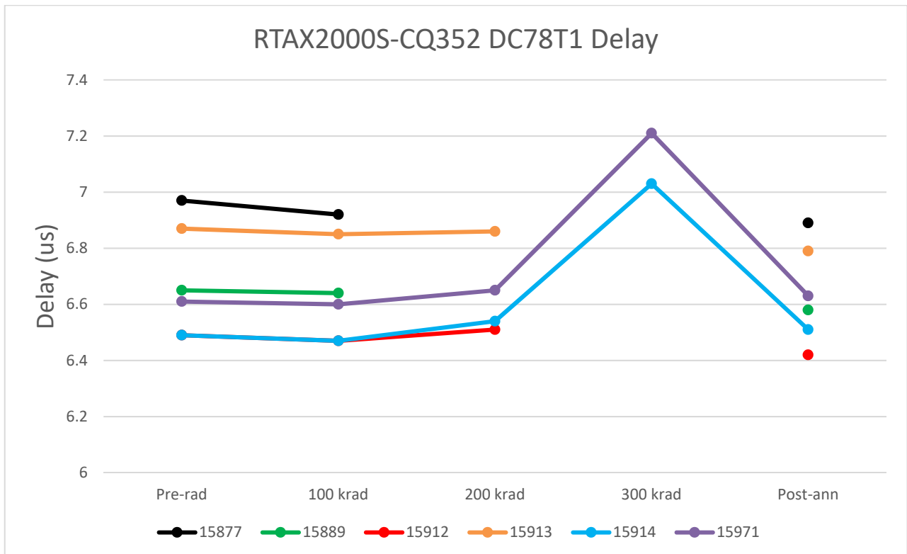
Figure 8 In-Situ Propagation Delay versus Total Dose
