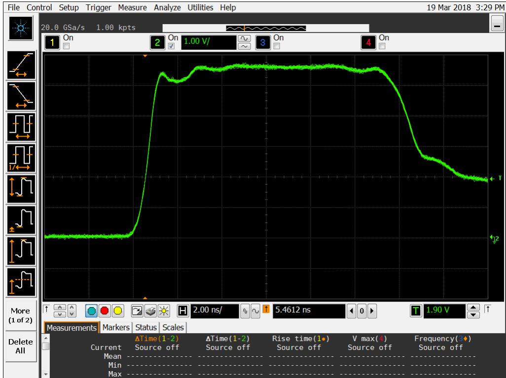
Figure 14b DUT 15889 Post-Annealing Rising Edge
