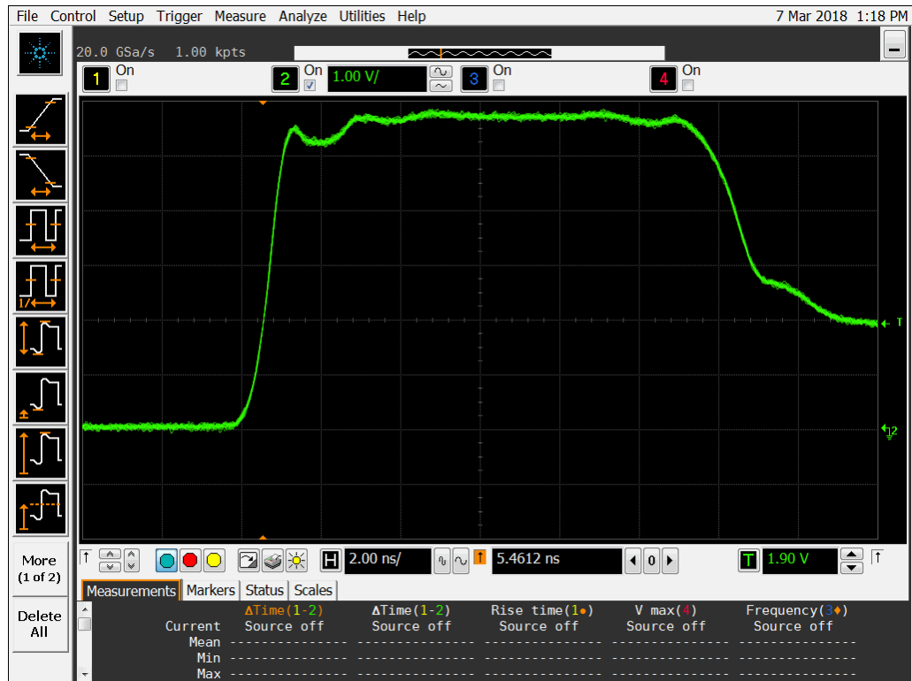
Figure 11a DUT 15912 Pre-Radiation Rising Edge
