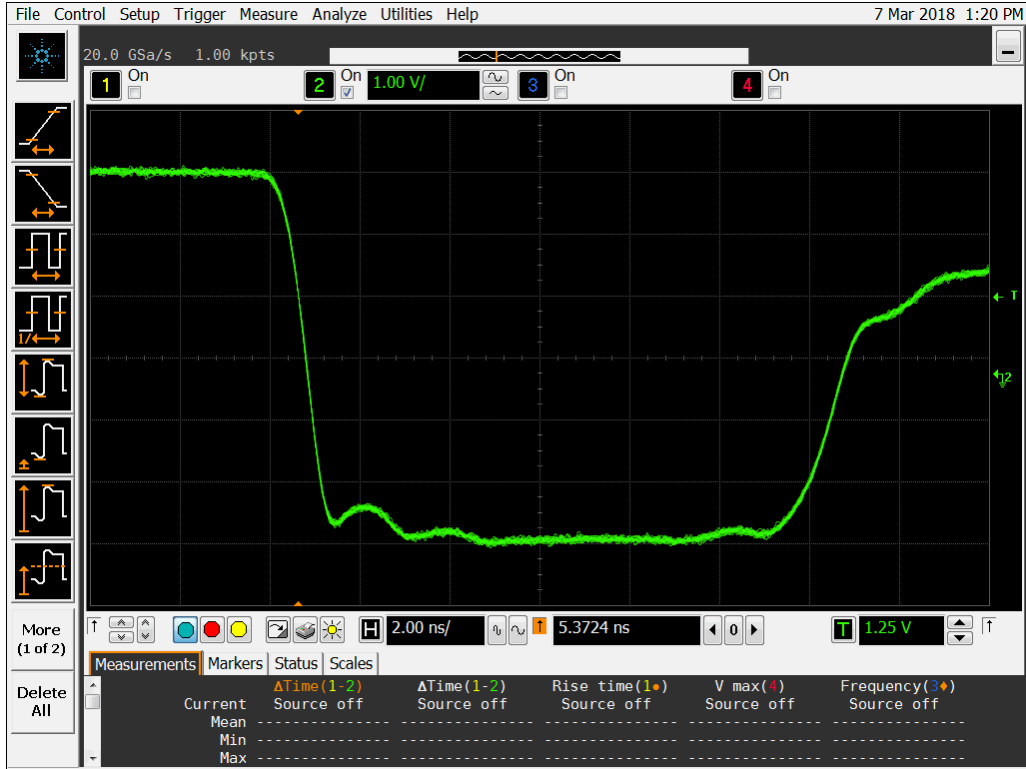
Figure 18a DUT 15913 Pre-Irradiation Falling Edge
