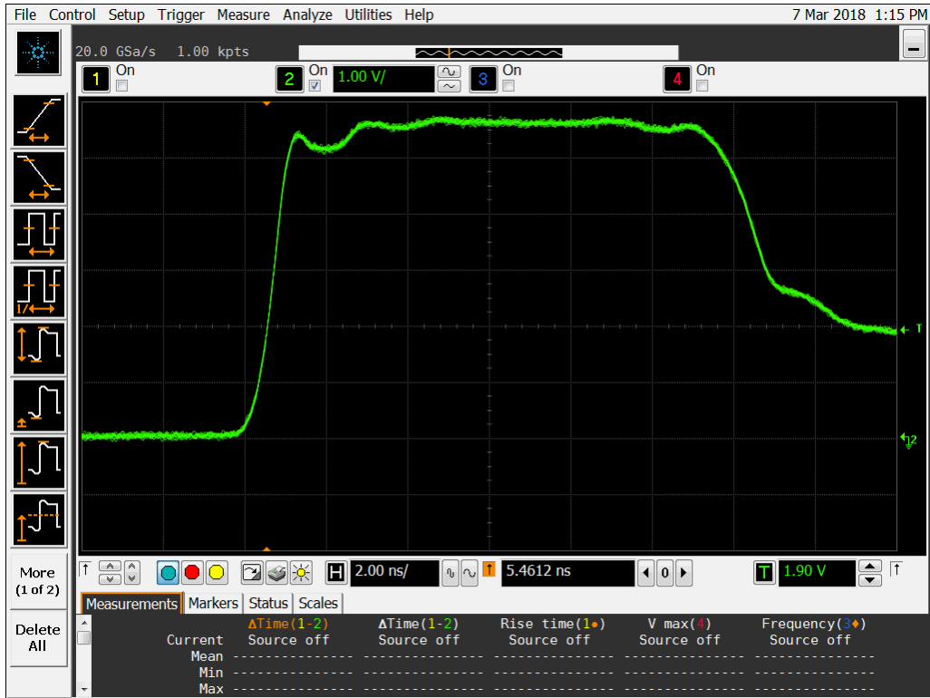
Figure 14a DUT 15889 Pre-Irradiation Rising Edge
