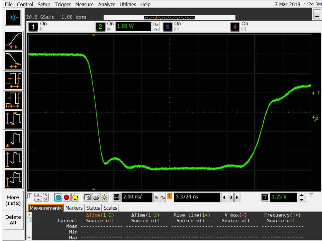
Figure 16a DUT 15971 Pre-Irradiation Falling Edge
