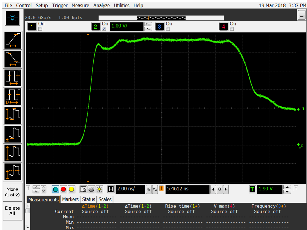
Figure 12b DUT 15913 Post-Annealing Rising Edge
