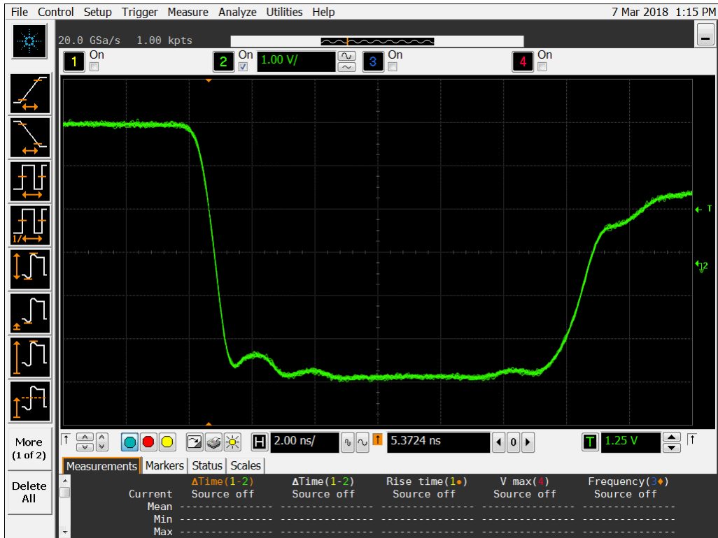
Figure 20a DUT 15889 Pre-Irradiation Falling Edge
