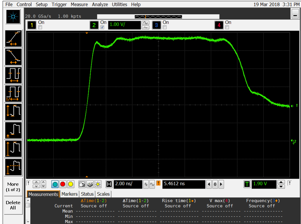
Figure 11b DUT 15912 Post-Annealing Rising edge
