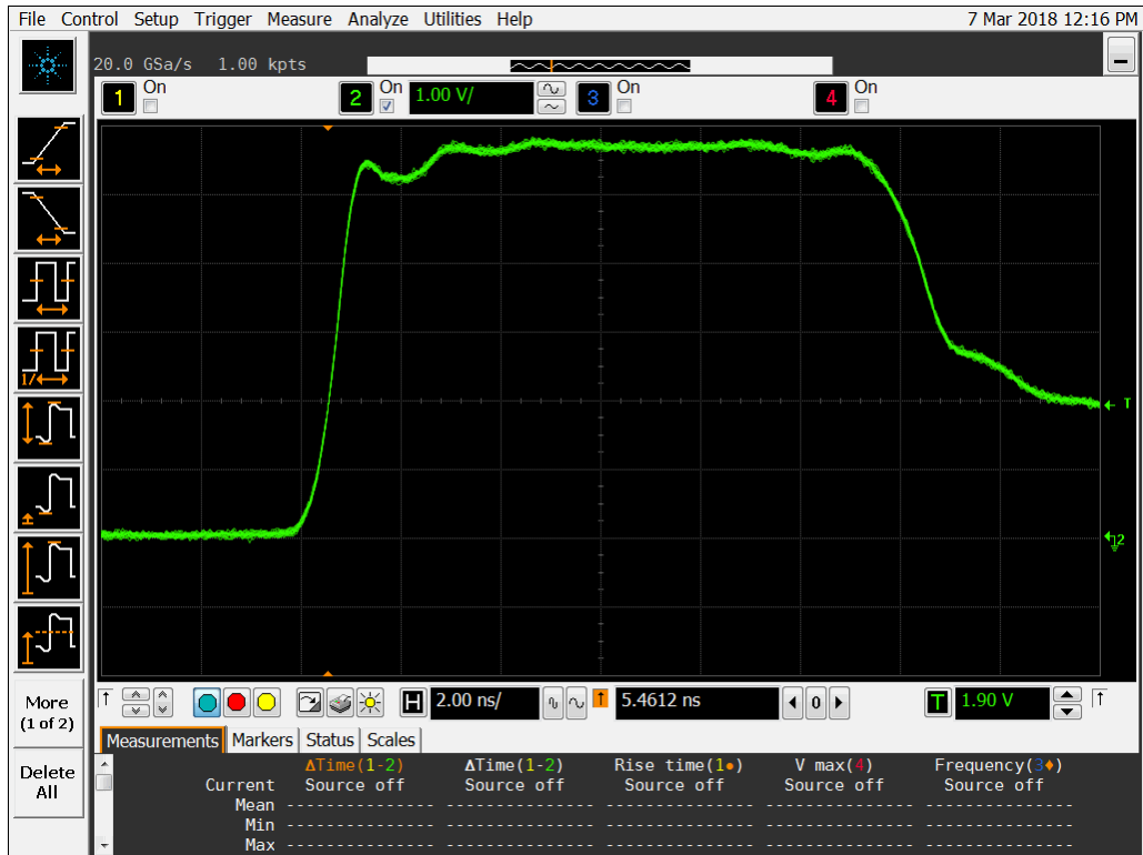
Figure 13a DUT 15877 Pre-Irradiation Rising Edge
