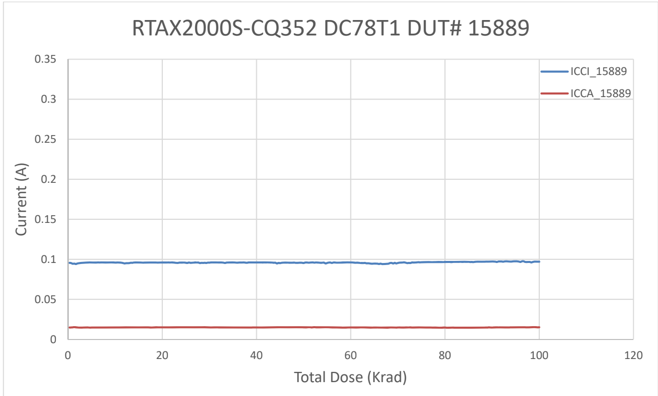
Figure 7 DUT 15889 Influx ICCA and ICCI
