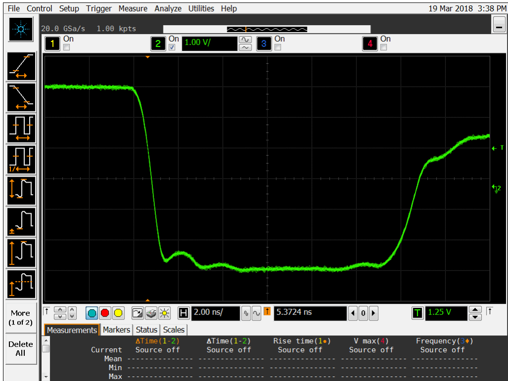
Figure 18b DUT 15913 Post-Annealing Falling Edge
