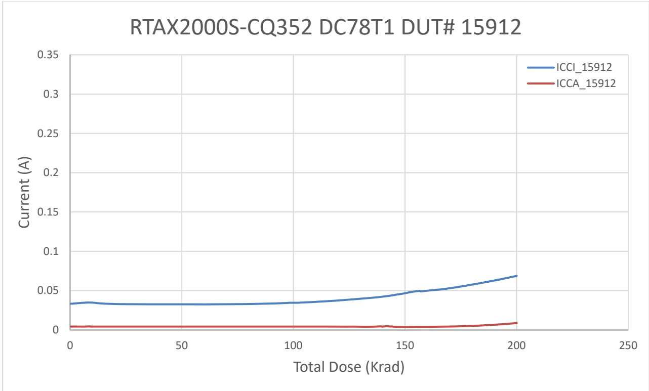
Figure 4 DUT 15912 Influx ICCA and ICCI
