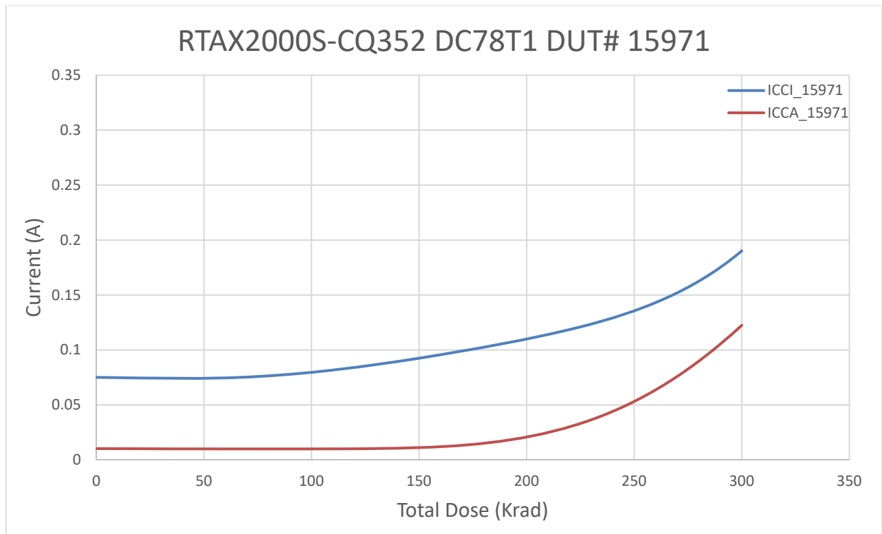
Figure 3 DUT 15971 Influx ICCA and ICCI
