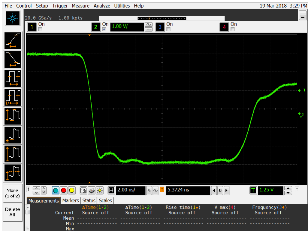
Figure 20b DUT 15889 Post-Annealing Falling Edge
