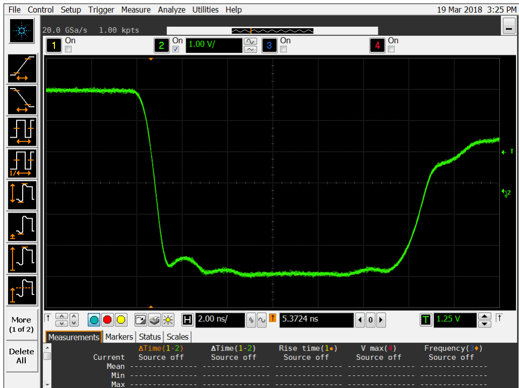
Figure 19b DUT 15877 Post-Annealing Falling Edge
