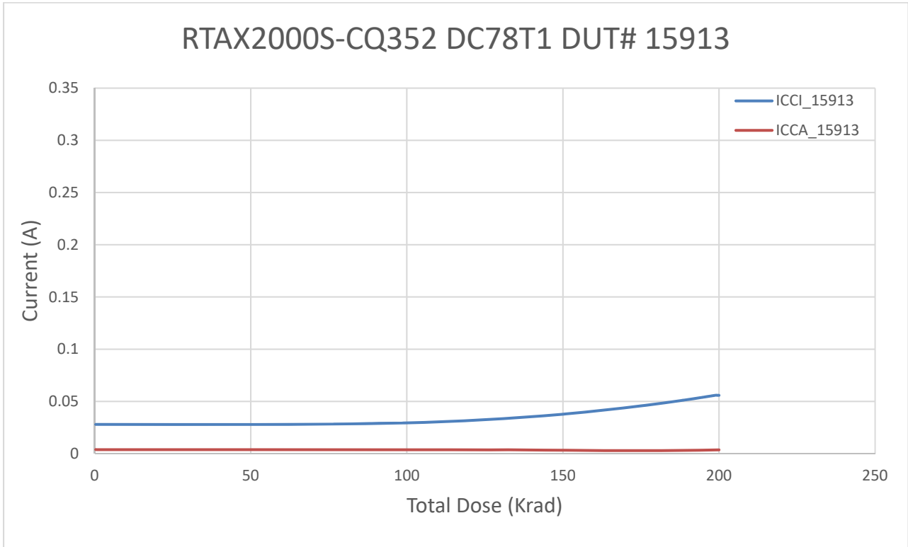
Figure 5 DUT 15913 Influx ICCA and ICCI
