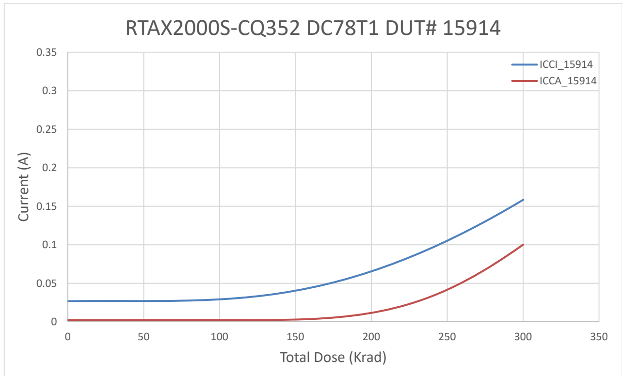
Figure 2 DUT 15914 Influx ICCA and ICCI
