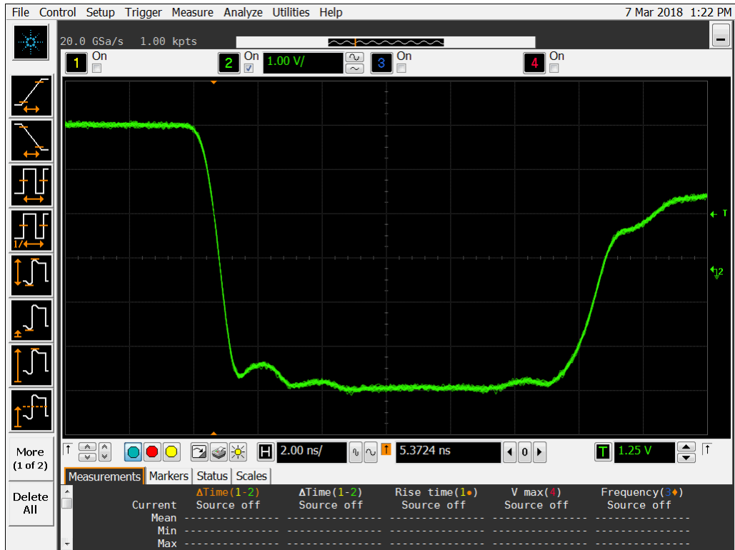
Figure 15a DUT 15914 Pre-Radiation Falling Edge
