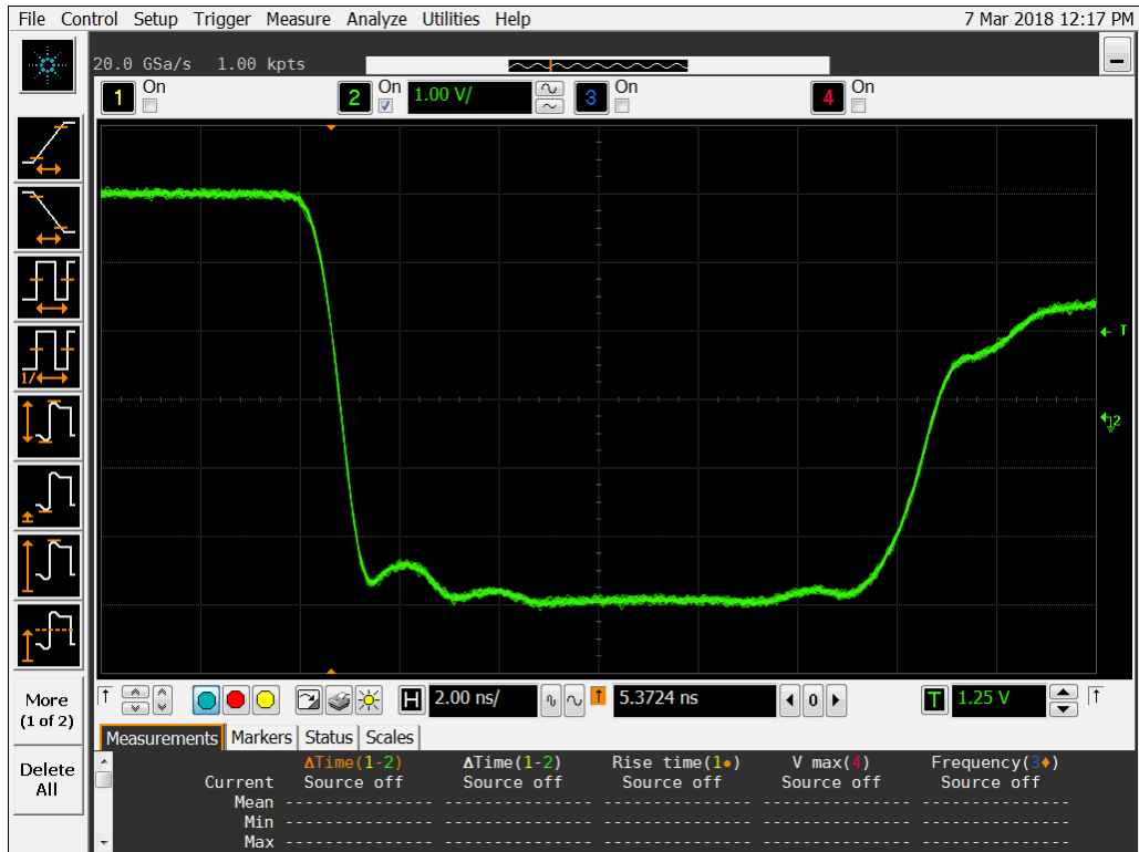
Figure 19a DUT 15877 Pre-Irradiation Falling Edge
