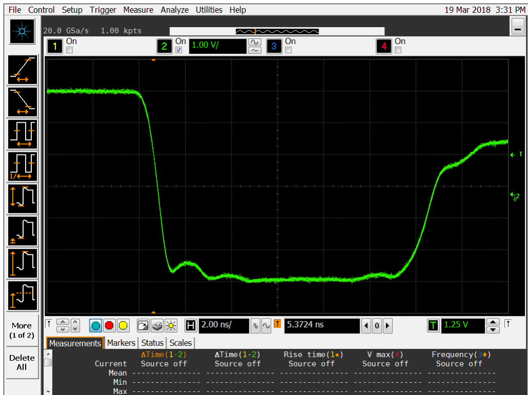
Figure 17b DUT 15912 Post-Annealing Falling Edge
