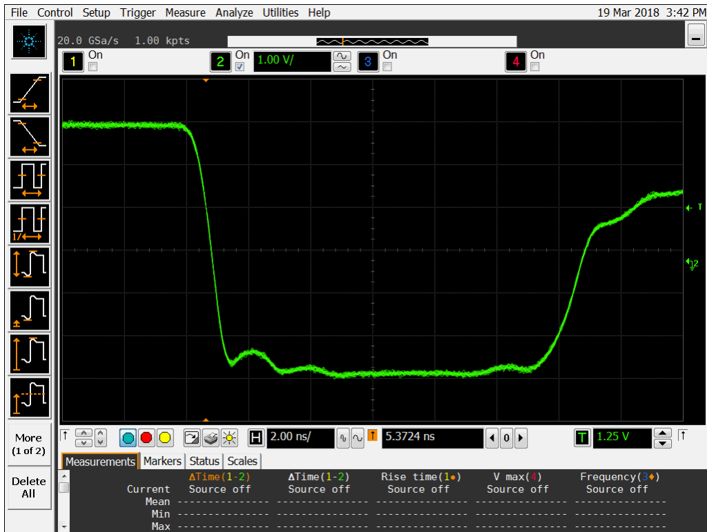
Figure 16b DUT 15971 Post-Annealing Falling Edge
