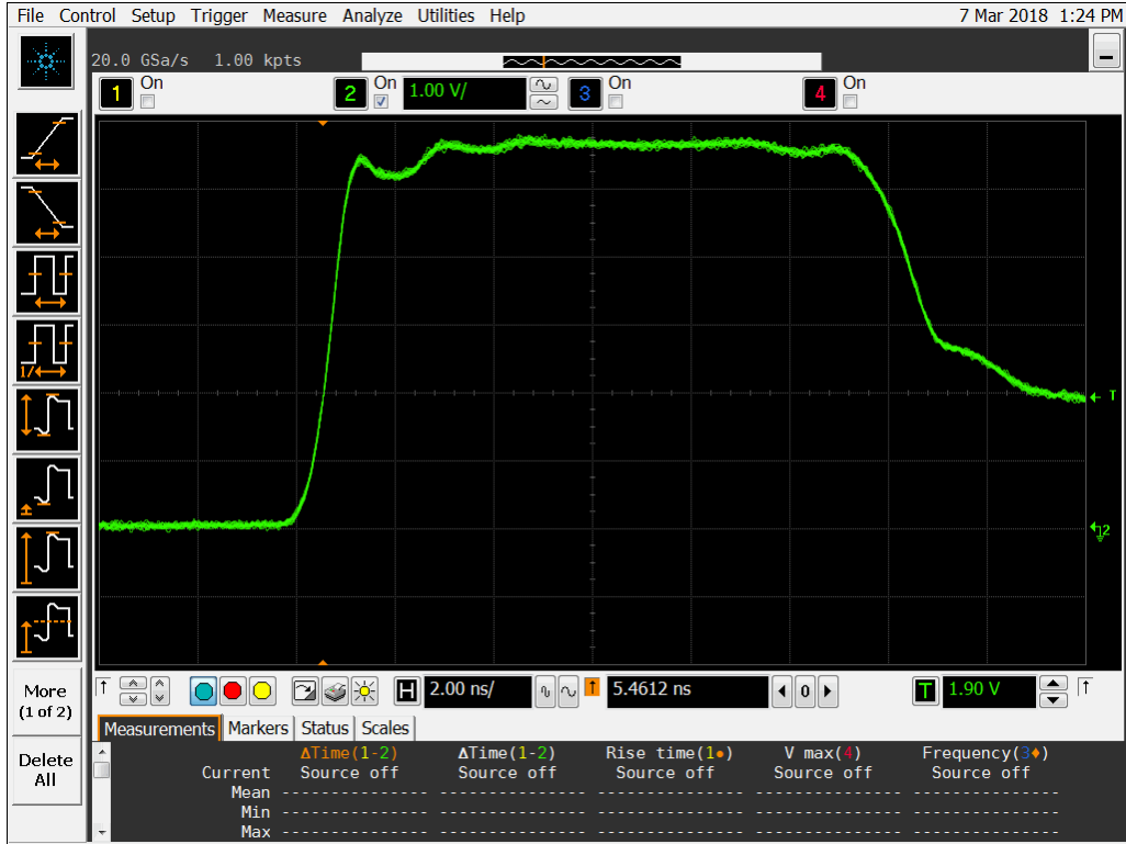
Figure 10a DUT 15971 Pre-Irradiation Rising Edge
