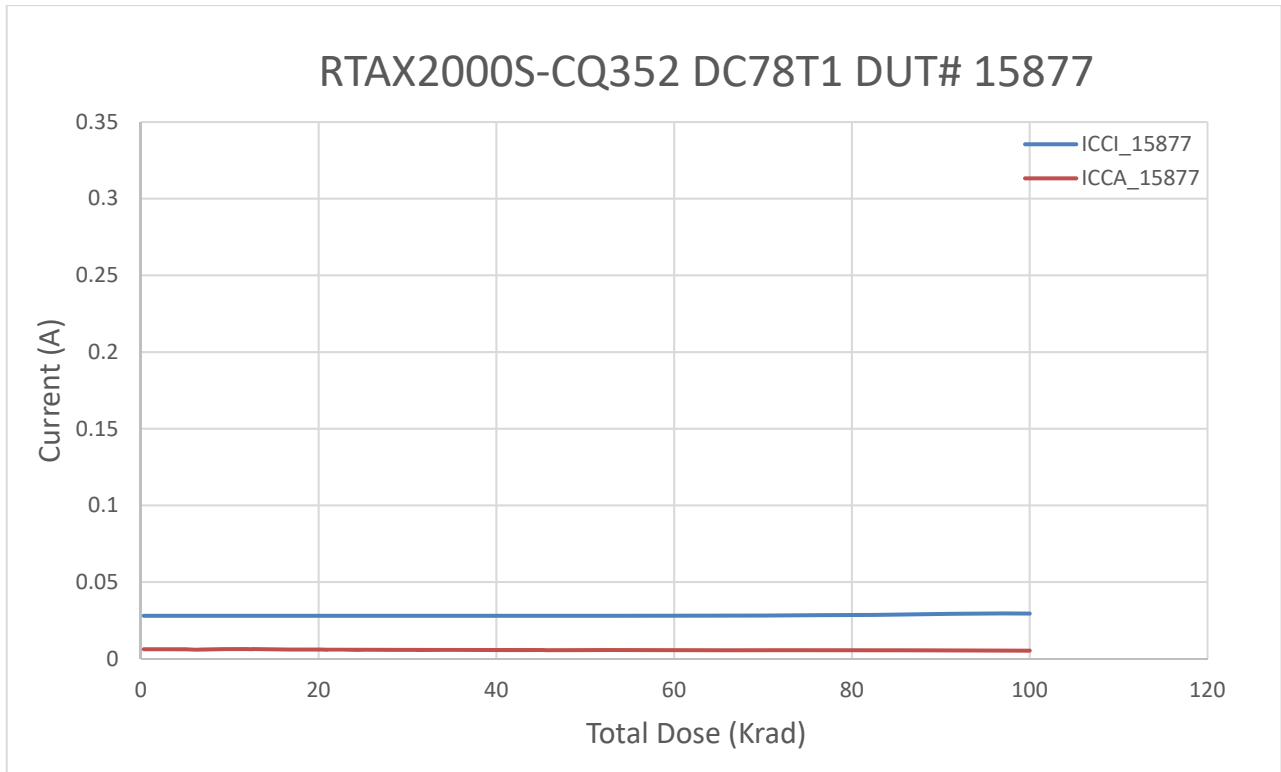
Figure 6 DUT 15877 Influx ICCA and ICCI
