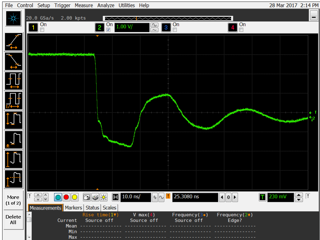
Figure 16a DUT 970 Pre-Irradiation Falling Edge.
