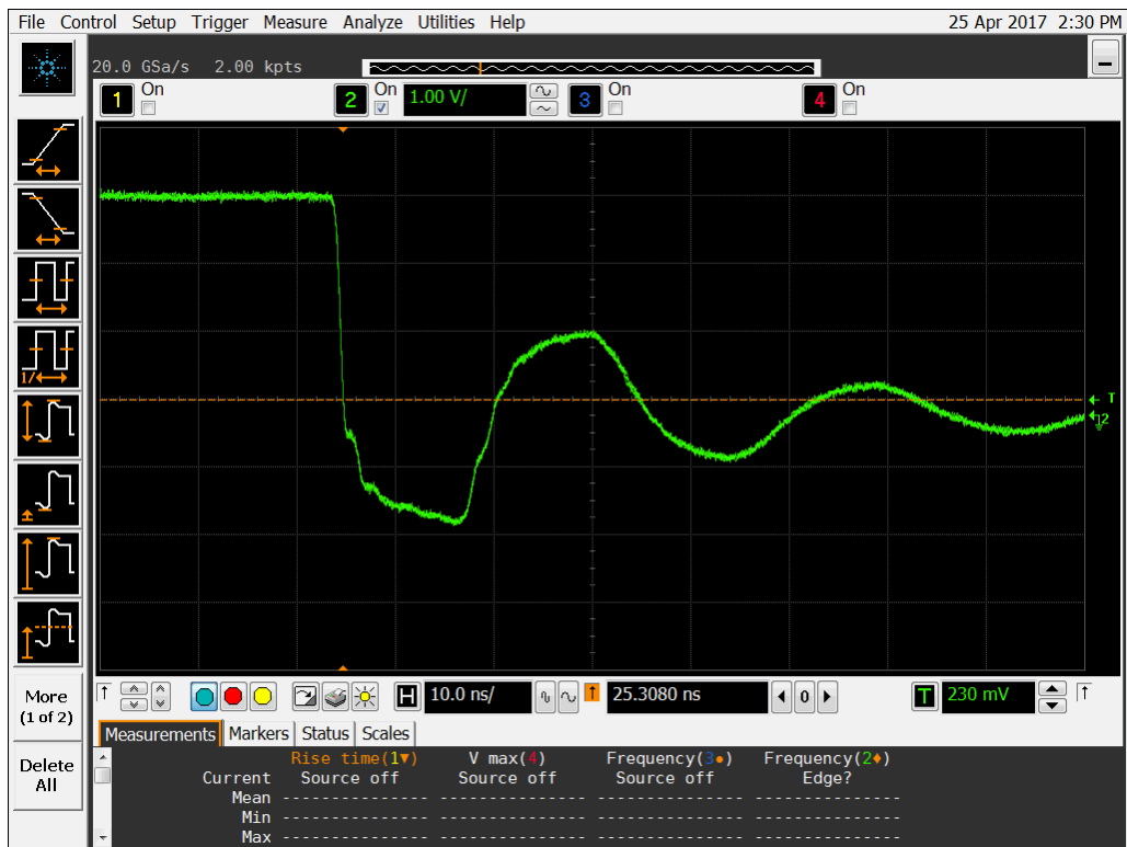
Figure 16b DUT 970 Post-Annealing Falling Edge.
