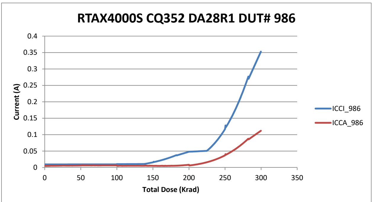
Figure 3 DUT 986 Influx ICCI and ICCA
