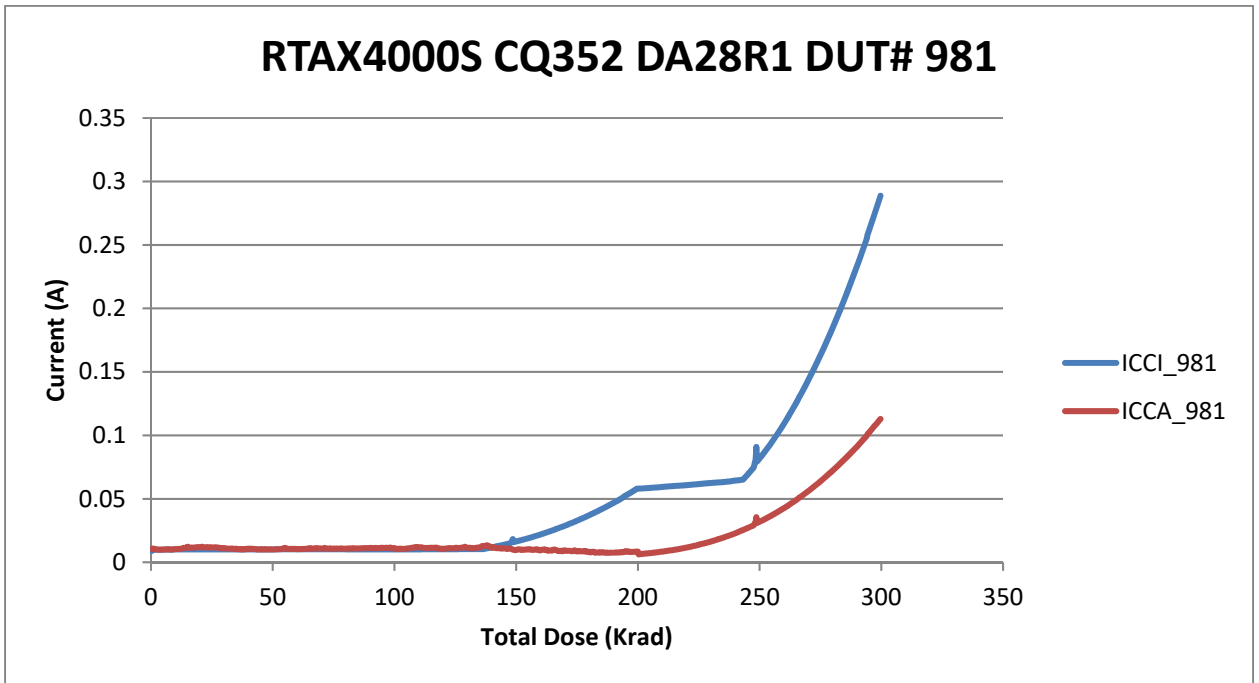
Figure 2 DUT 981 Influx ICCI and ICCA
