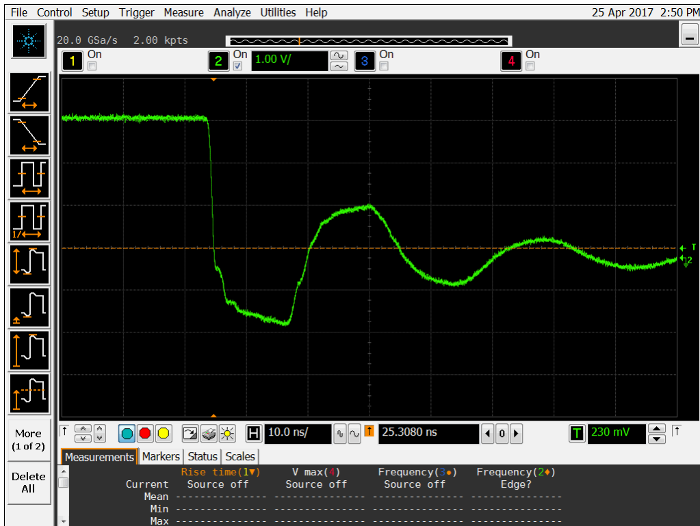
Figure 15b DUT 986 Post-Annealing Falling Edge.
