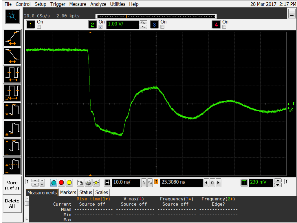
Figure 17a DUT 975 Pre-Irradiation Falling Edge.
