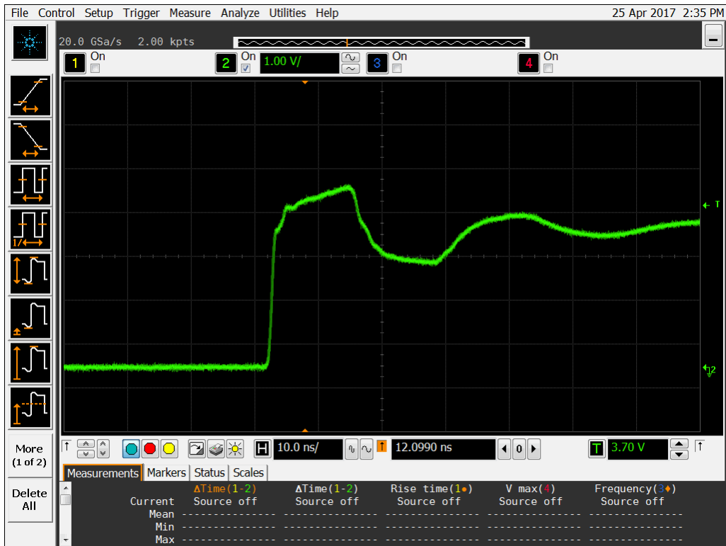
Figure 11b DUT 975 Post-Annealing Rising Edge.
