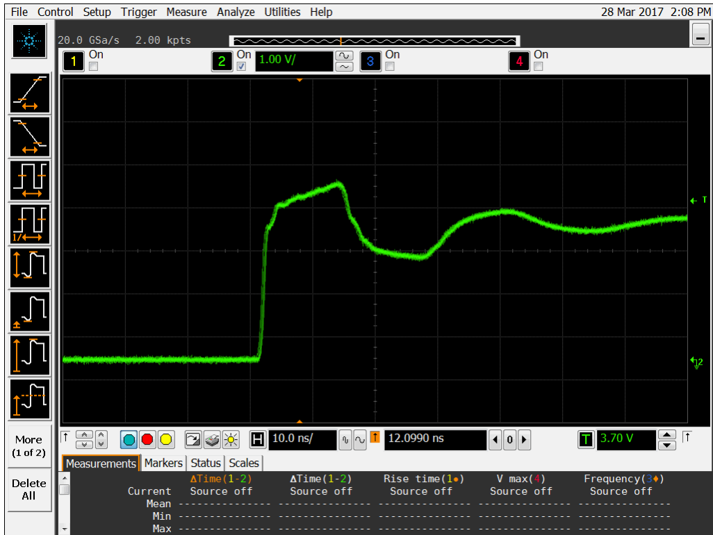
Figure 13a DUT 968 Pre-Irradiation Rising Edge.
