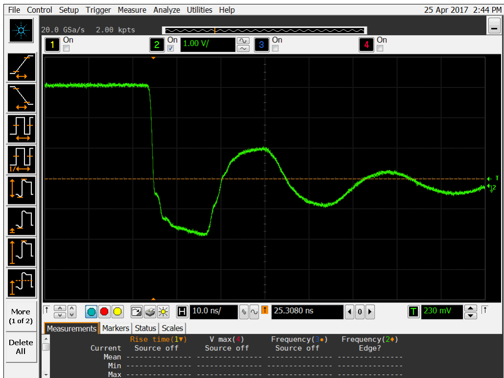
Figure 14b DUT 981 Post-Annealing Falling Edge.
