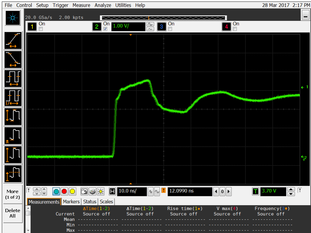
Figure 11a DUT 975 Pre-Irradiation Rising Edge.
