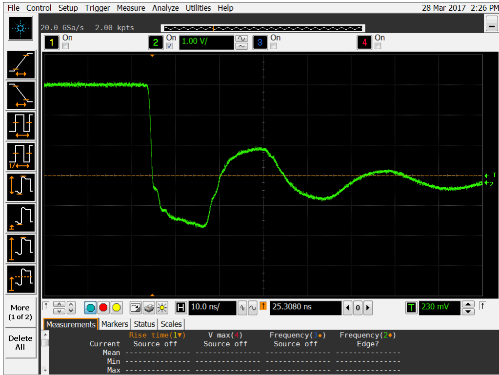
Figure 15a DUT 986 Pre-Irradiation Falling Edge.
