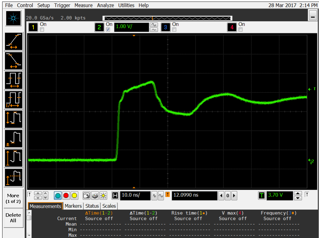
Figure 10a DUT 970 Pre-Irradiation Rising Edge.
