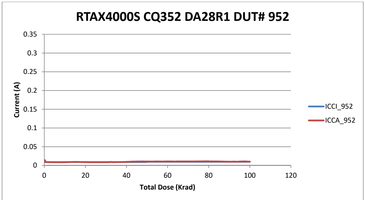
Figure 6 DUT 952 Influx ICCI and ICCA
