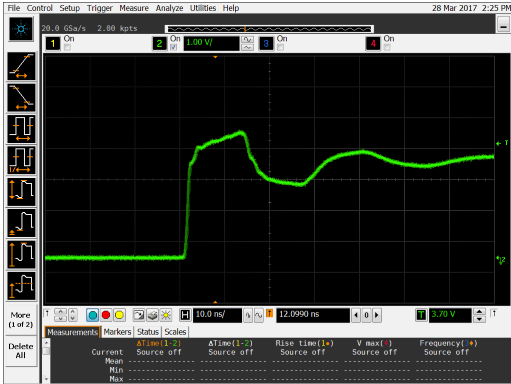
Figure 9a DUT 986 Pre-irradiation Rising Edge.
