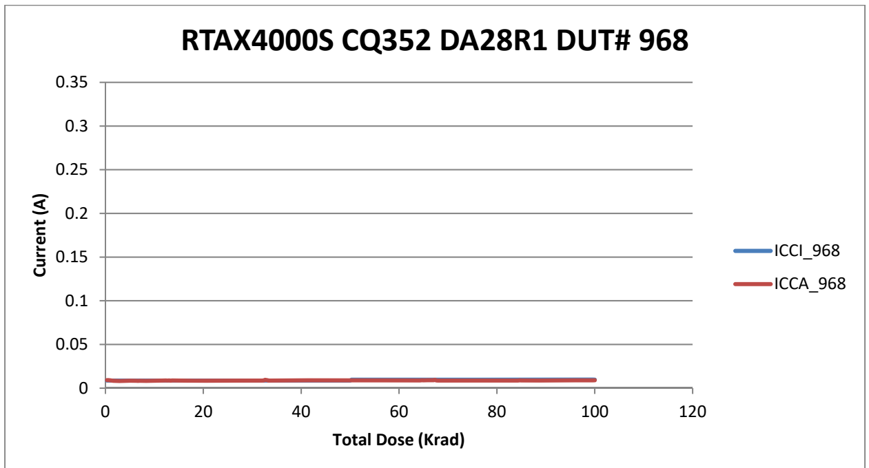
Figure 7 DUT 968 Influx ICCI and ICCA
