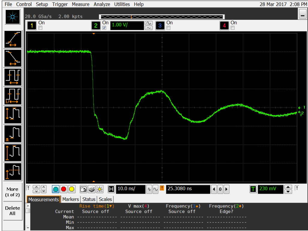
Figure 19a DUT 968 Pre-Irradiation Falling Edge.
