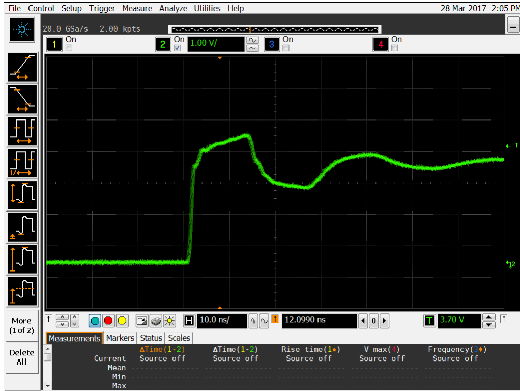
Figure 12a DUT 952 Pre-Irradiation Rising Edge.
