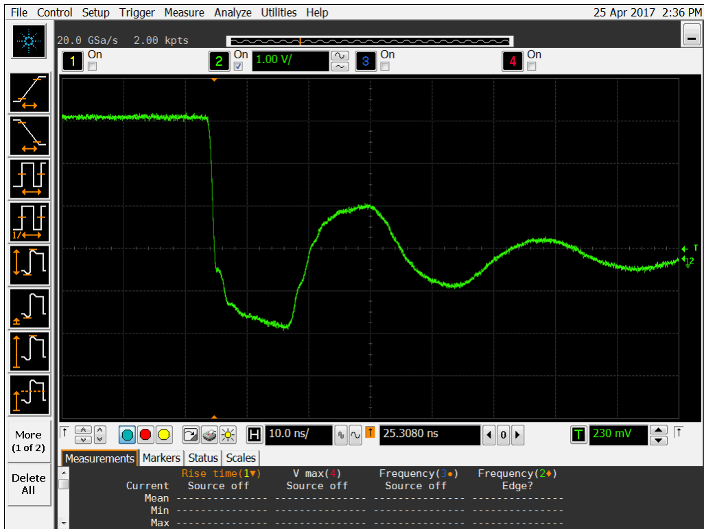
Figure 17b DUT 975 Post-Annealing Falling Edge.
