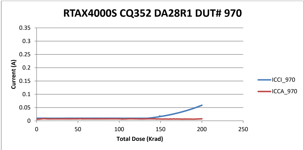
Figure 4 DUT 970 Influx ICCI and ICCA
