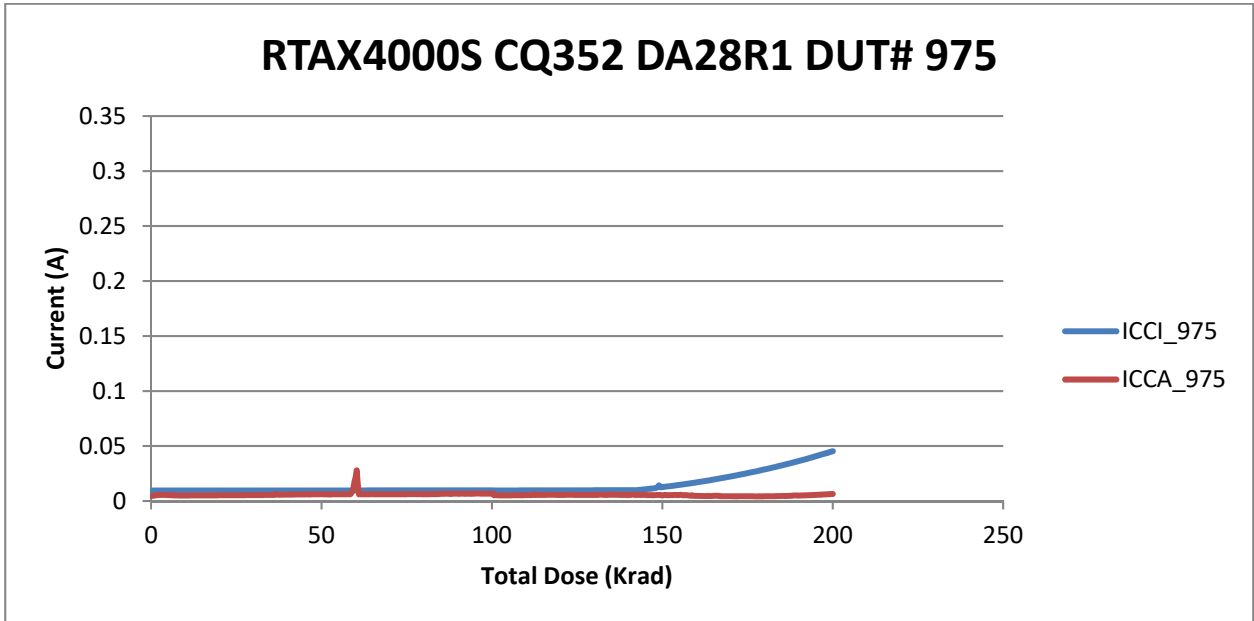
Figure 5 DUT 975 Influx ICCI and ICCA
