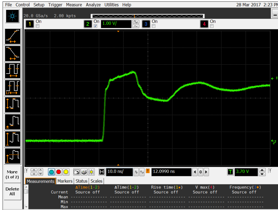
Figure 8a DUT 981 Pre-Irradiation Rising Edge.
