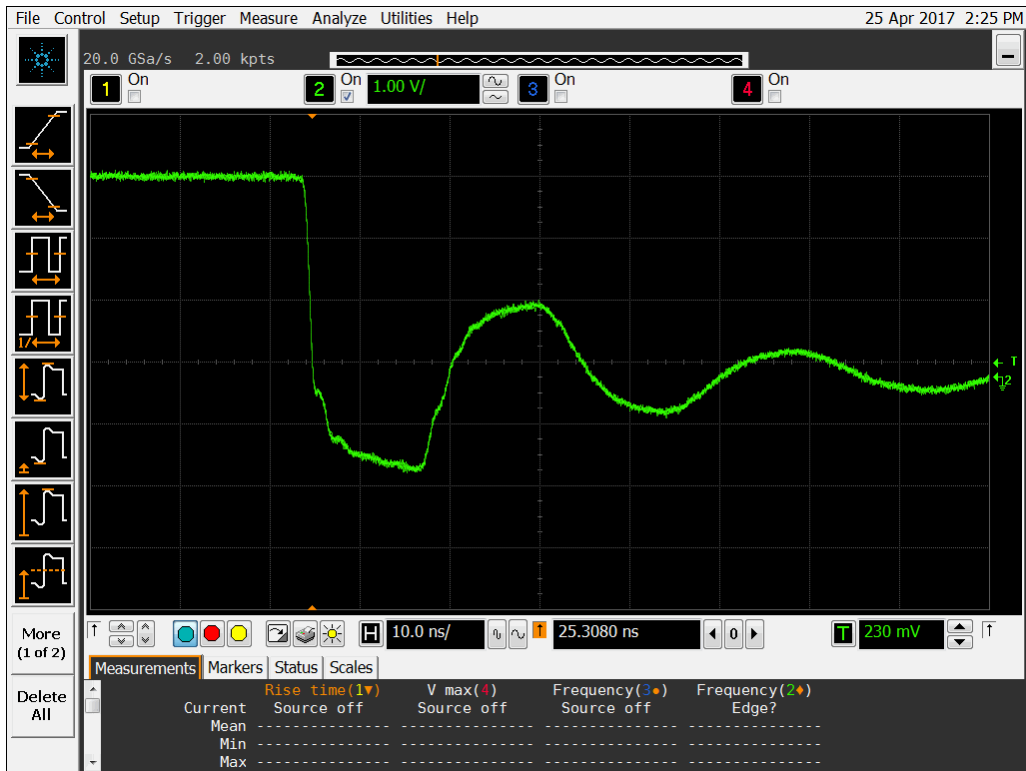
Figure 19b DUT 968 Post-Annealing Falling Edge.
