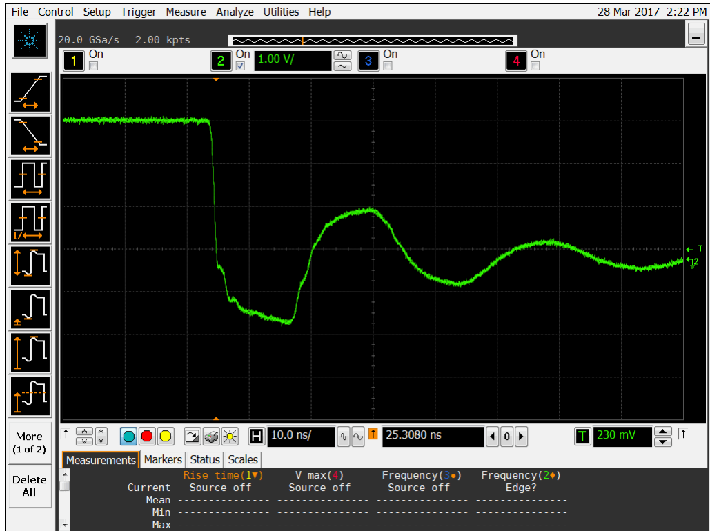
Figure 14a DUT 981 Pre-Irradiation Falling Edge.
