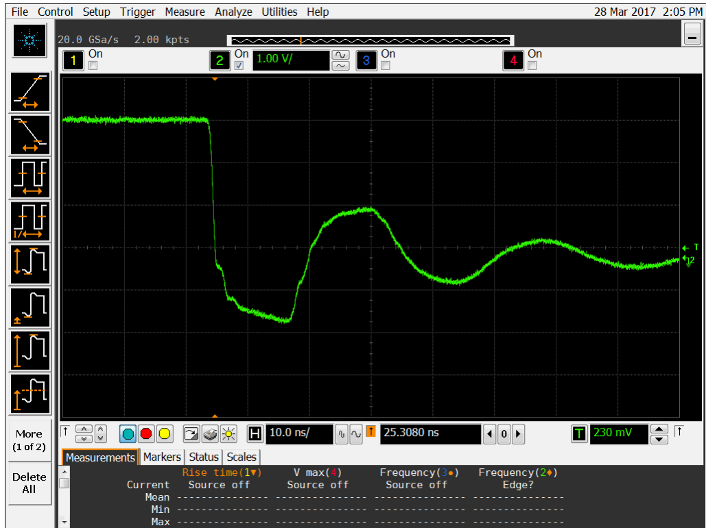
Figure 18a DUT 952 Pre-Irradiation Falling Edge.
