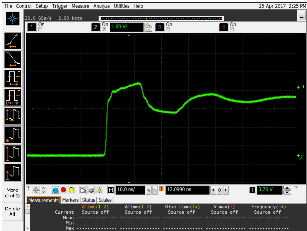
Figure 13b DUT 968 Post-Annealing Rising Edge.
