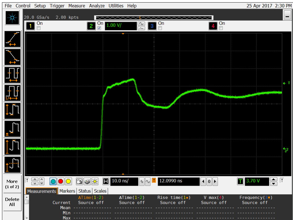
Figure 10b DUT 970 Post-Annealing Rising Edge.
