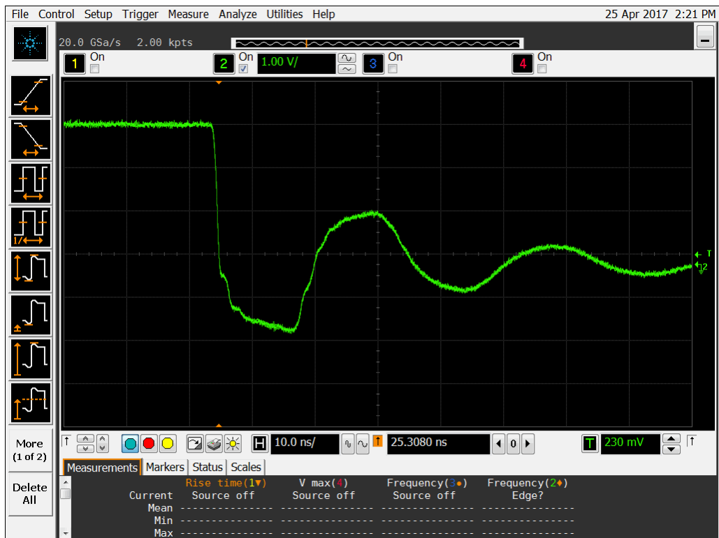
Figure 18b DUT 952 Post-Annealing Falling Edge.
