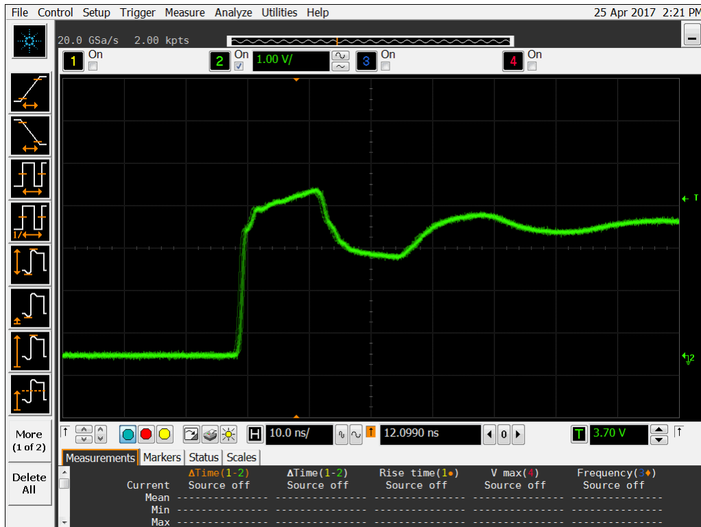
Figure 12b DUT 952 Post-Annealing Rising Edge.
