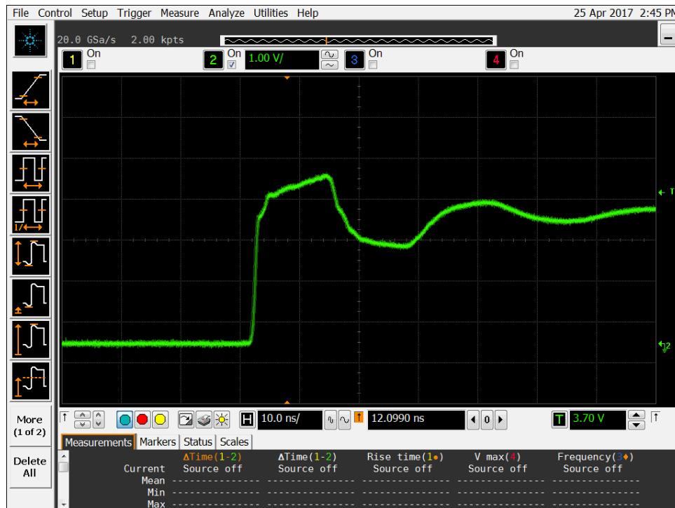
Figure 8b DUT 981 Post-Annealing Rising Edge.
