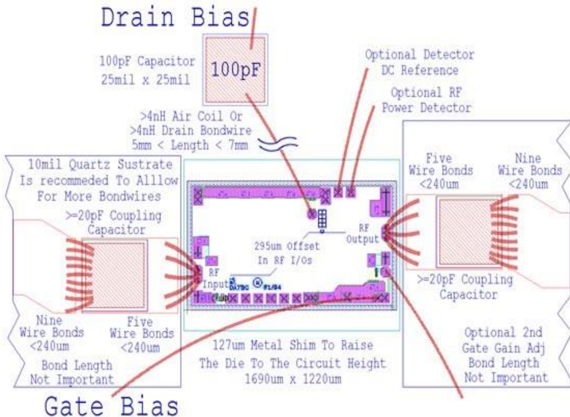
Figure 2. -65GHz bonding diagram
