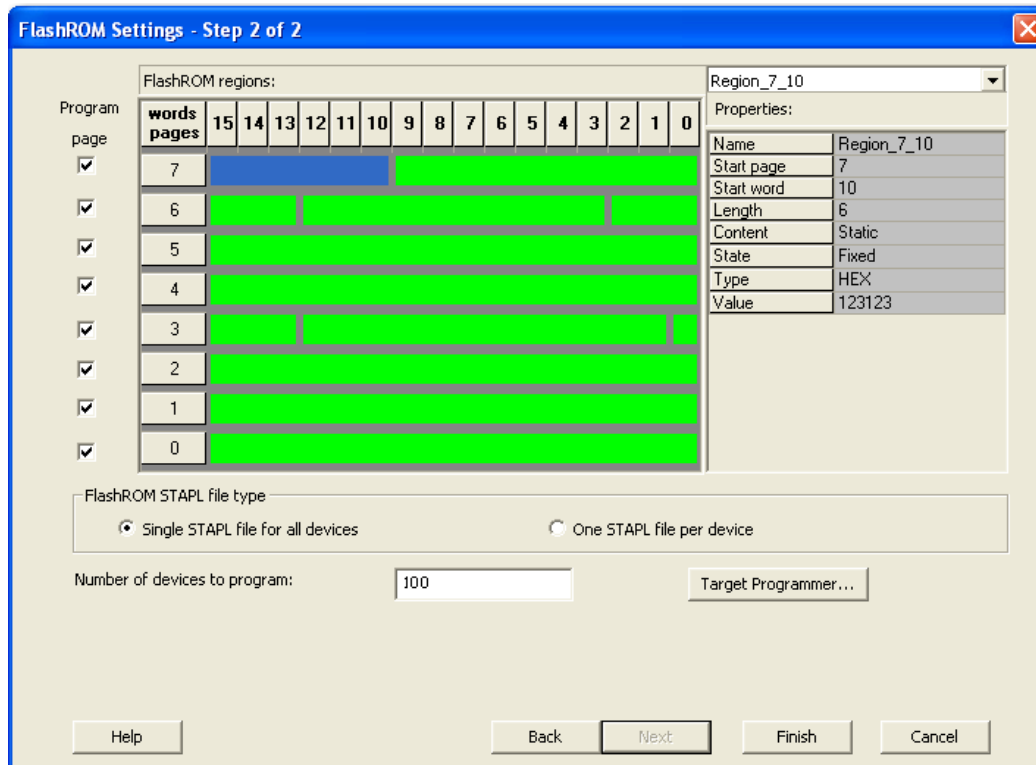
Figure 144 · FlashROM Settings
