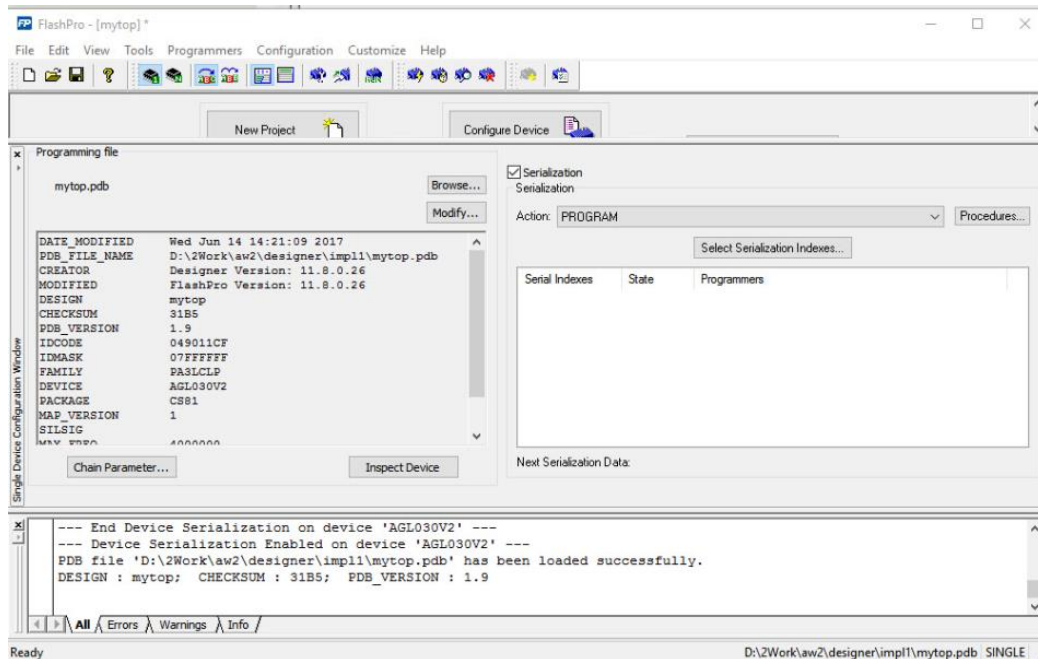
Figure 24 · FlashPro
