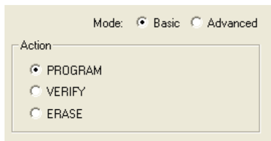
Figure 181 · Basic Mode
