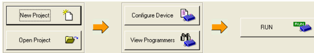
Figure 174 · Flow Window
