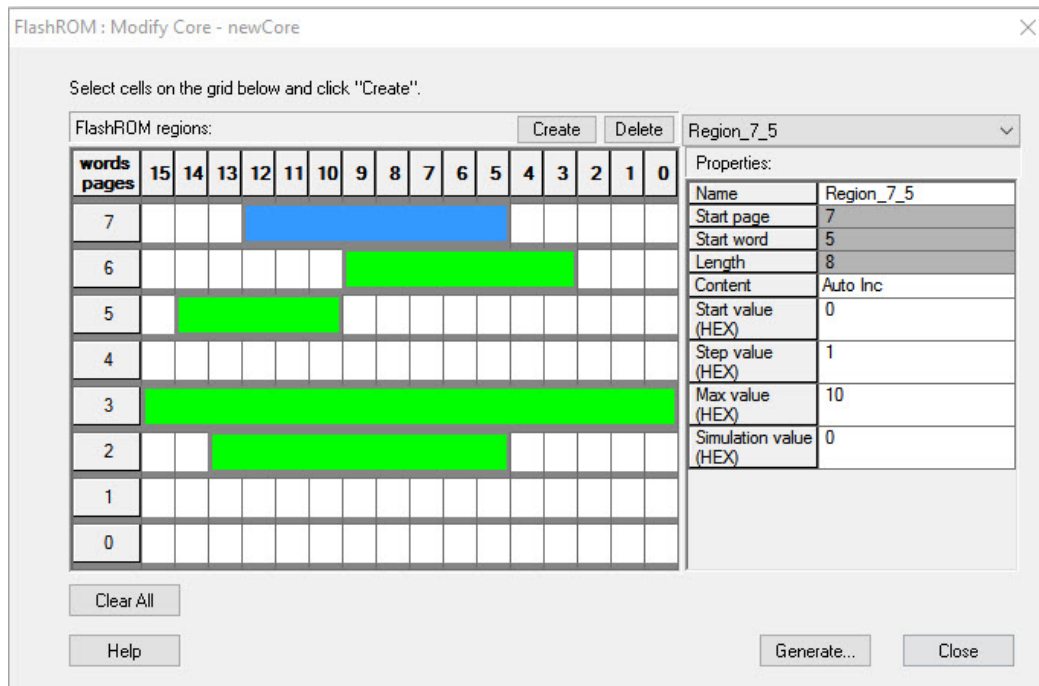
Figure 22 • FlashROM Settings
