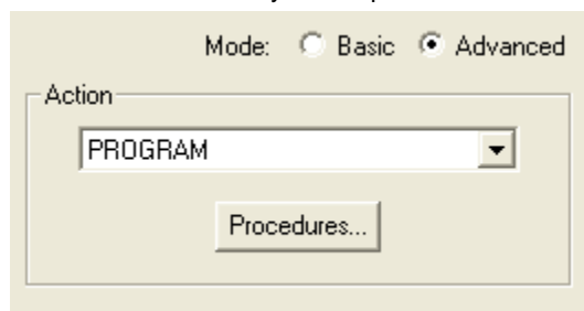
Figure 182 · Advanced Mode
