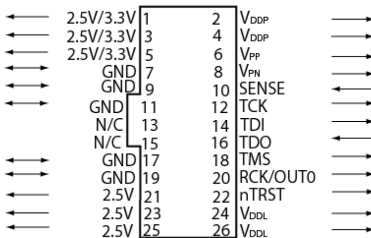
Figure 164 · 26-pin connections for FlashPro
