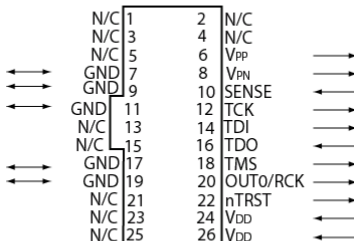
Figure 163 · 26-pin Connector for FlashPro Lite
