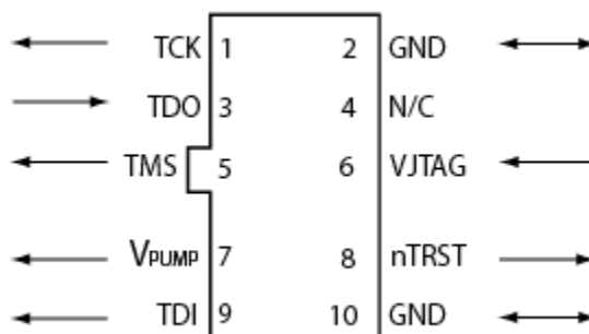
Figure 162 · FlashPro3 10-Pin Connector
