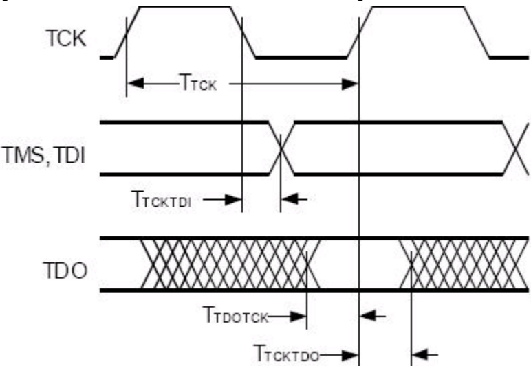
Figure 165 · JTAG Switching Characteristics
