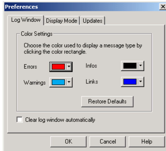
Figure 175 · Preferences
