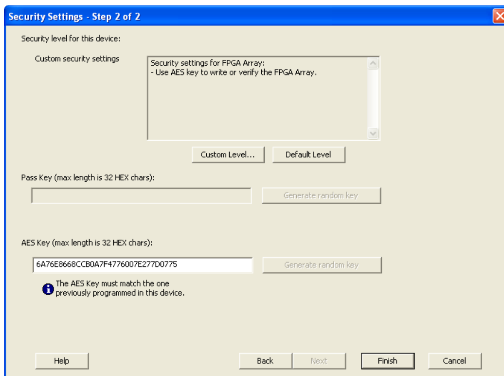
Figure 149 · Security Settings
