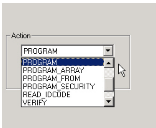
Figure 183 · Action Menu
