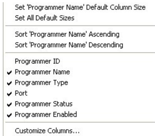
Figure 169 · Right-click Menu
