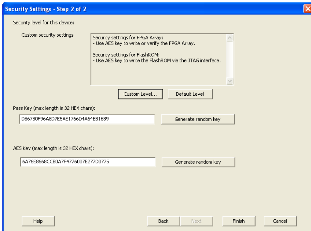
Figure 147 · Security Settings
