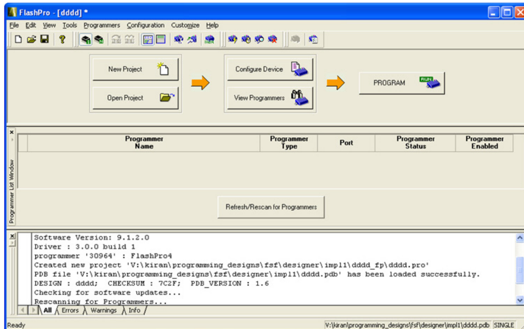
Figure 12 · FlashPro GUI
