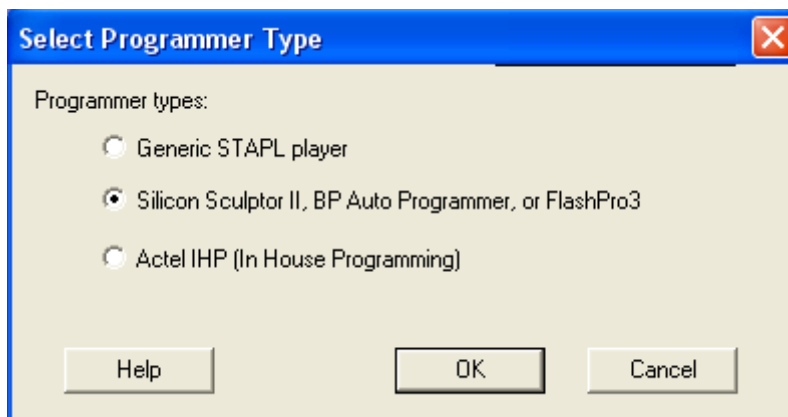
Figure 145 · Select Programmer
