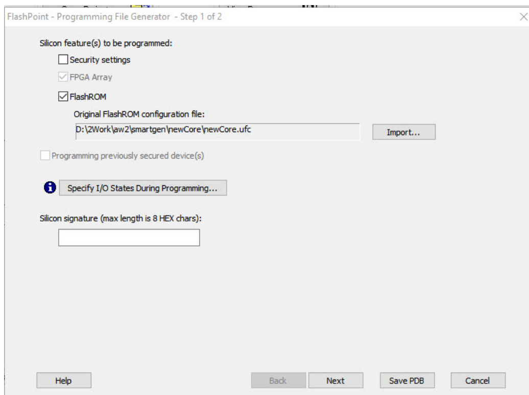
Figure 23 · FlashPoint
