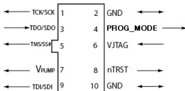
Figure 160 · FlashPro5 10-Pin Connector
