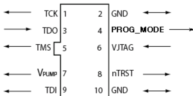
Figure 161 · FlashPro4 10-Pin Connector
