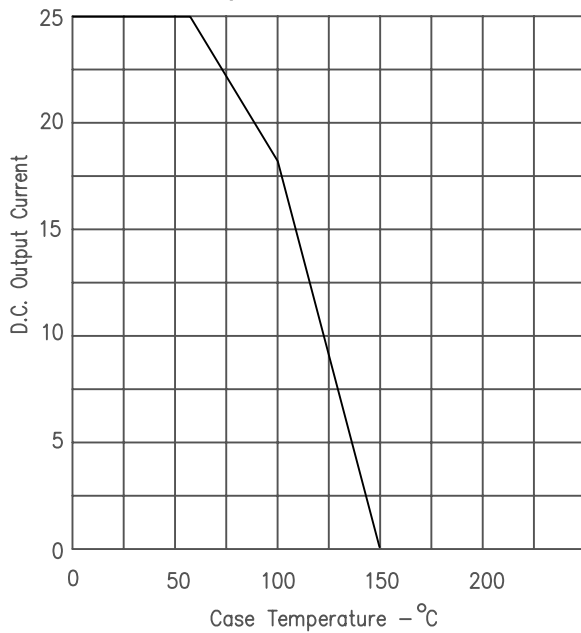
Figure 3 Current Derating
