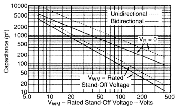
Figure 1 – Capacitance vs Stand-Off Voltage For 1500W TVSs
