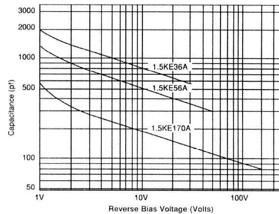
Figure 2 – Capacitance vs Reverse Bias Voltage
