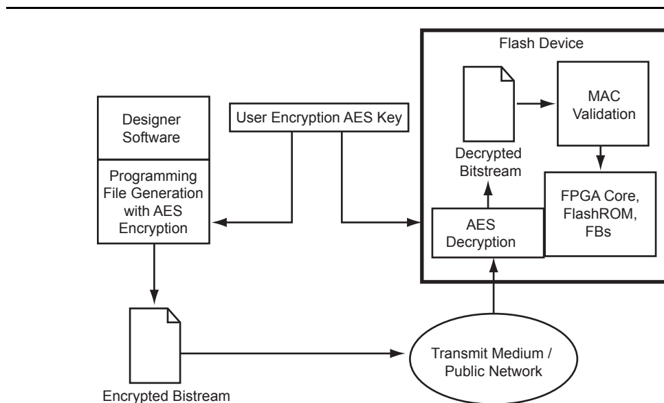
Figure 12-1 • AES-128 Security Features
