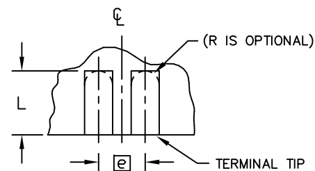
EVEN TERMINAL DETAIL 'A'
