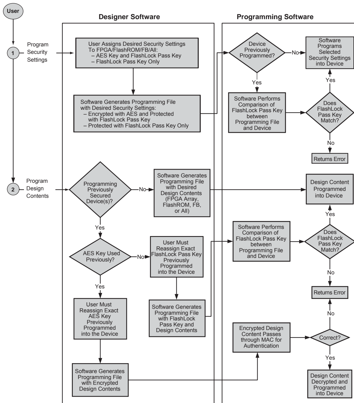
Figure 10-9 • Security Programming Flows
