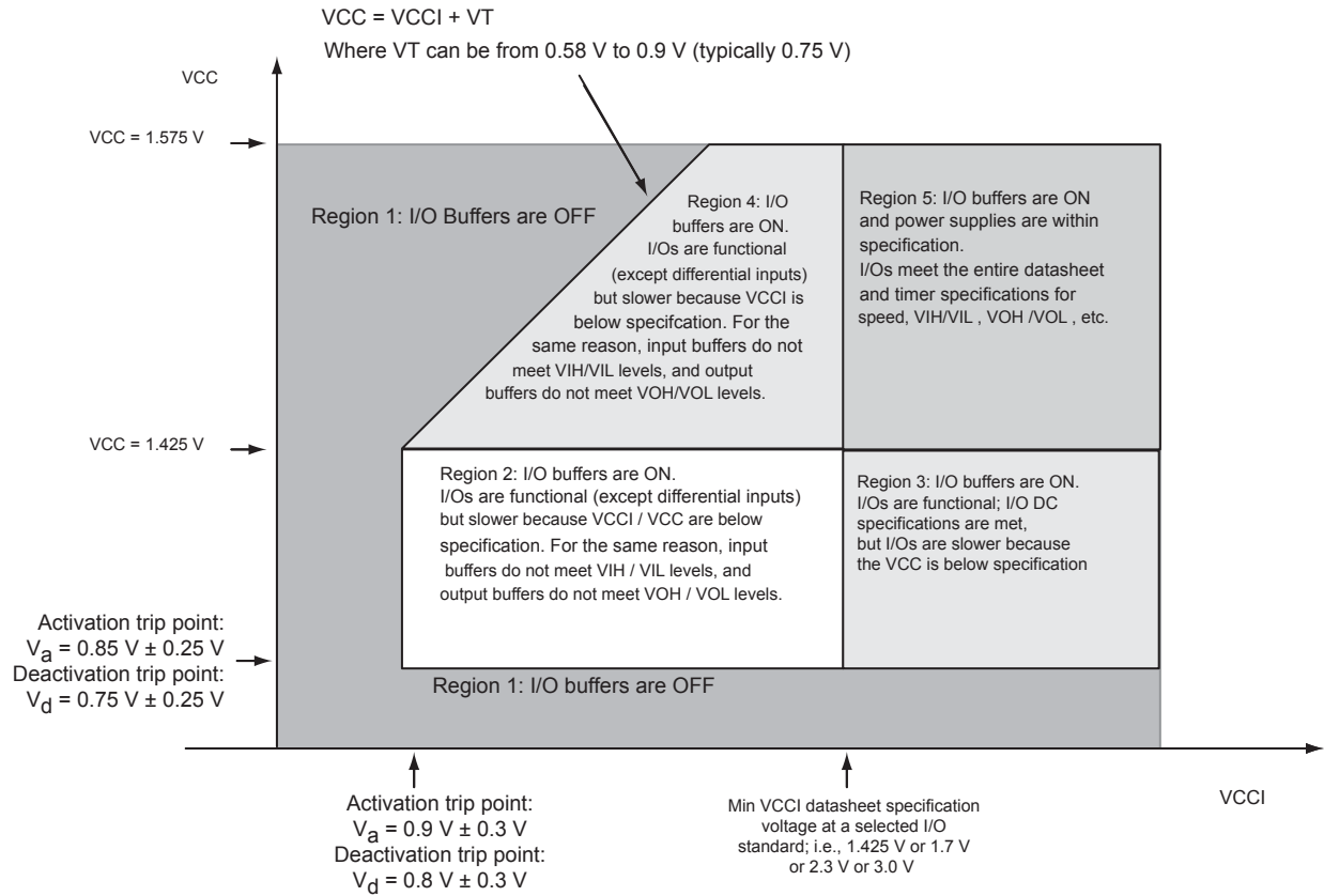
Figure 15-4 • I/O State as a Function of V_{CCI} and V_{CC} Voltage Levels for IGLOO V5, IGLOO nano V5, IGLOO PLUS V5, ProASIC3L, and ProASIC3 Devices Running at V_{CC} = 1.5 \text{ V} \pm 0.075 \text{ V}
