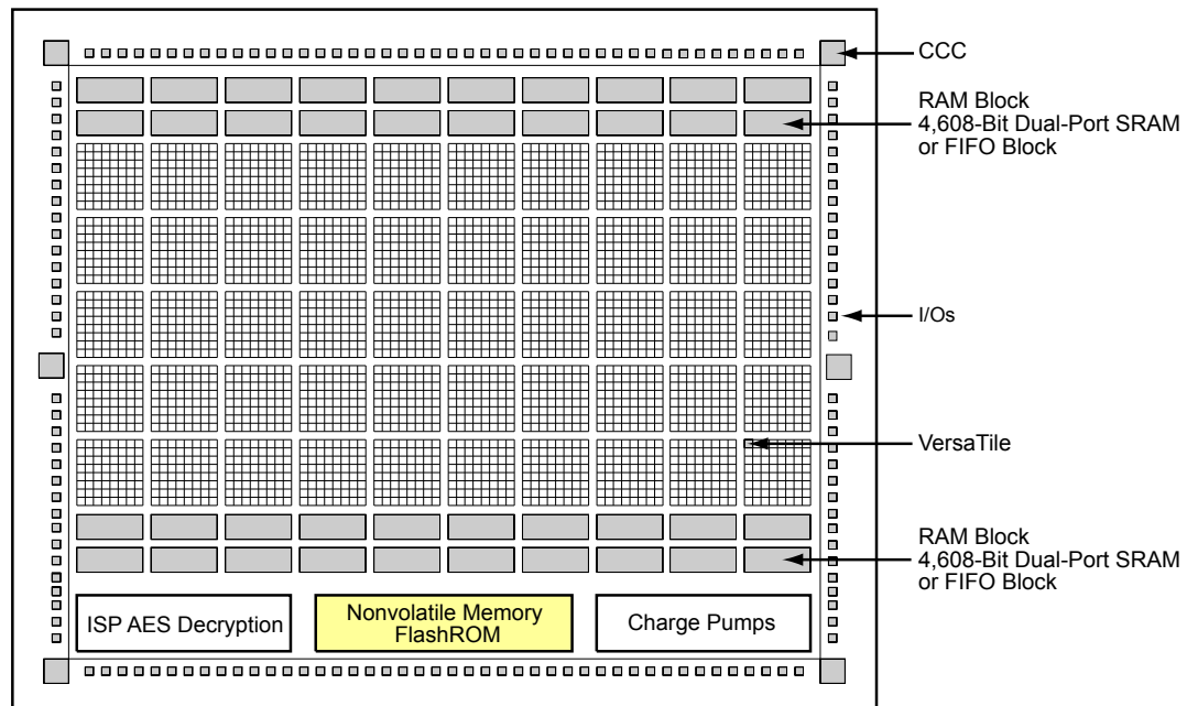
Figure 5-3 • ProASIC3 and IGL00 Device Architecture
