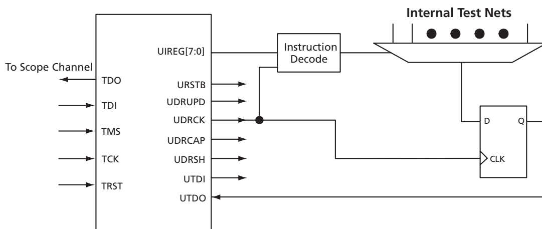
Figure 14-6 • UJTAG Usage Example in Test and Debug Applications
