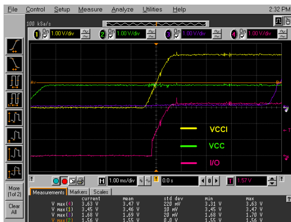
Figure 15-2 • I/O State when VCC Is Powered before VCCI
