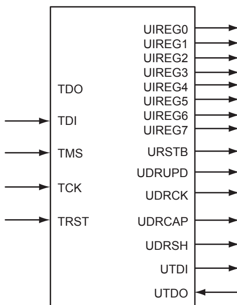
Figure 14-2 • UJTAG Tile Block Symbol
