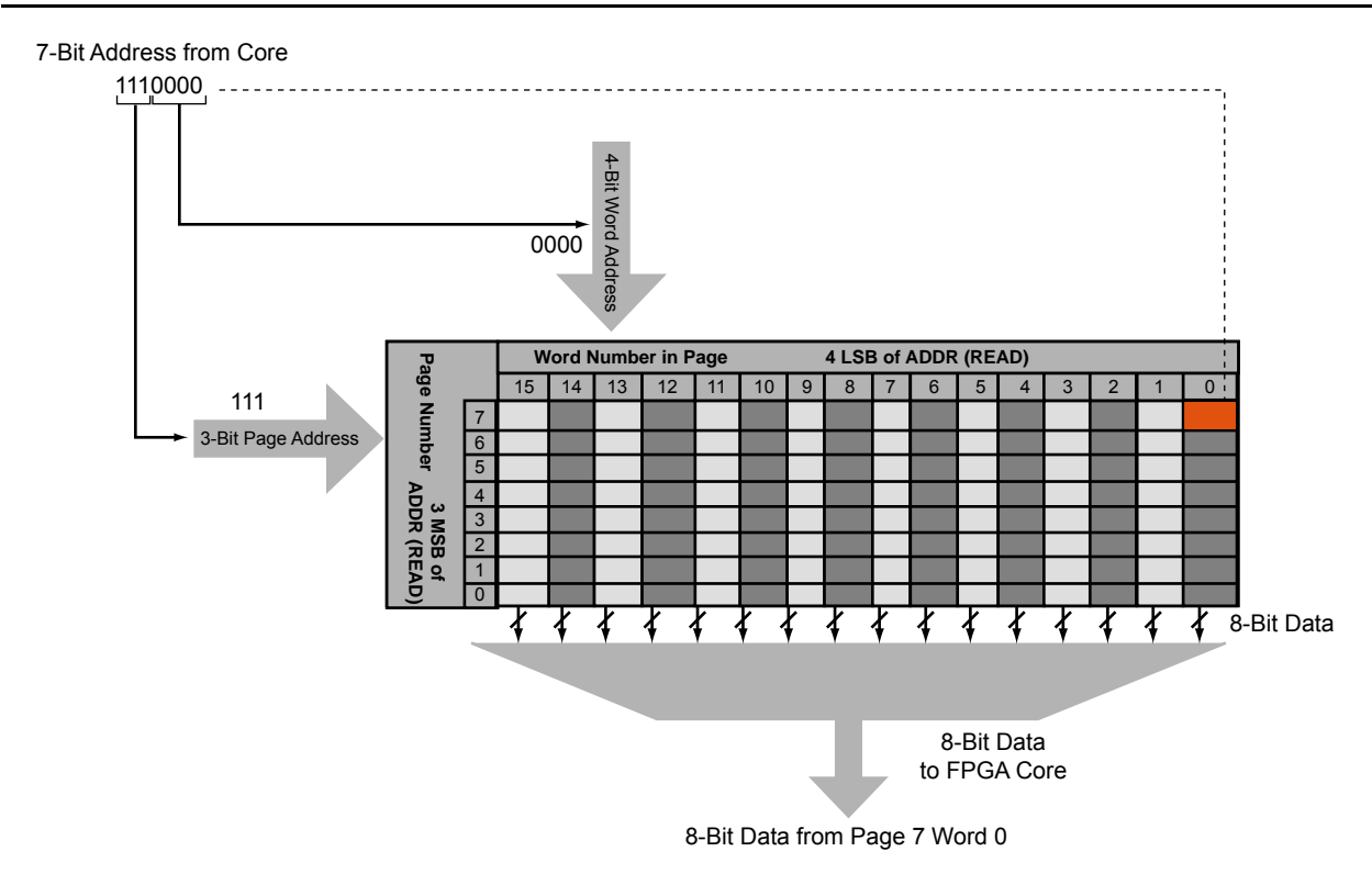
Figure 5-7 • Accessing FlashROM Using FPGA Core
