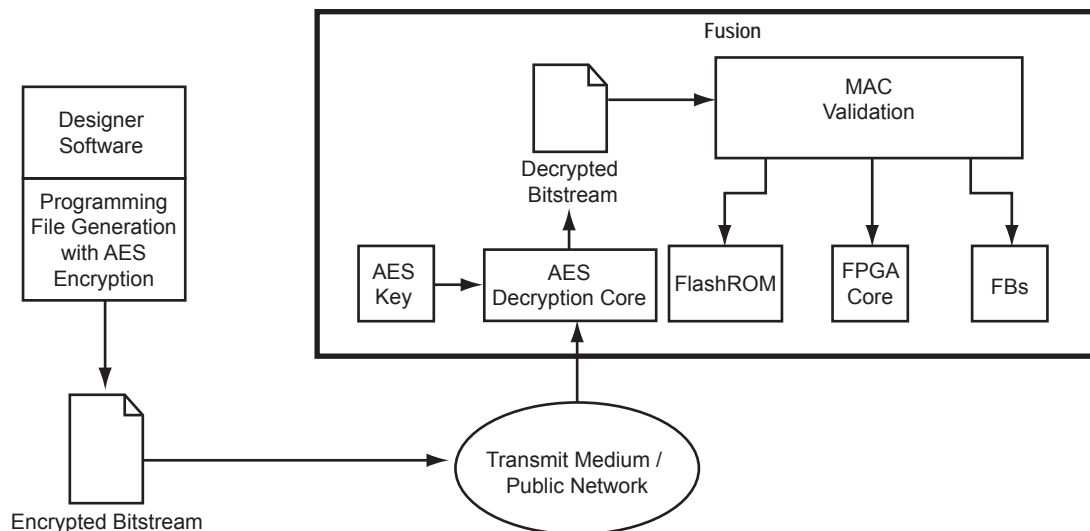
Figure 10-5 • Example Application Scenario Using AES in Fusion Devices
