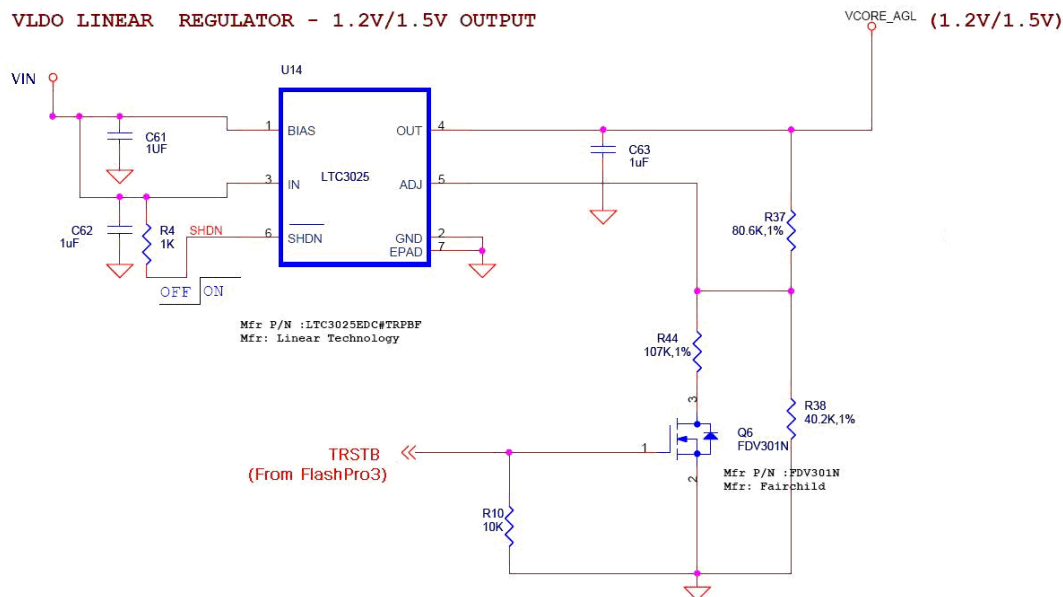
Figure 12-1 • Circuit Diagram
