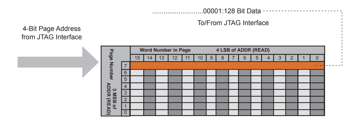
Figure 5-8 • Accessing FlashROM Using JTAG Port
