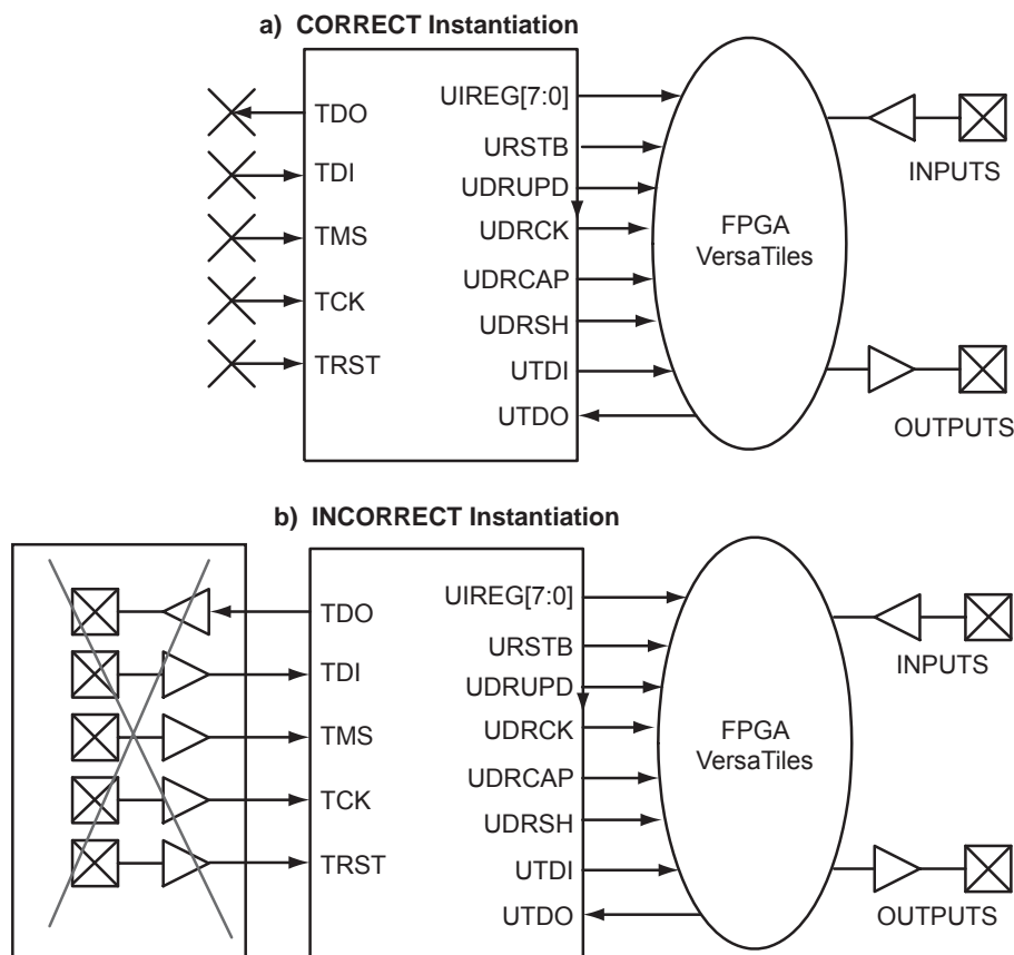
Figure 14-3 • Connectivity Method of UJTAG Macro
