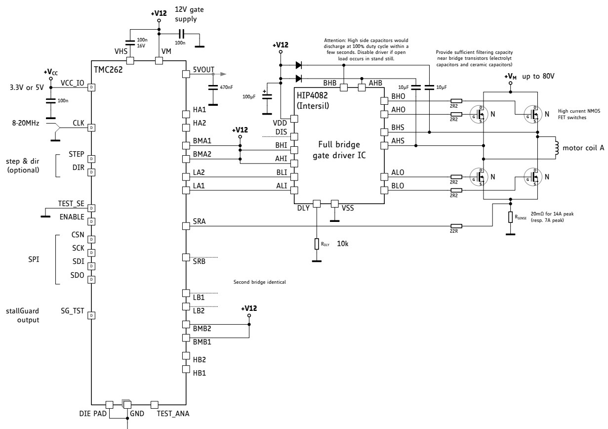
Figure 14.1 High-current, high-voltage power stage using external gate drivers (minimum part count)
