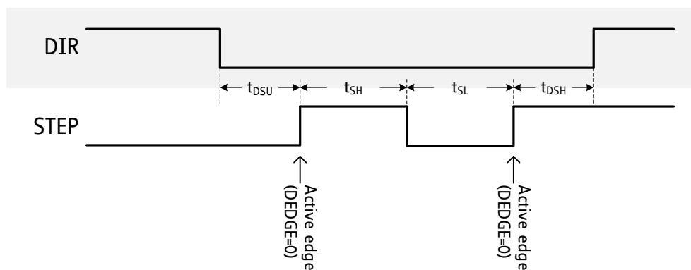
Figure 7.1 STEP/DIR timing
