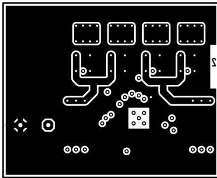
Figure 15.1 Layout example
