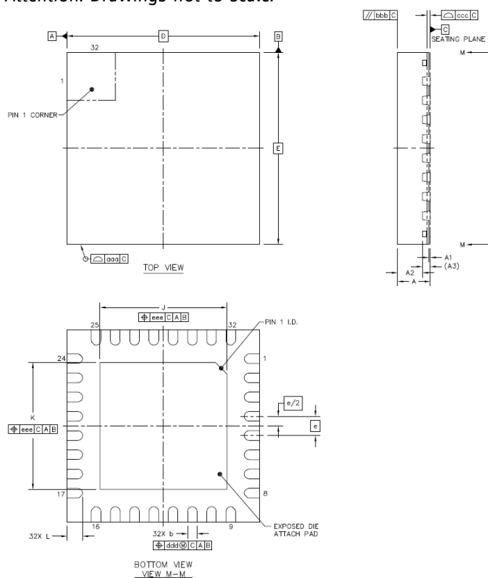
Figure 18.1 Dimensional drawings
