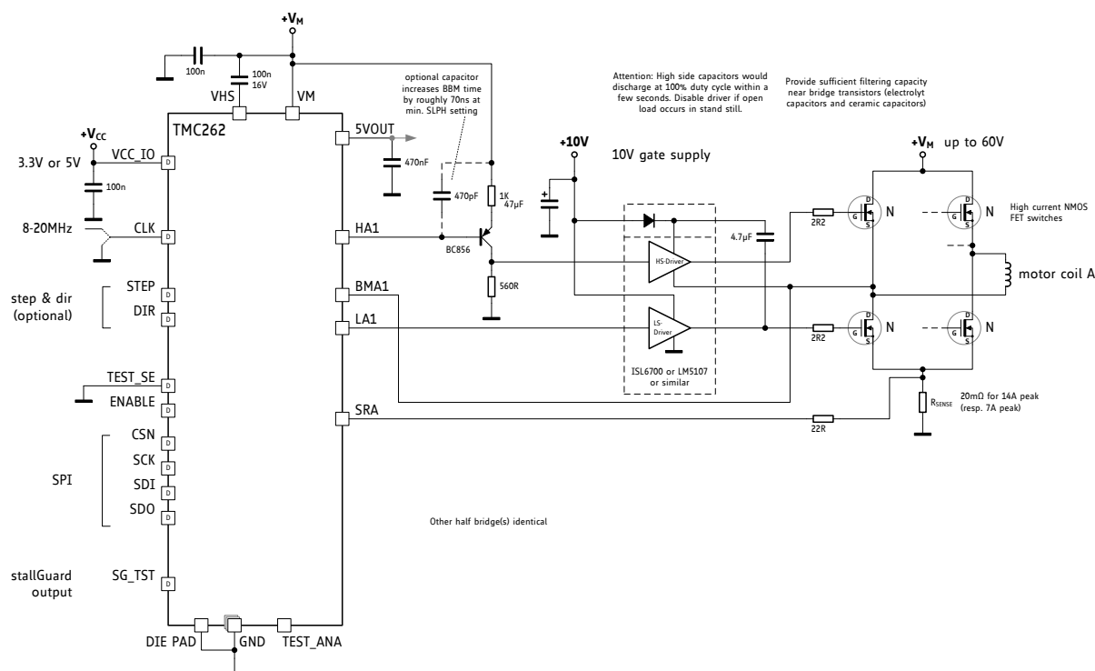
Figure 14.2 High-current power stage using external gate drivers with short to GND protection
