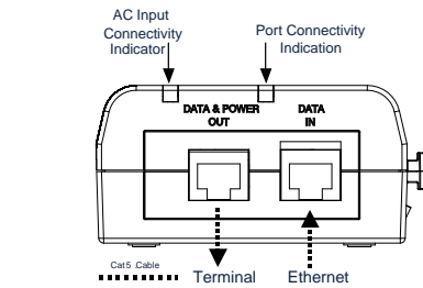
Figure 3: Connecting the PoE Midspan Indicators
