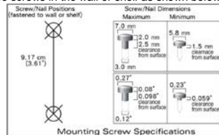
Figure 1: Mounting Instructions
