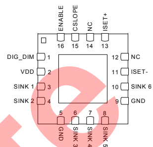
LQ PACKAGE (Top View)
