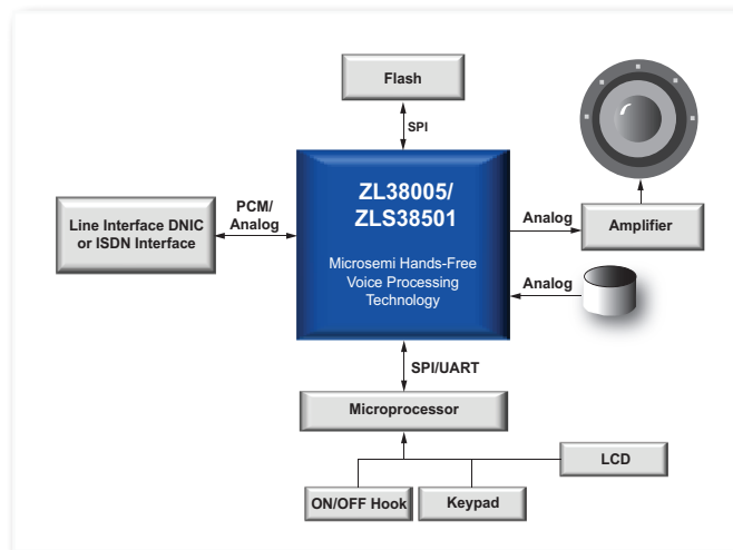
Figure 1: Speakerphone Application
